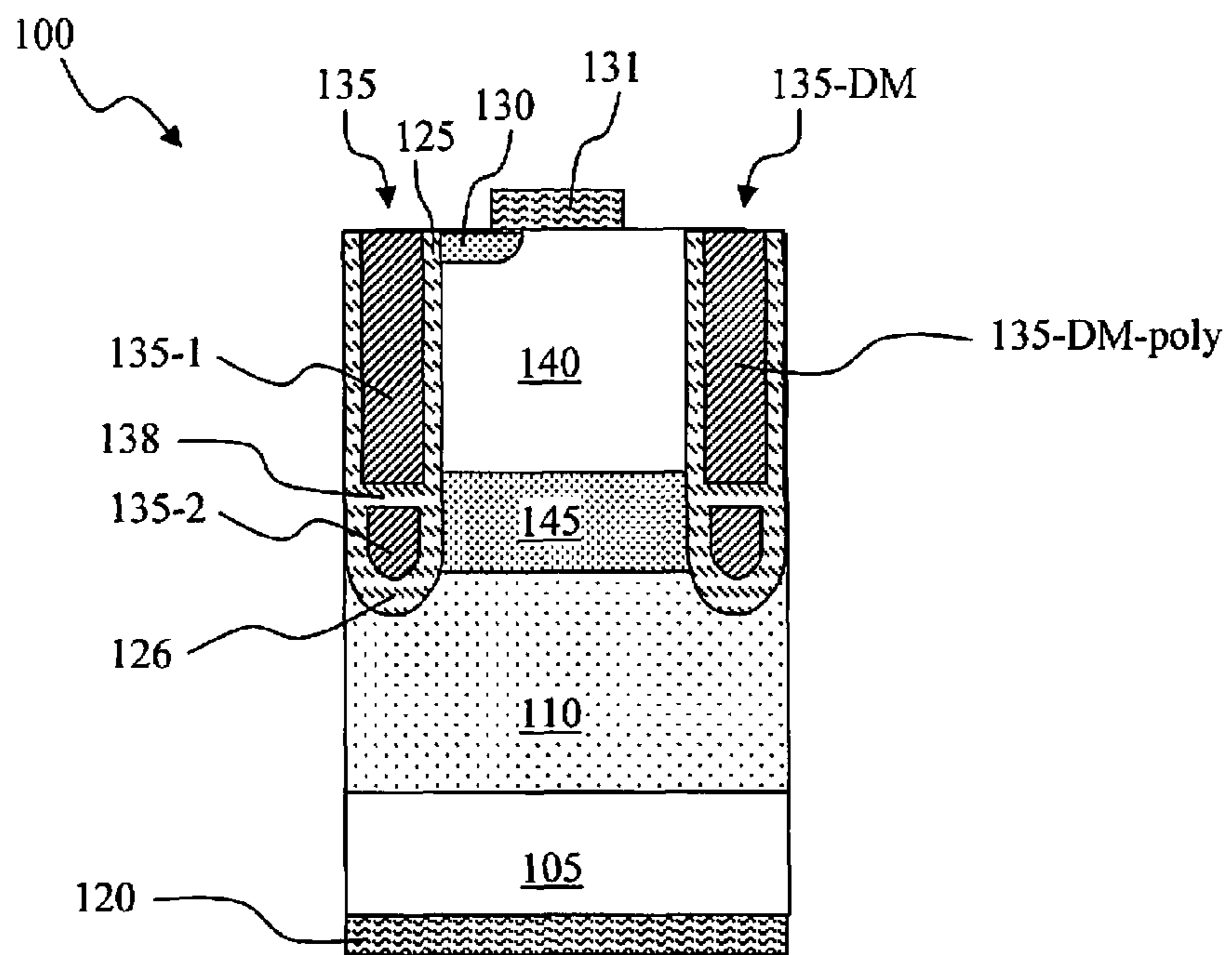
Fig. 2 Present Invention
