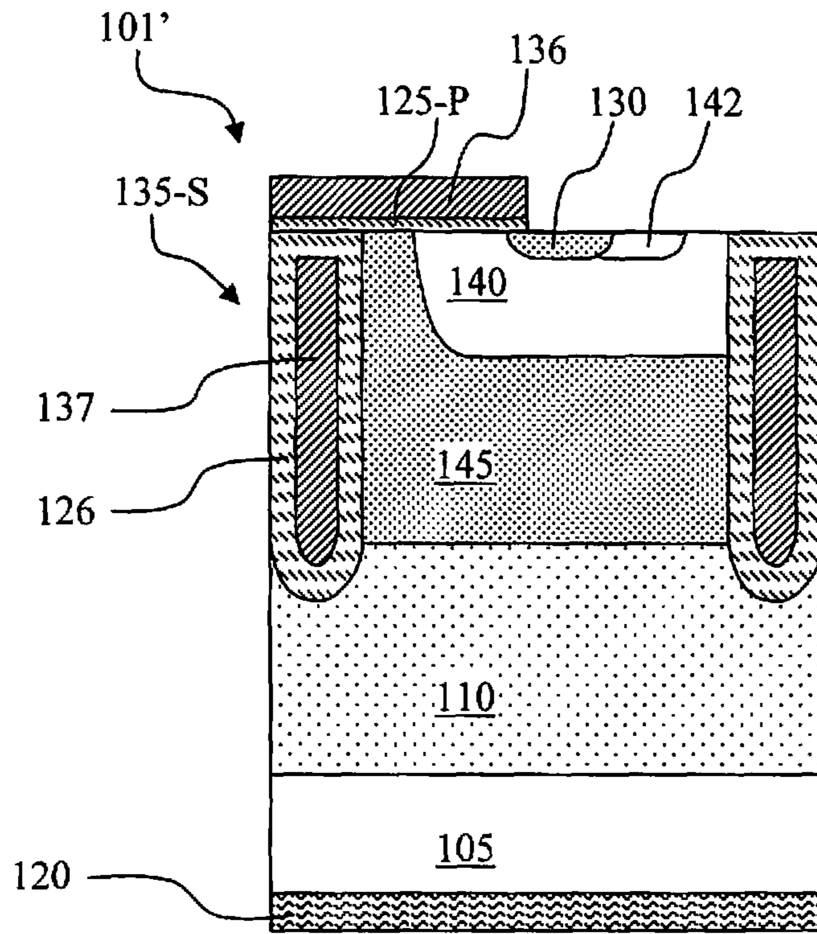
Fig. 5 Present Invention
