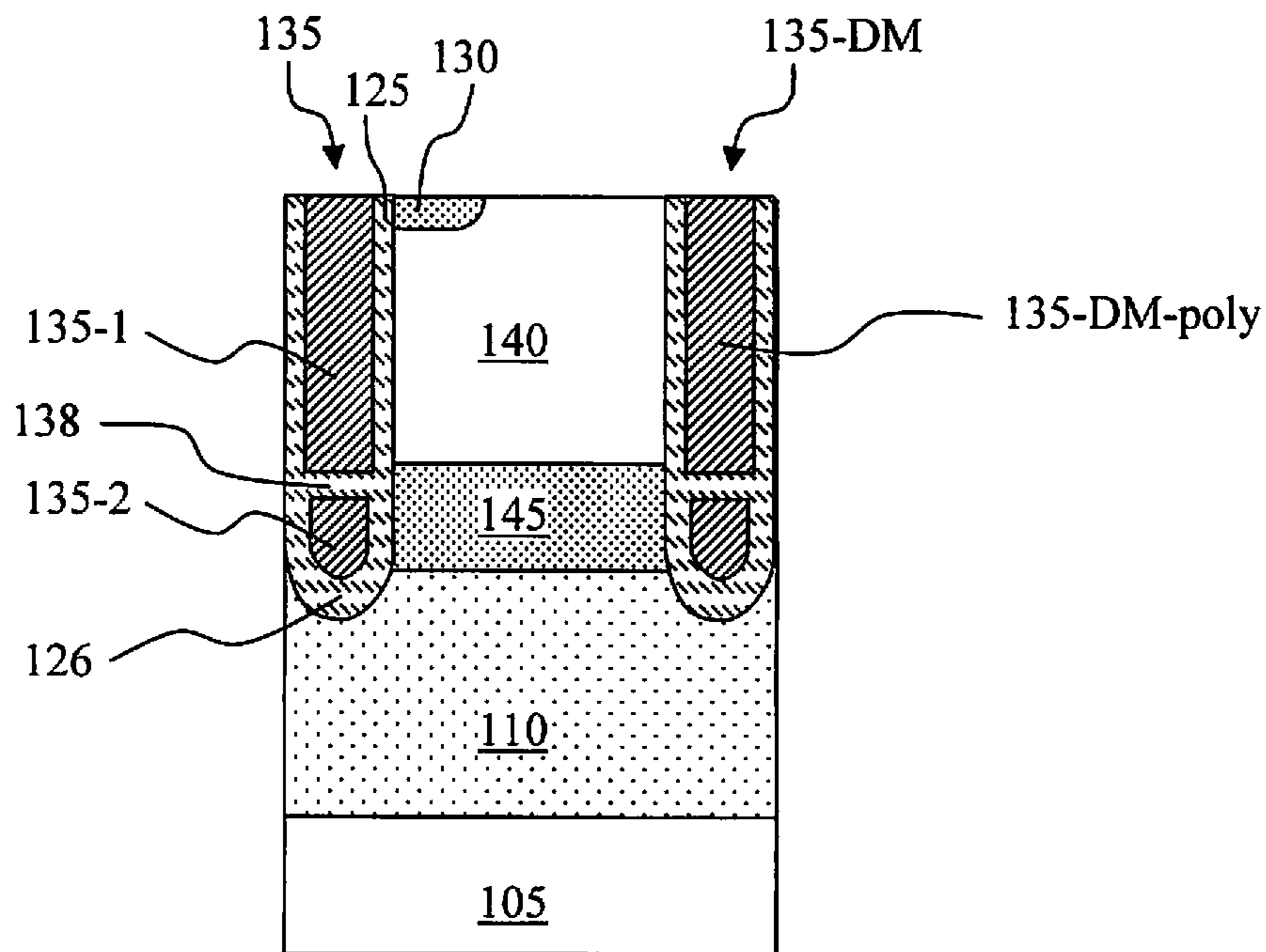
Fig. 8I Present Invention
