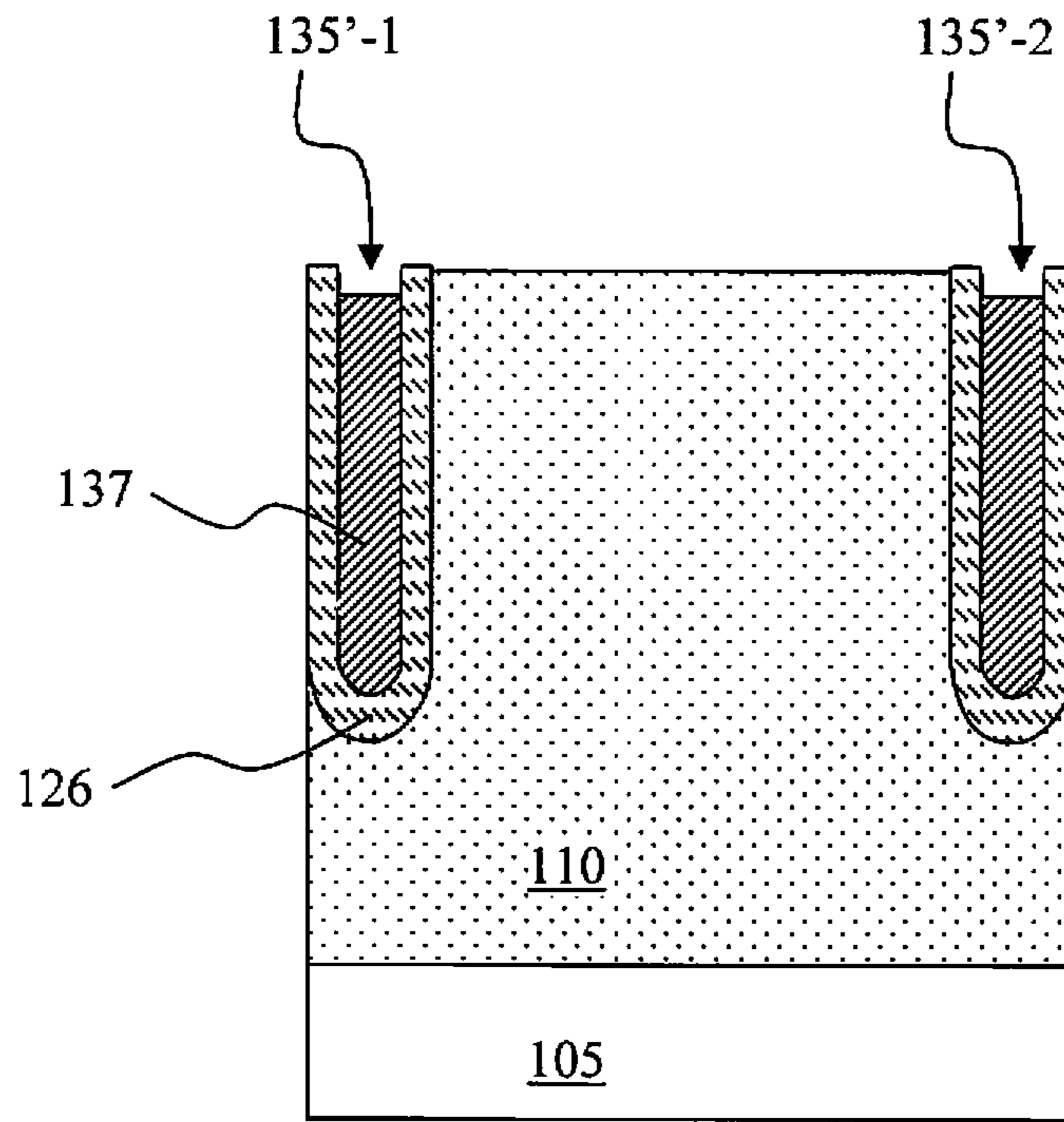
Fig. 15C Present Invention
