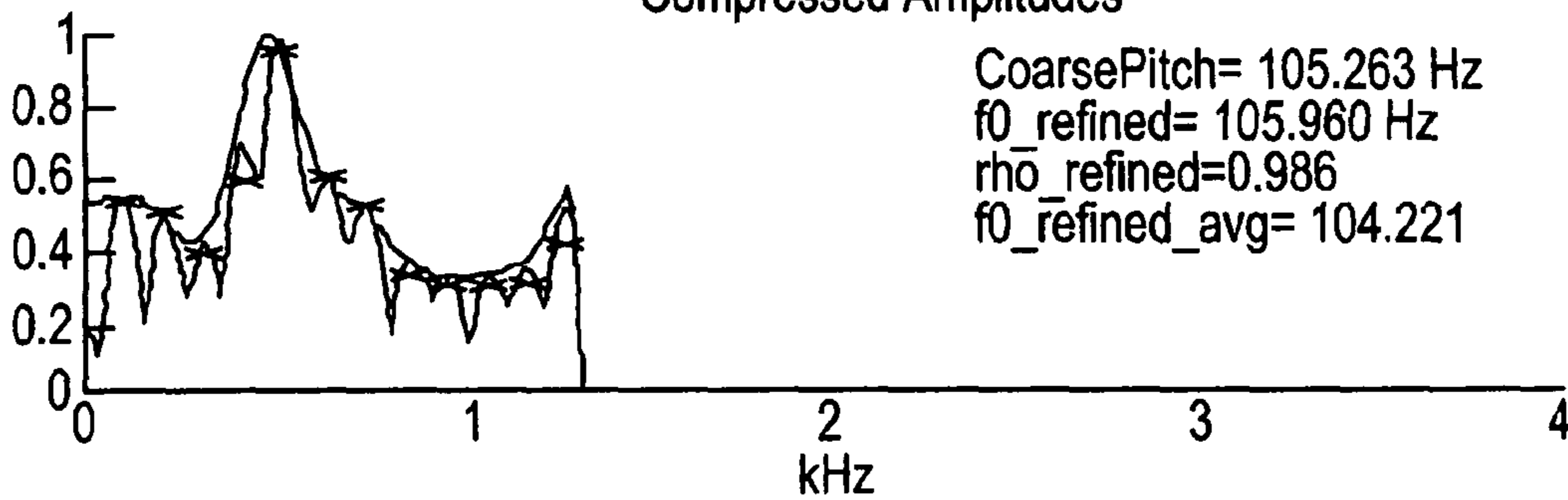
Compressed Amplitudes
