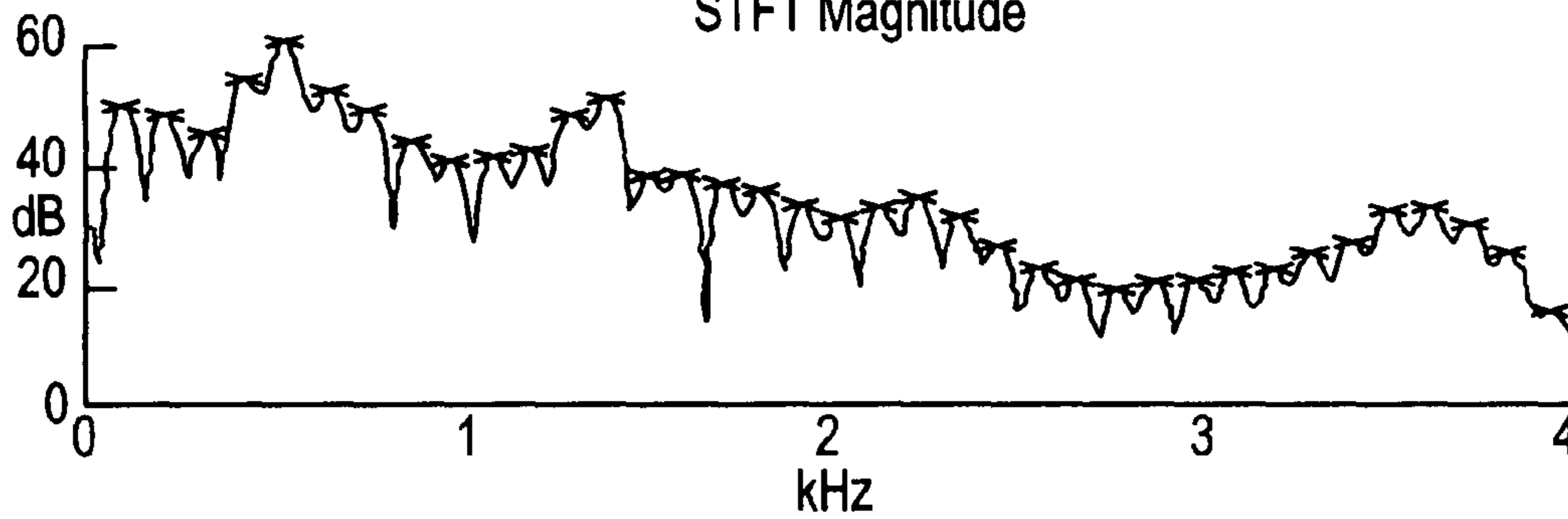
Compressed Amplitudes
