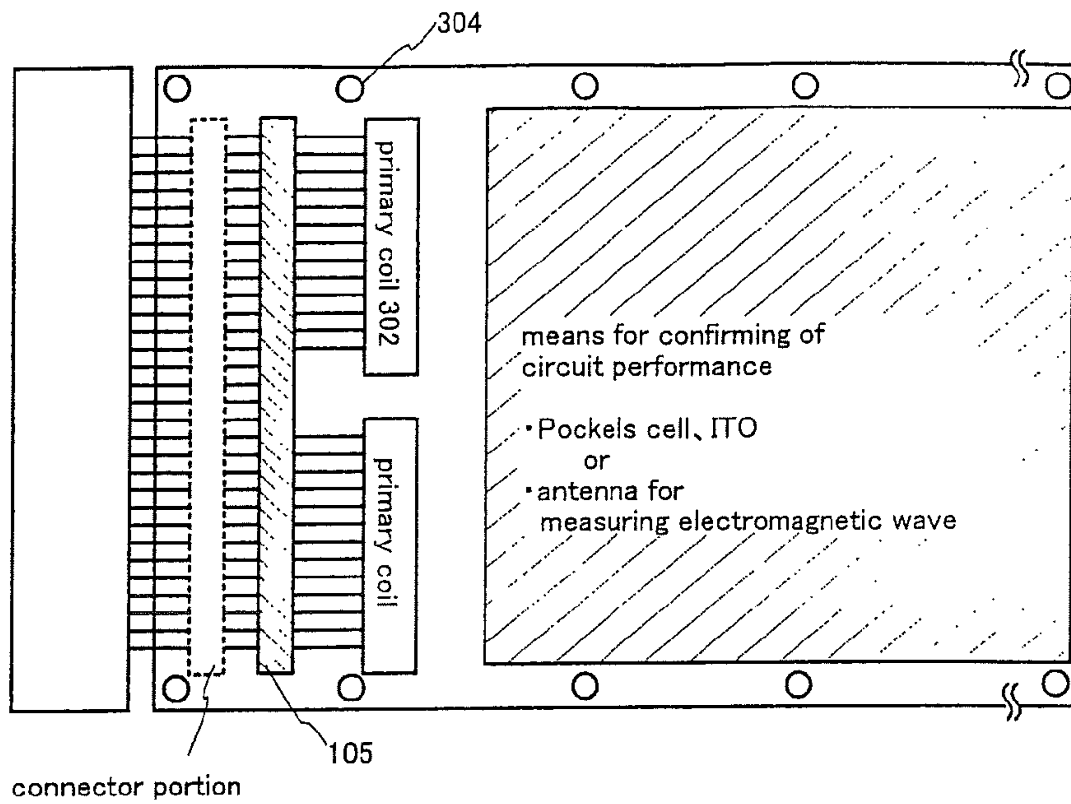
FIG. 4A check substrate
