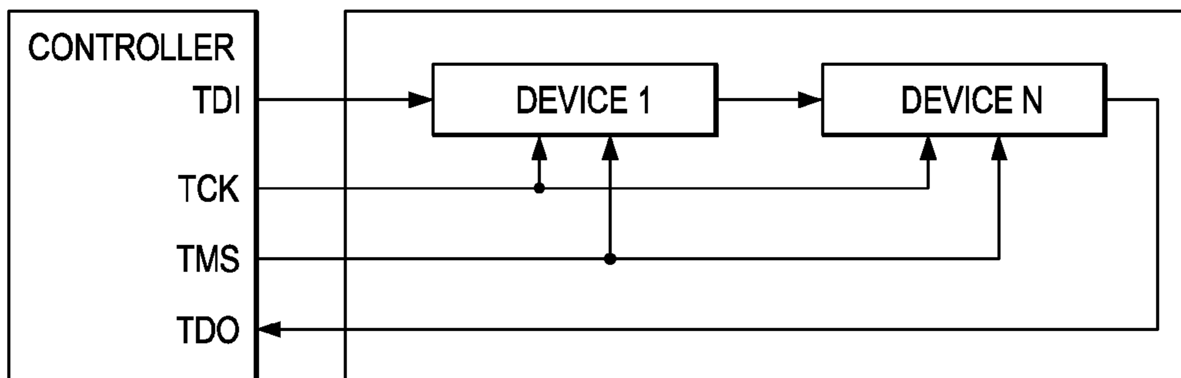
FIG. 6 (PRIOR ART)
