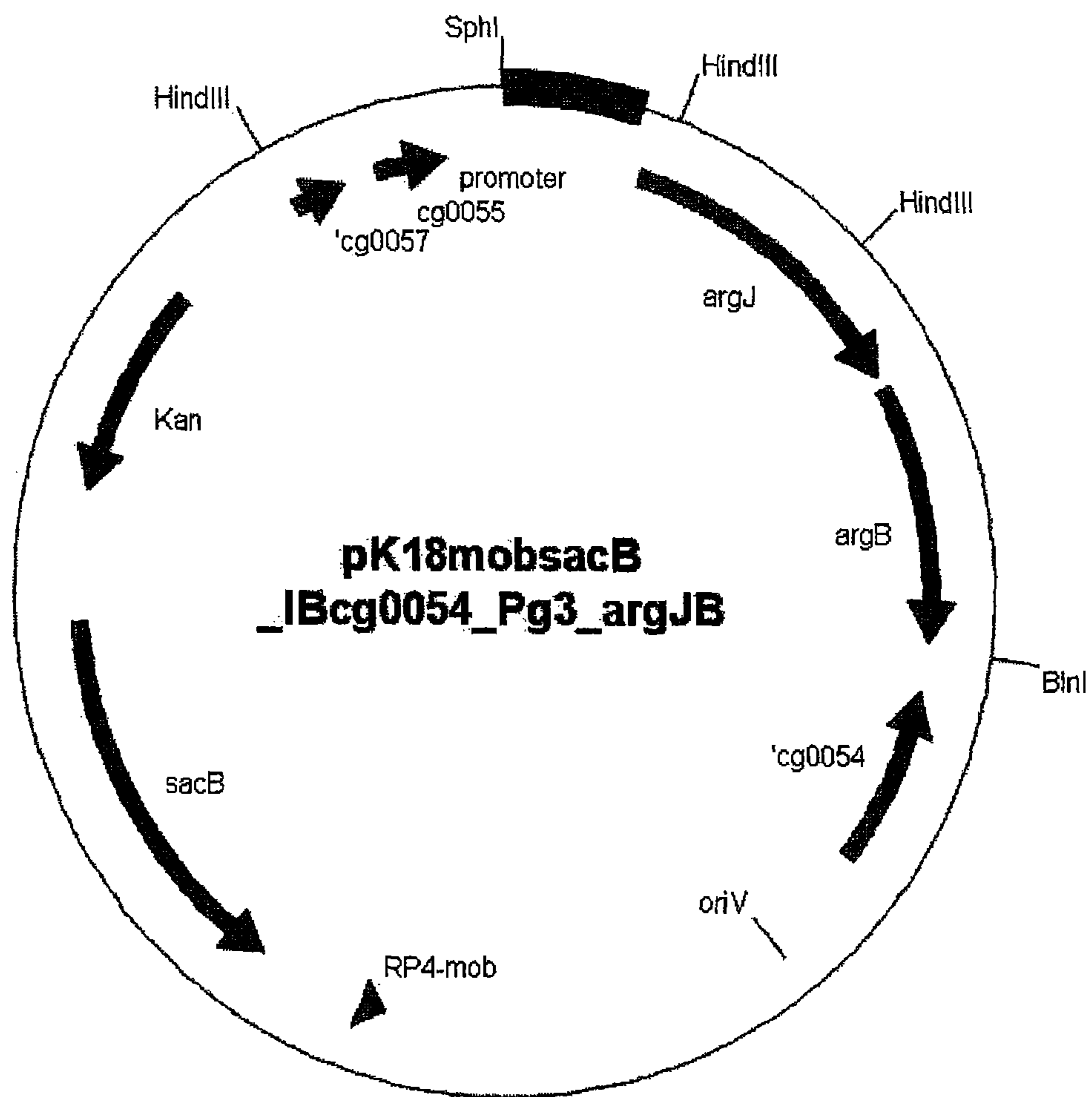
Figure 2: Plasmid pK18mobsacB_IBcg0054_Pg3_argJB
