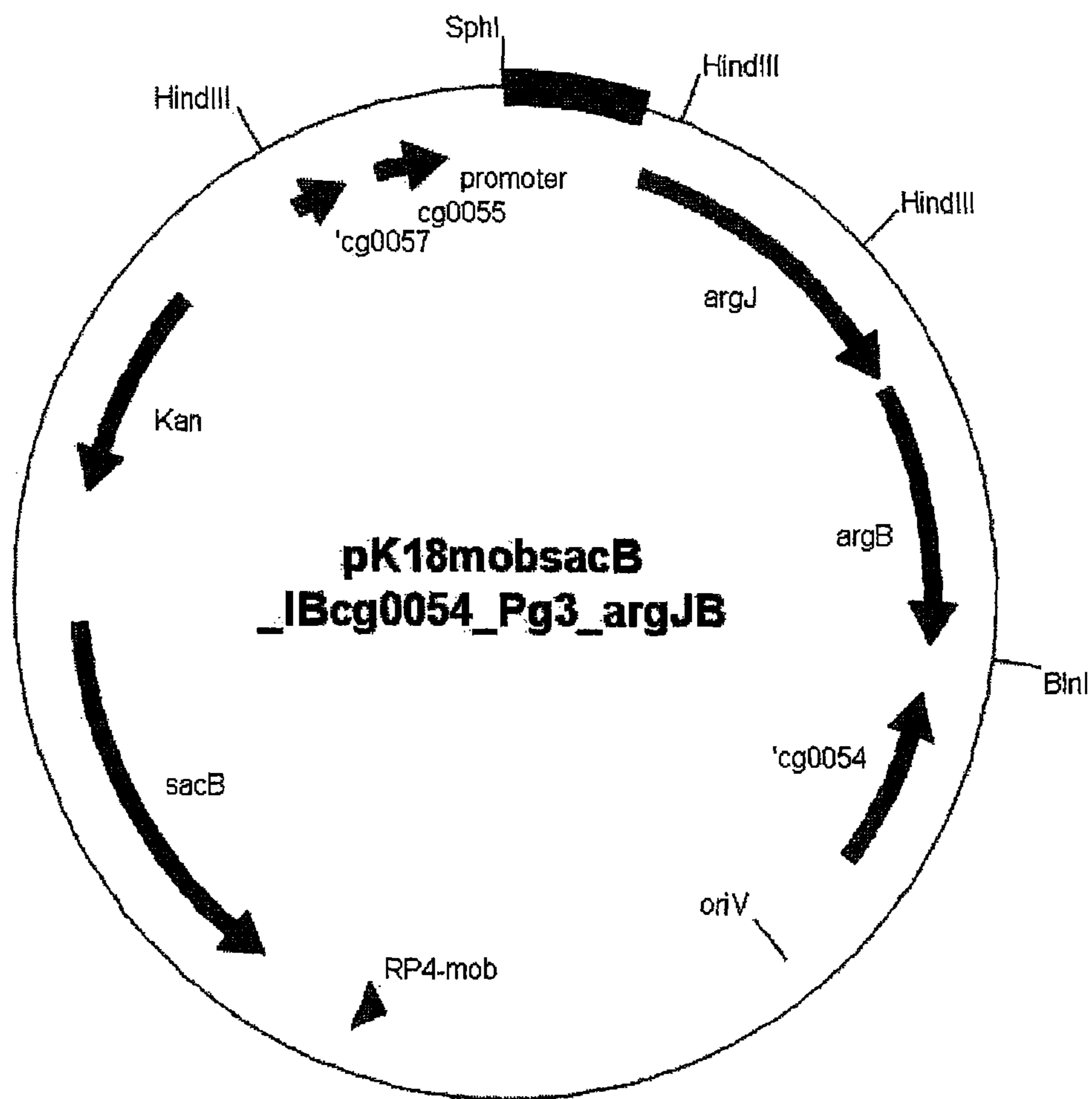
Figure 2: Plasmid pK18mobsacB_IBcg0054_Pg3_argJB
