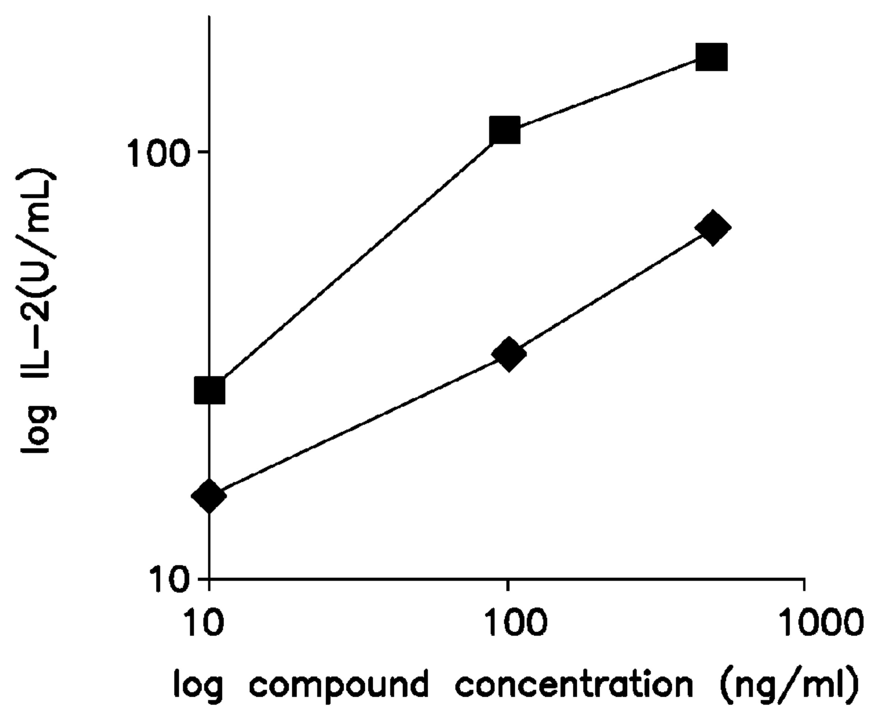
NKT cell stimulatory activity biotin-appended 6-amino-6-deoxygalactosylceramide 13. 1-◆ ; 14-■.
