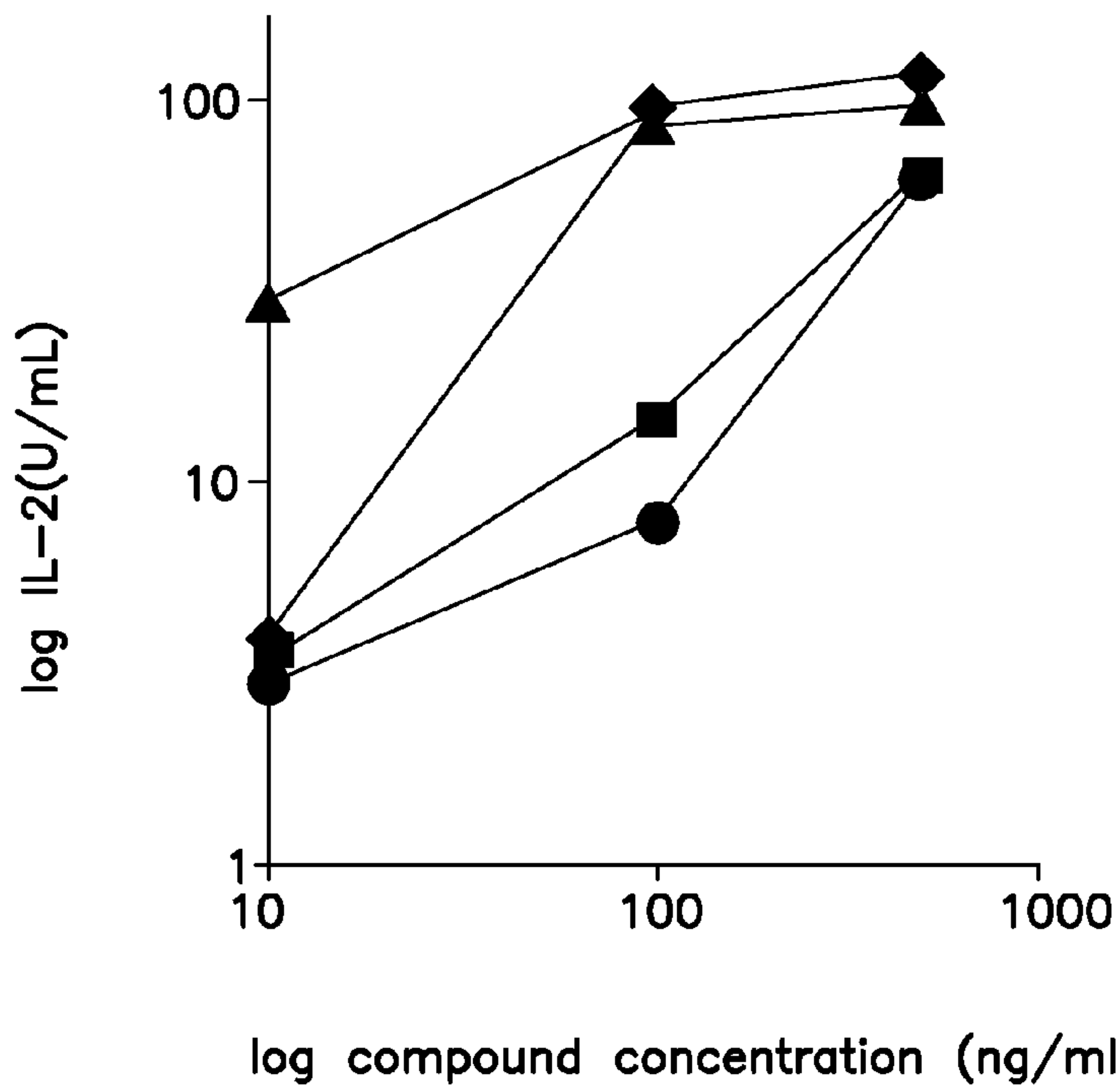
NKT cell stimulatory activity of fluorophore-appended 6-amino-6-deoxygalactosylceramides 8, 10, 12. 1-◆ ;8-● ;10-▲ ;12-■.
