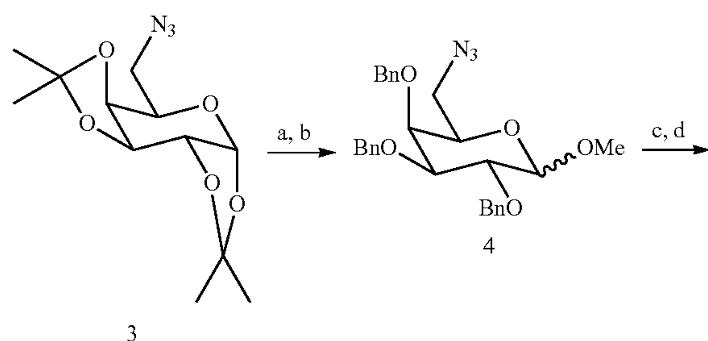
SCHEME 1
