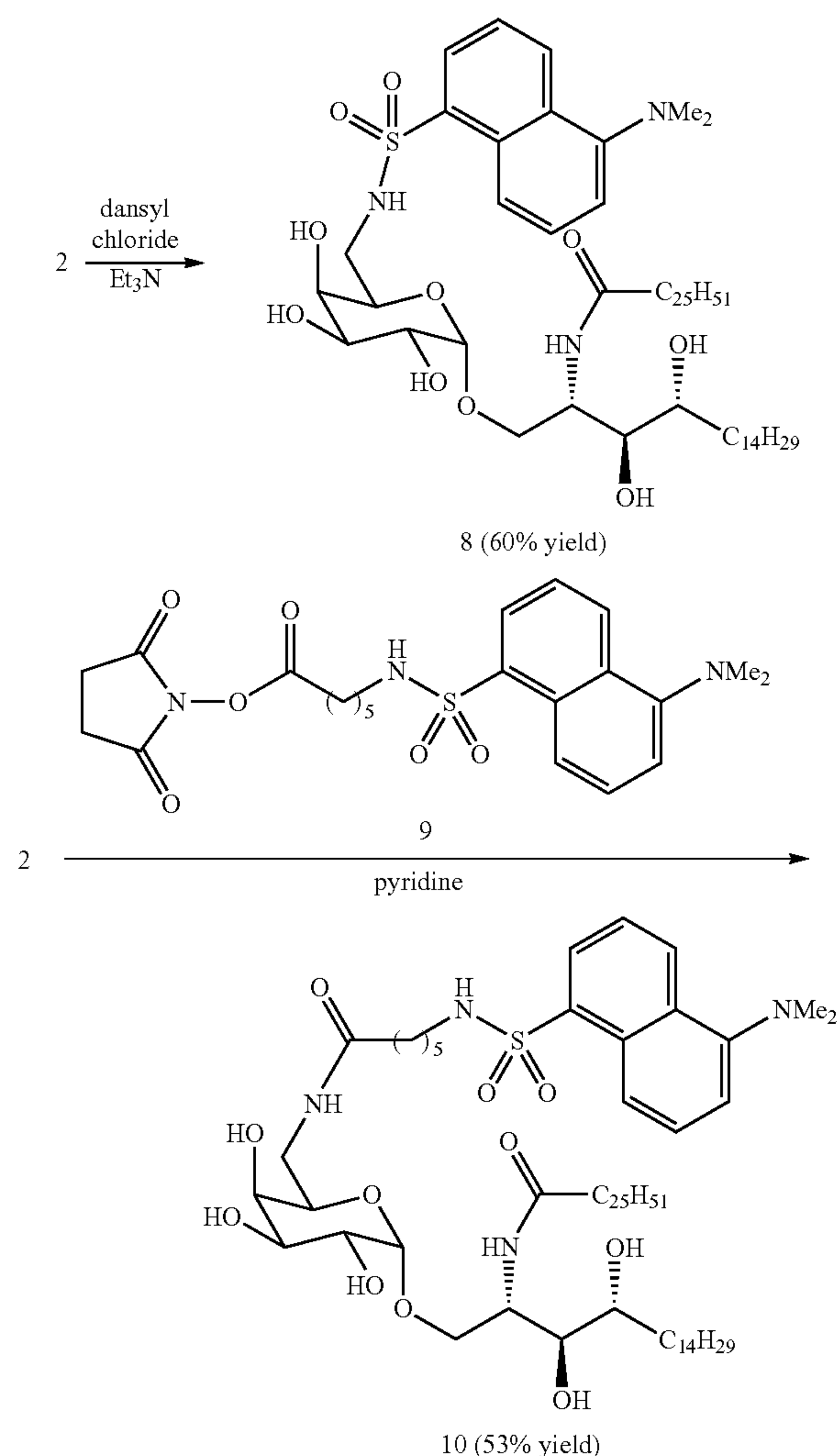
SCHEME 2
