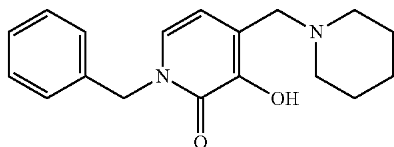
1-Benzyl-3-hydroxy-4-(piperidin-1-ylmethyl)pyridin-2(1H)-one
