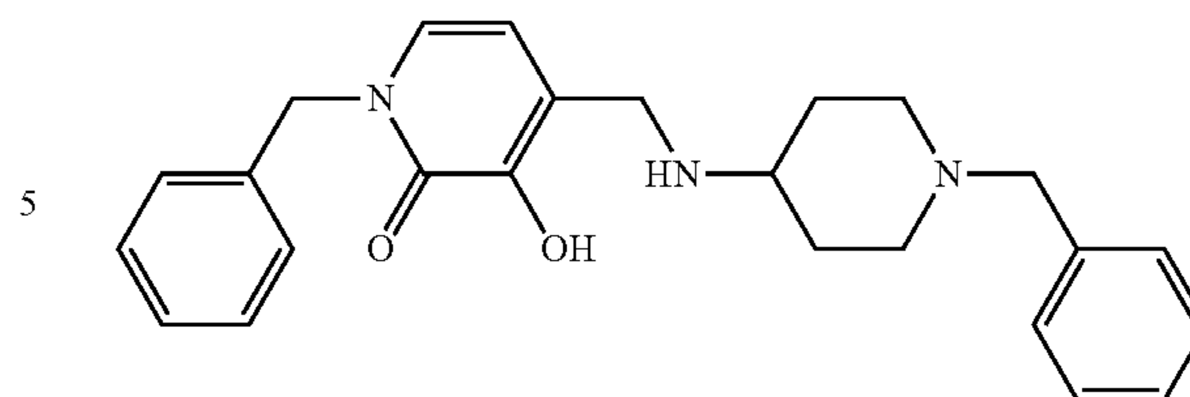
1-Benzyl-3-hydroxy-4-[(1-benzylpiperidin-4-yl)amino]methyl]pyridin-2(1H)-one
