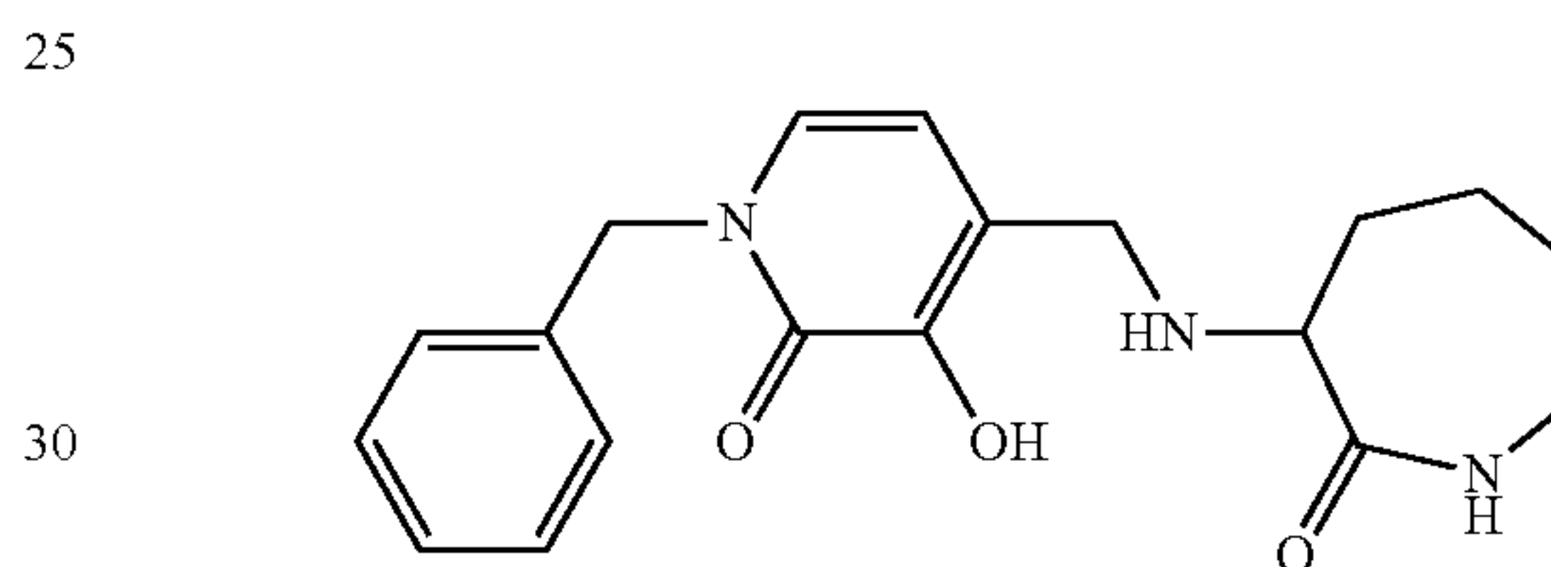
3-[(1-Benzyl-3-hydroxy-2-oxo-1,2-dihydropyridin-4-yl)methylamino]azepan-2-one
