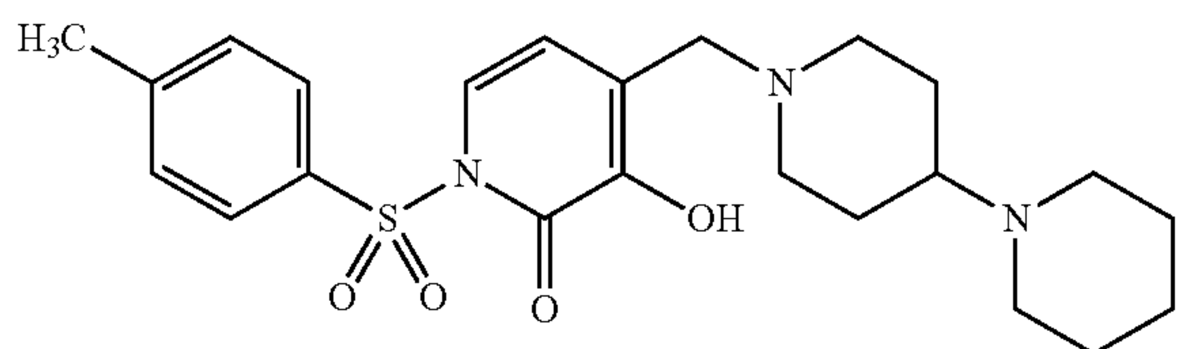
1-(4'-Methylbenzenesulfonyl)-3-hydroxy-4-[1,4'] Bipiperidiny-1'-ylmethylpyridin-2(1H)-one
