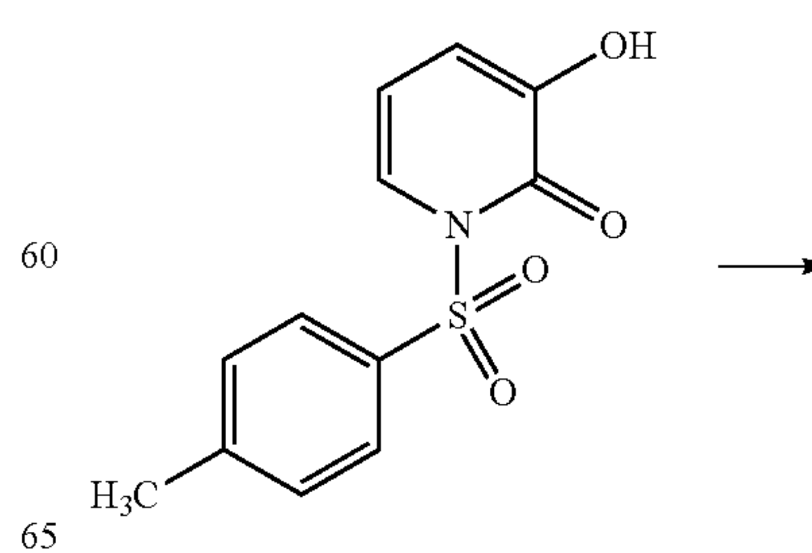
Scheme IV
