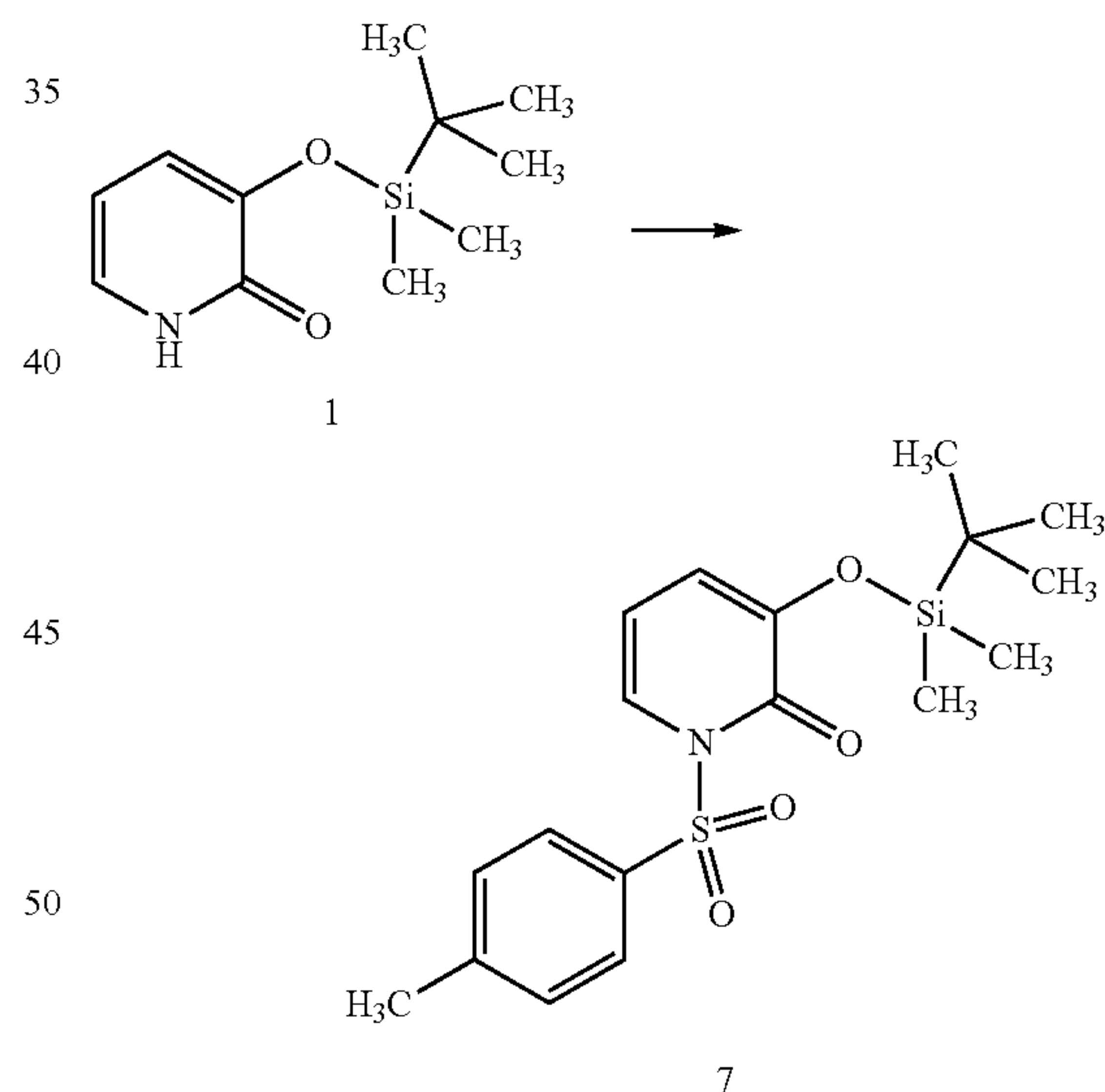
Scheme III
