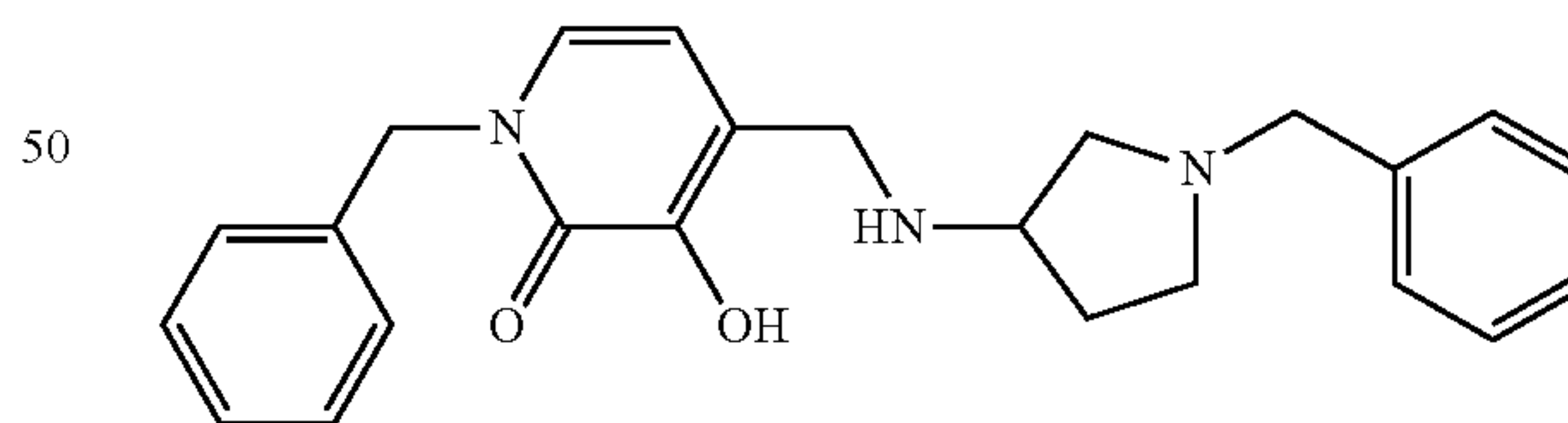
1-Benzyl-3-hydroxy-4-[(1-benzylpyrrolidin-3-yl)amino]methyl]pyridin-2(1H)-one
