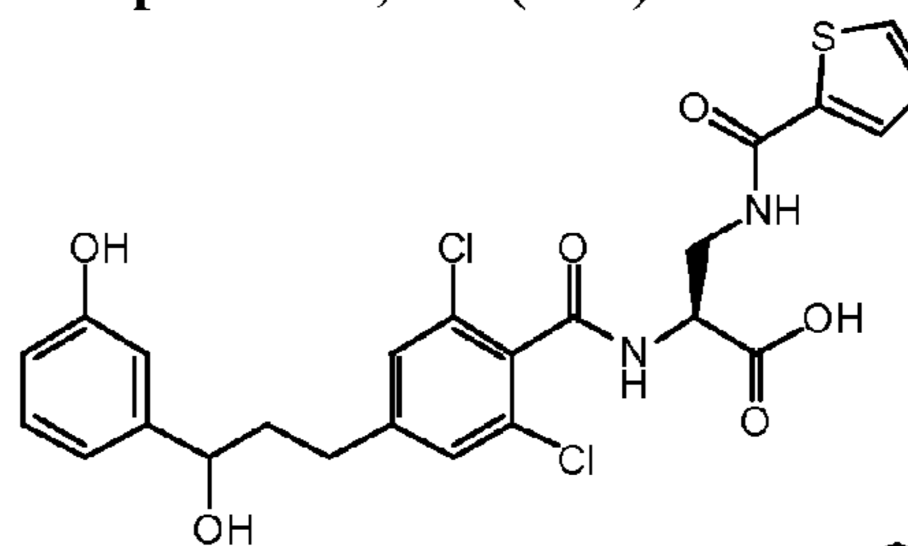
Compound 4
