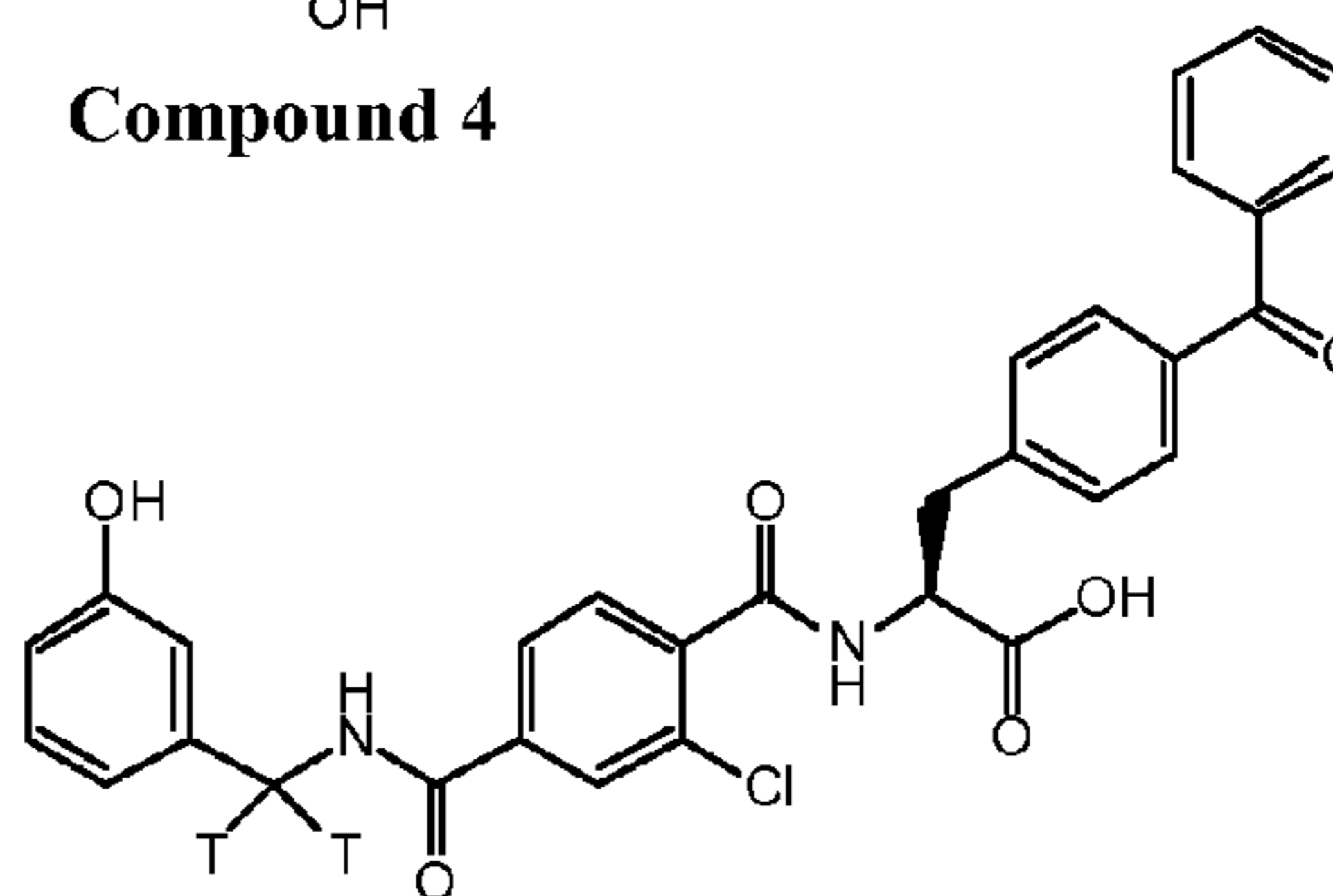
Compound 5
