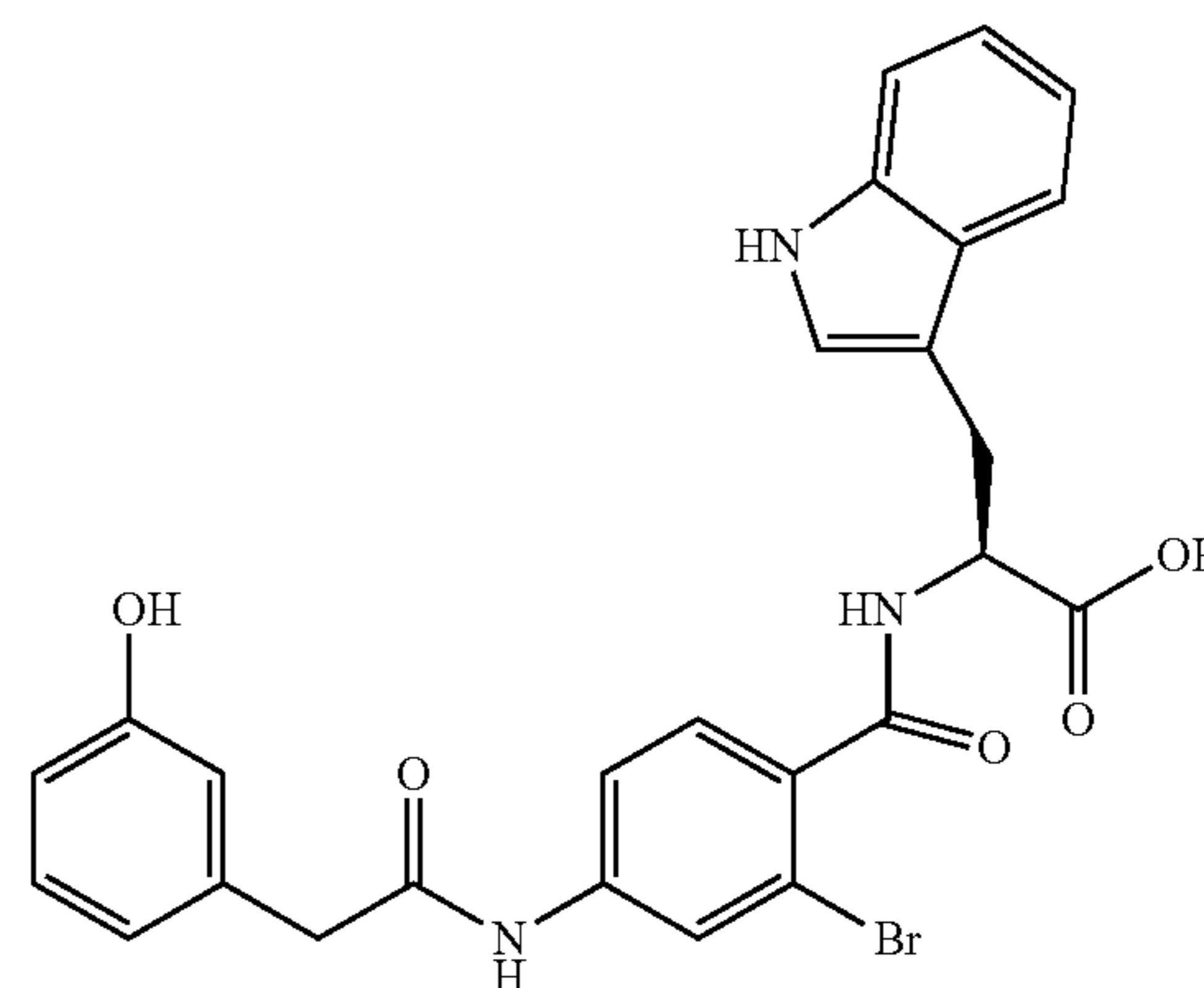
Compound 7
