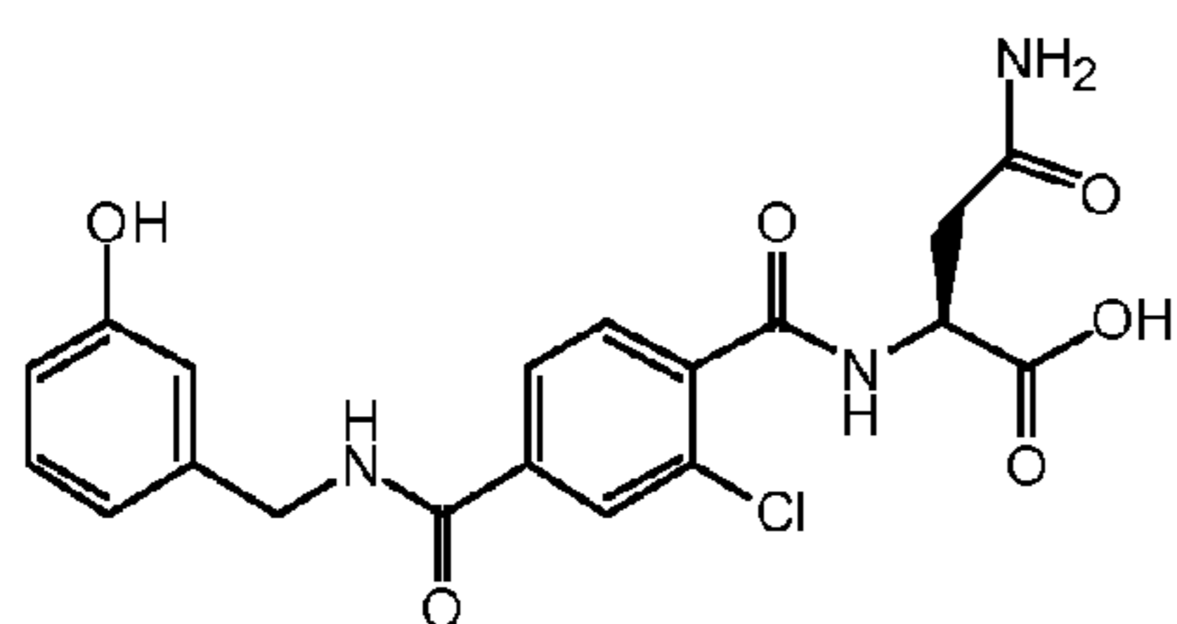
Compound 3
