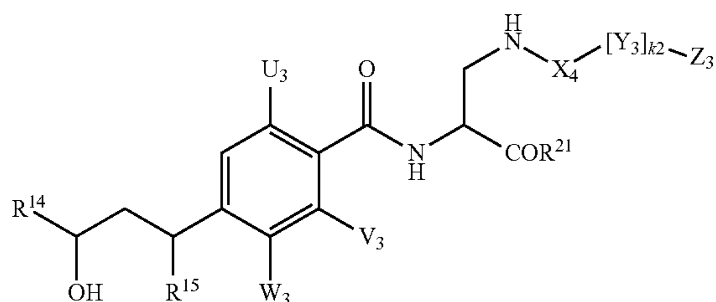
Formula V
