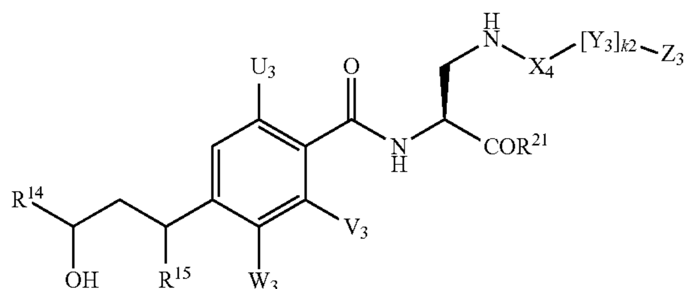
Formula V'
