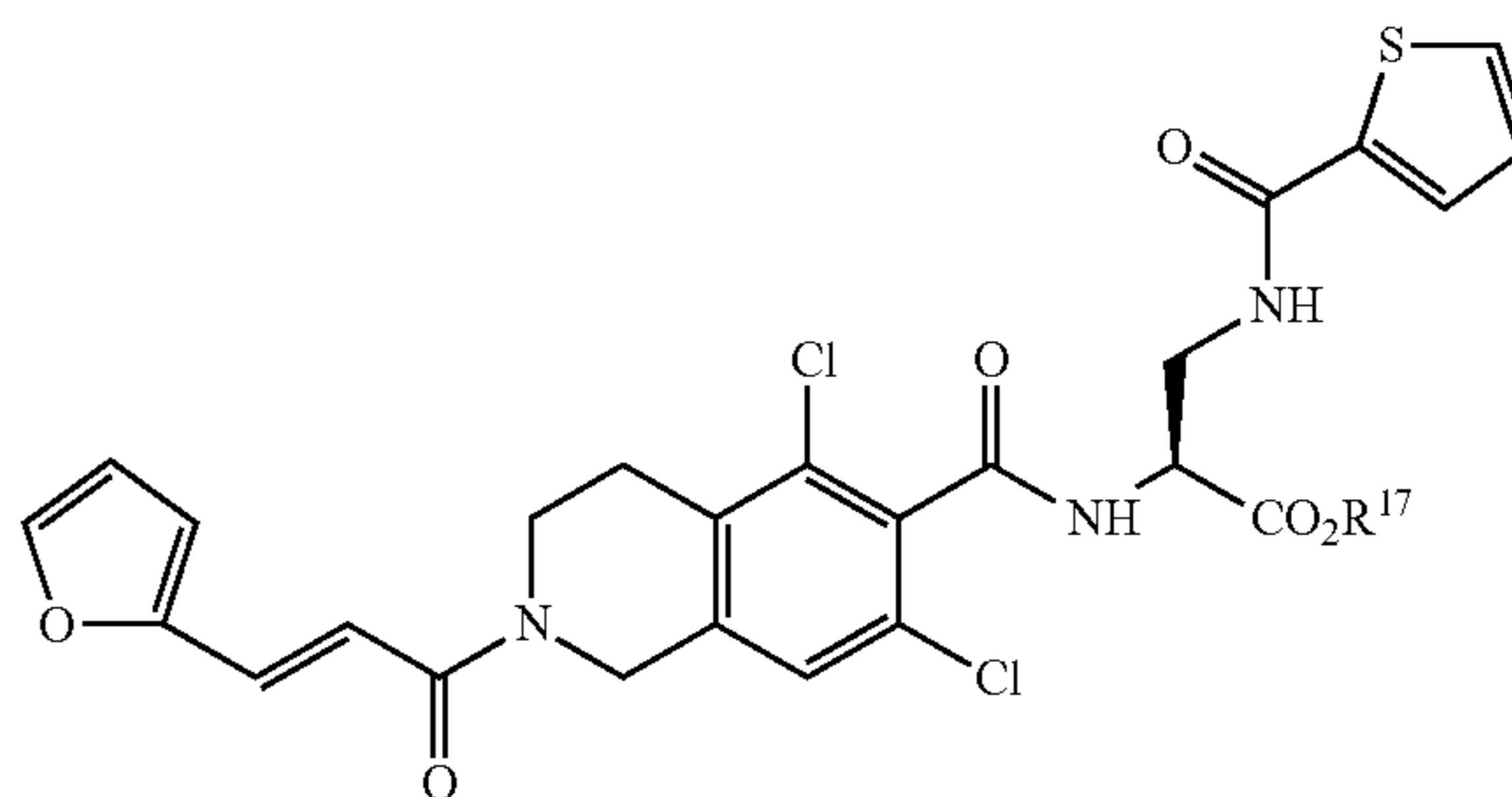
Formula IIA
