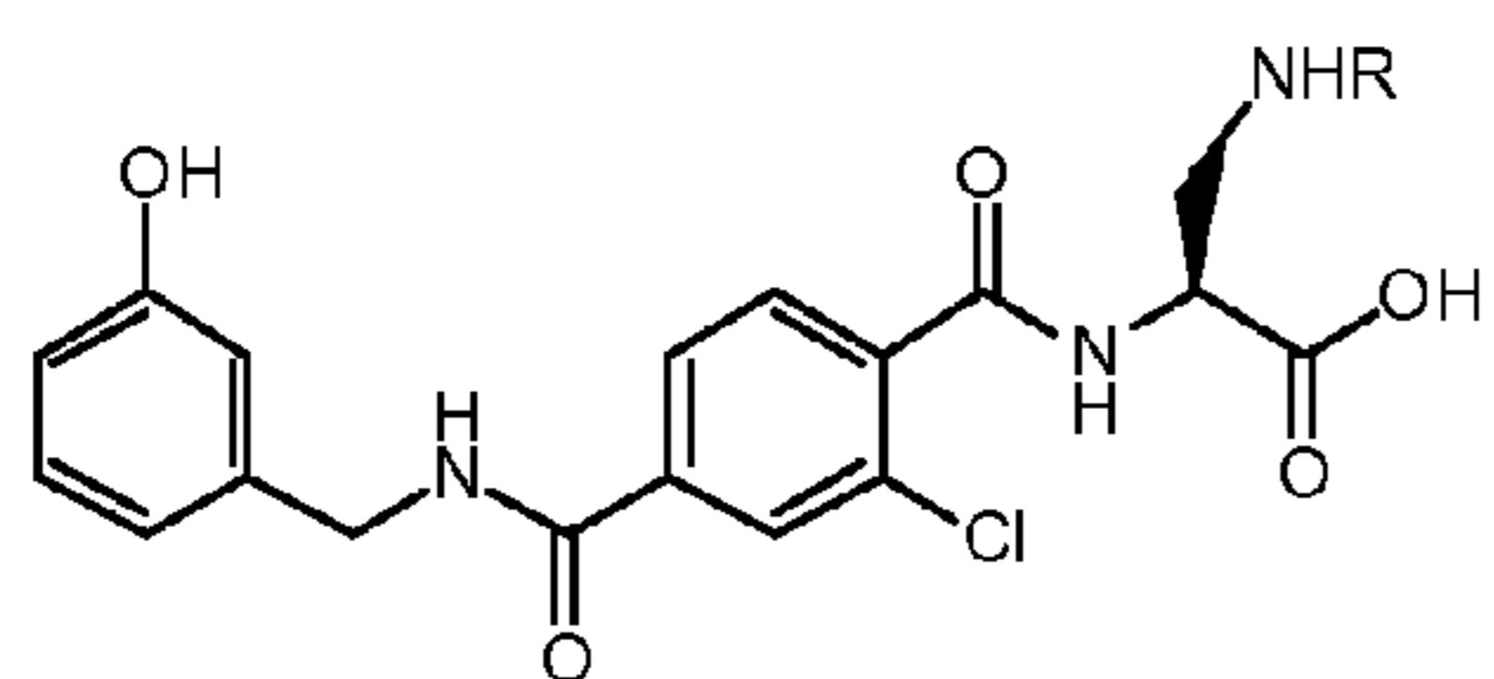
Compound 1, R = (C=S)NH-Fluorescein
