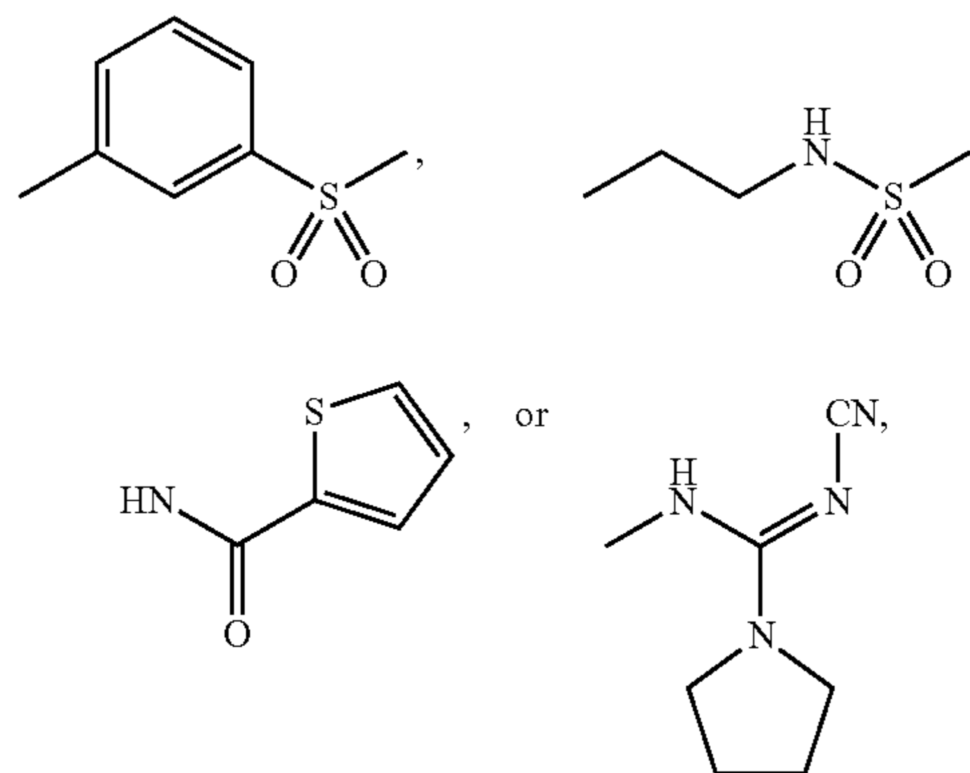
Formula II
