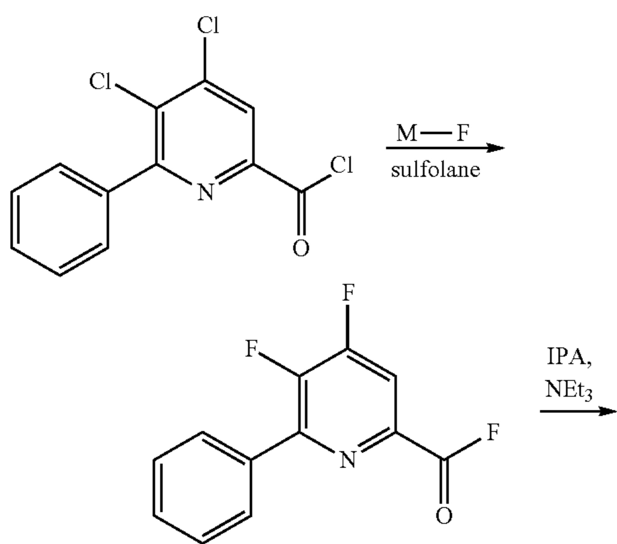
Scheme 4
