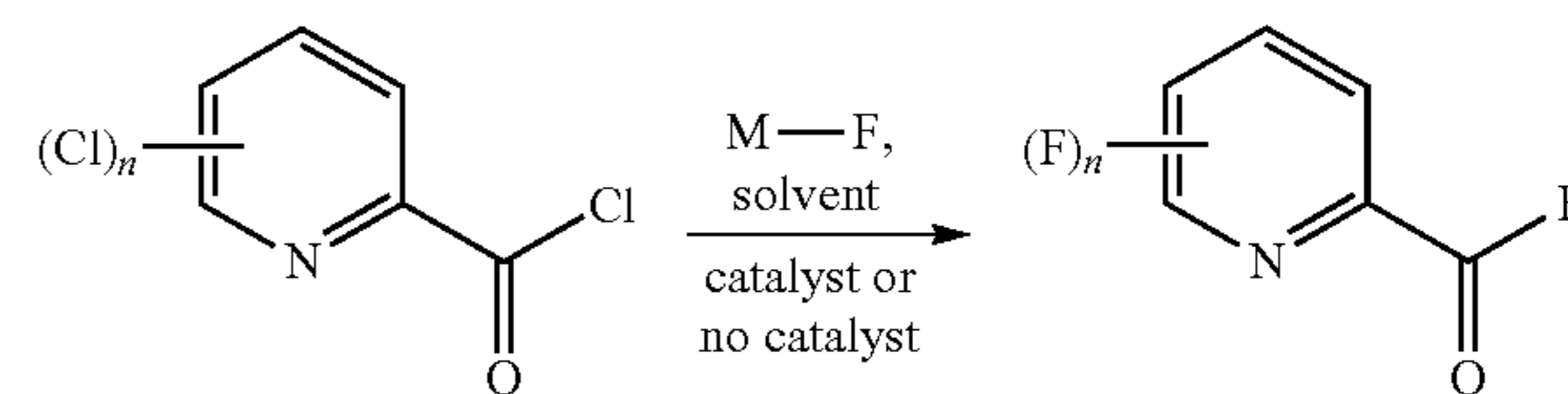
Scheme 1
