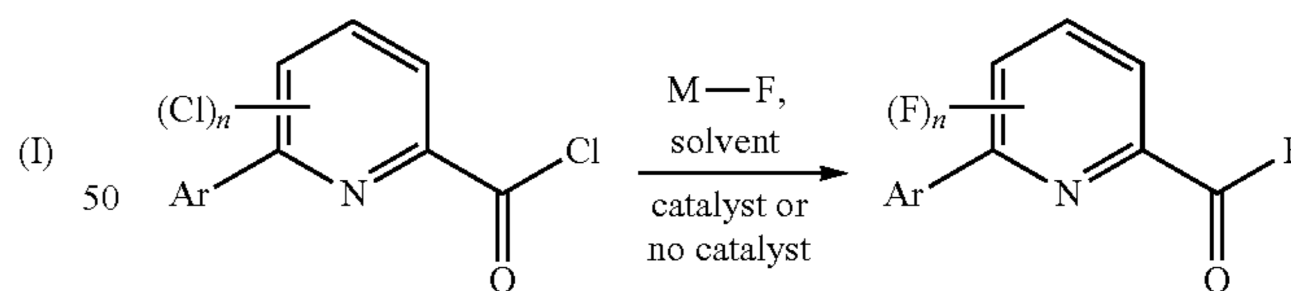
Scheme 2
