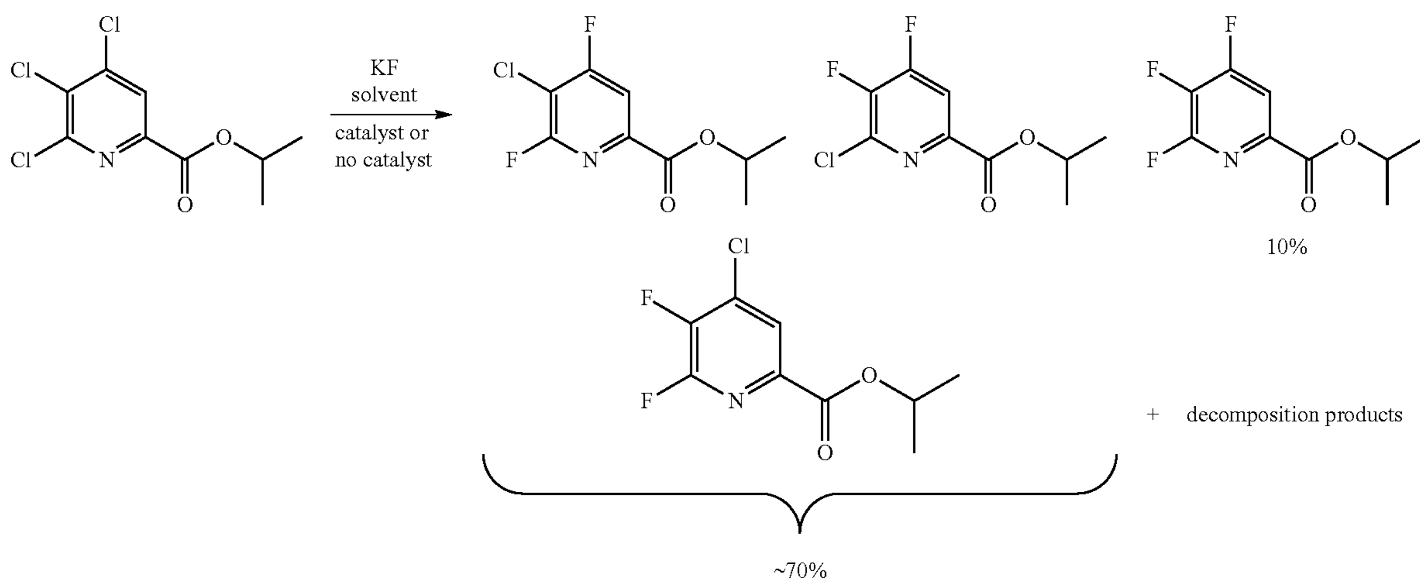
Scheme 5
