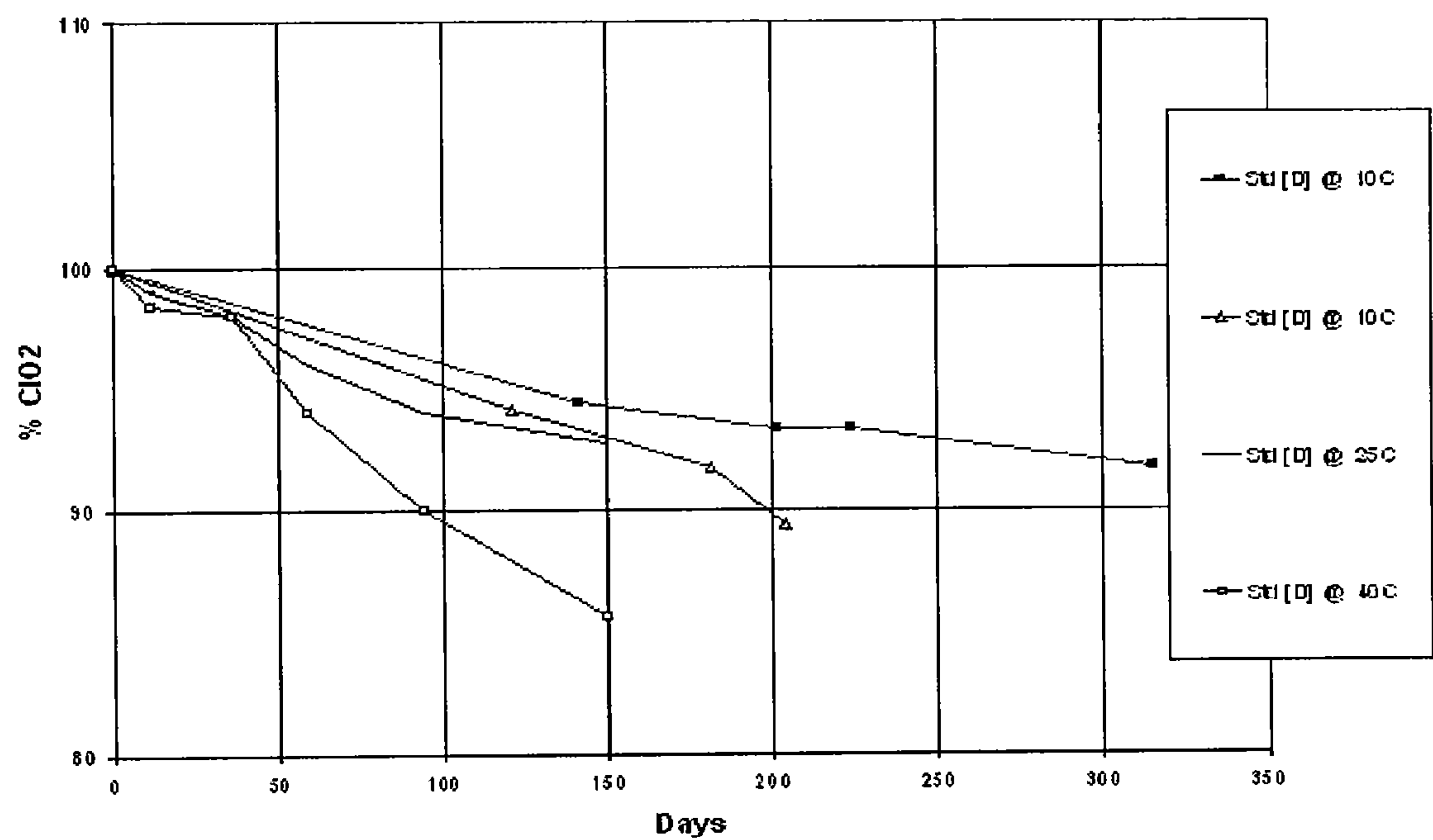
Figure 2: ClO 2 Stability In Glass Bottles Beginning At 4500 ppm
