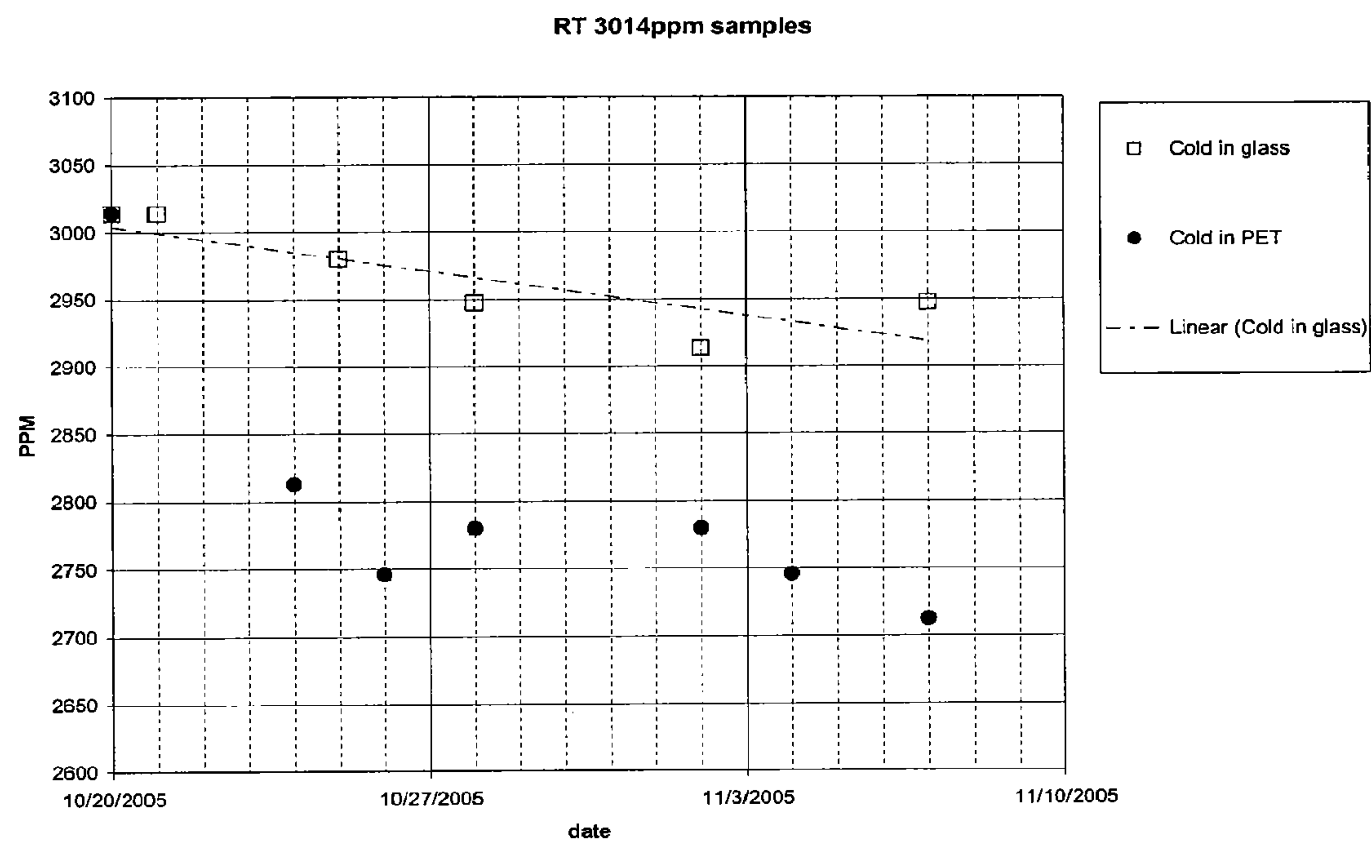
Figure 6 – Solutions Stored In PET Bottles
