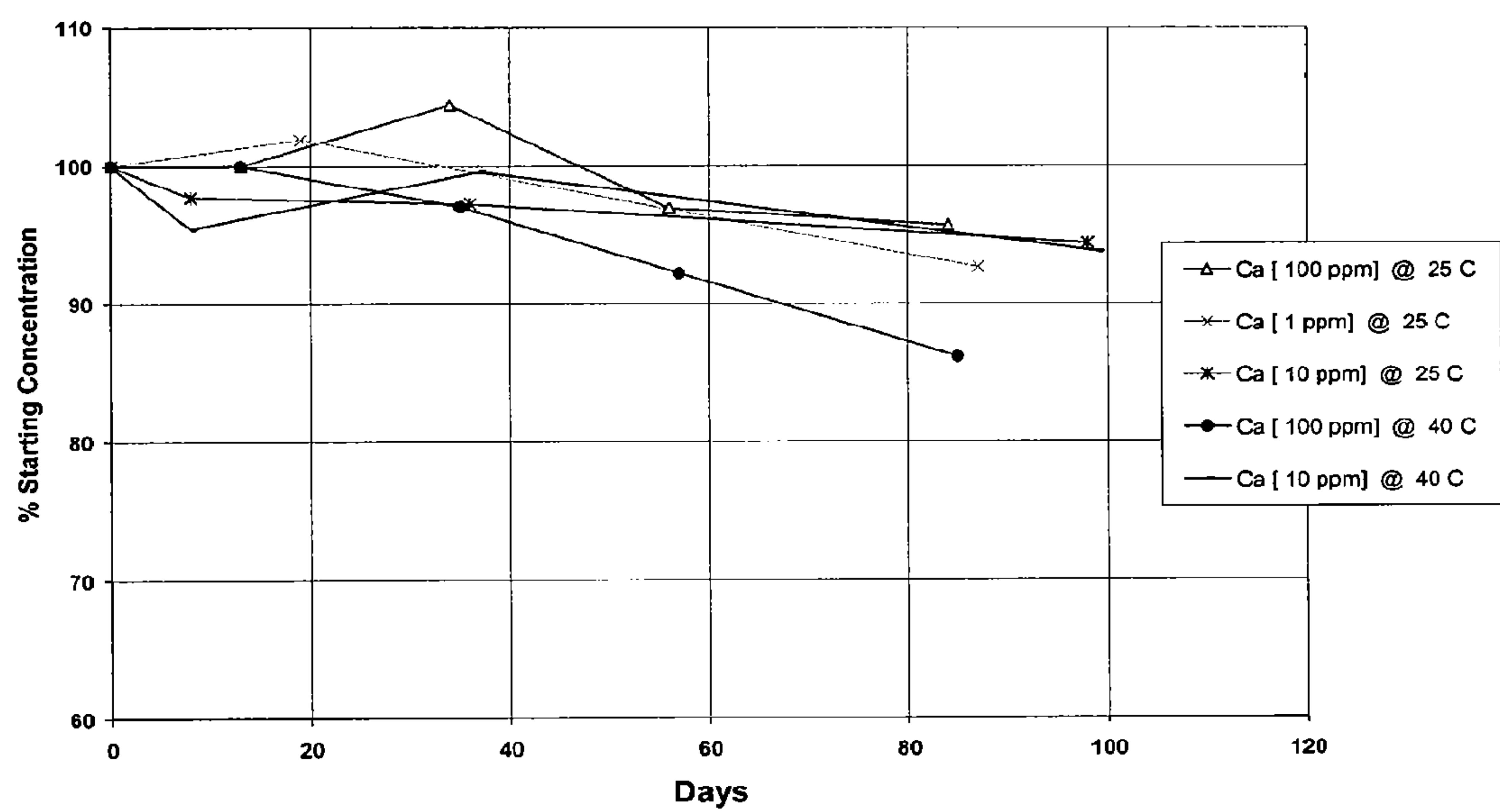
Figure 8 - Low Levels of CaCl2 in Deionized Water
