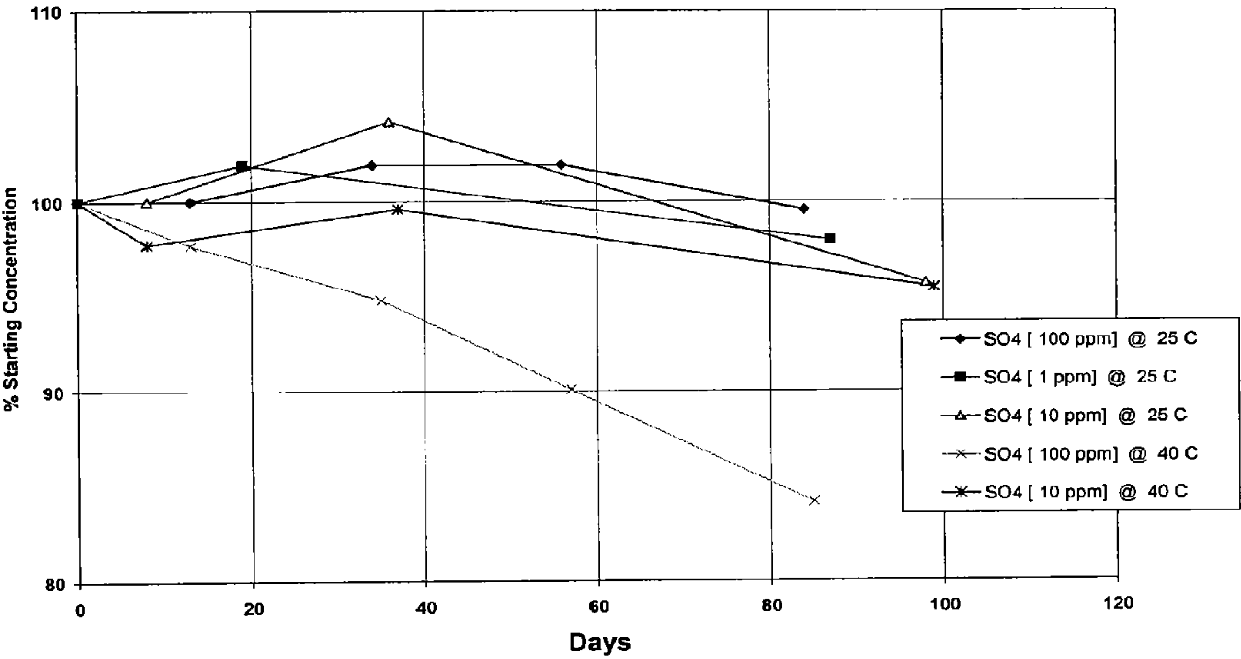
Figure 9 -Low Levels of Na2SO4 in Deionized Water
