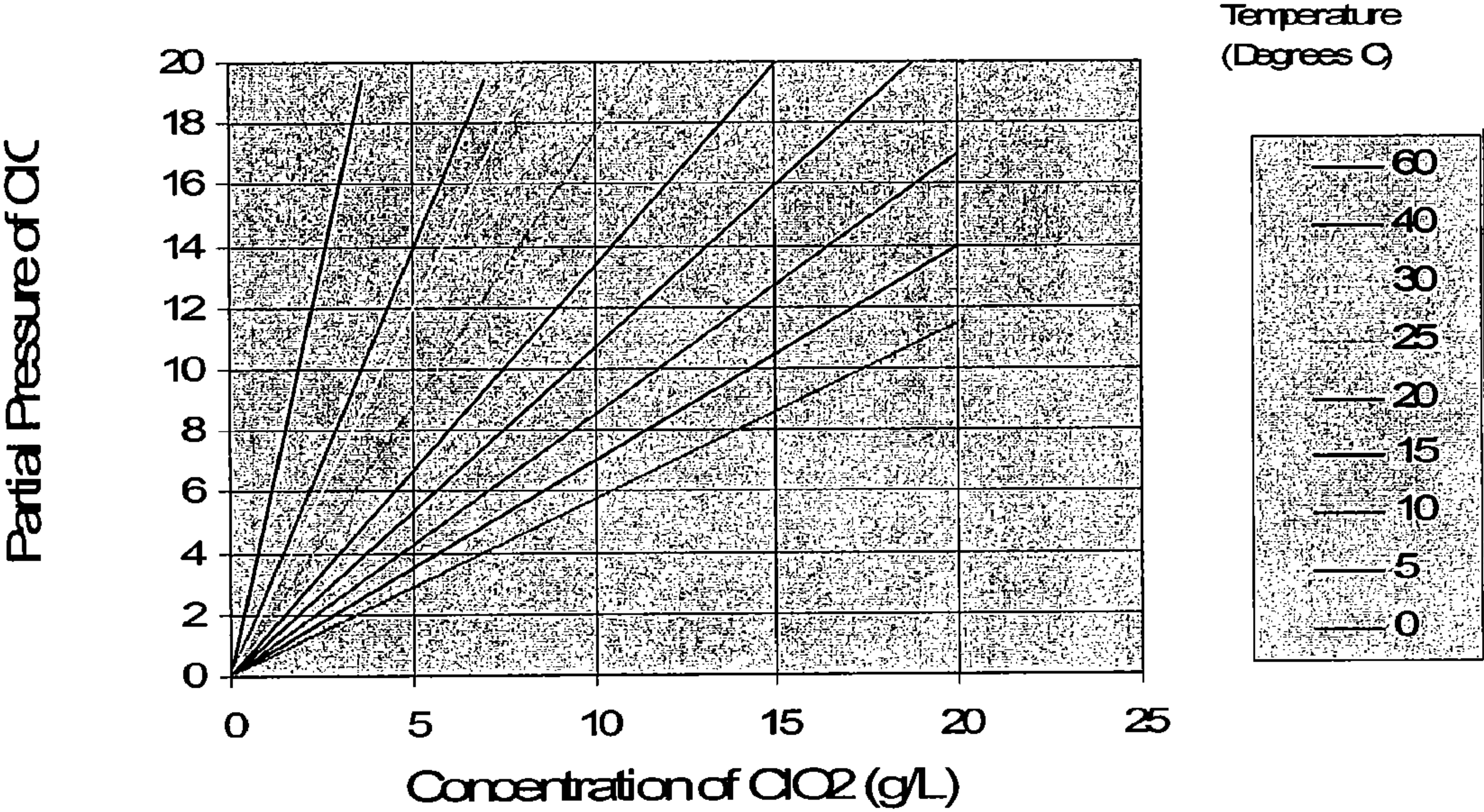
Figure 1 - Solubility of Chlorine Dioxide in Water
