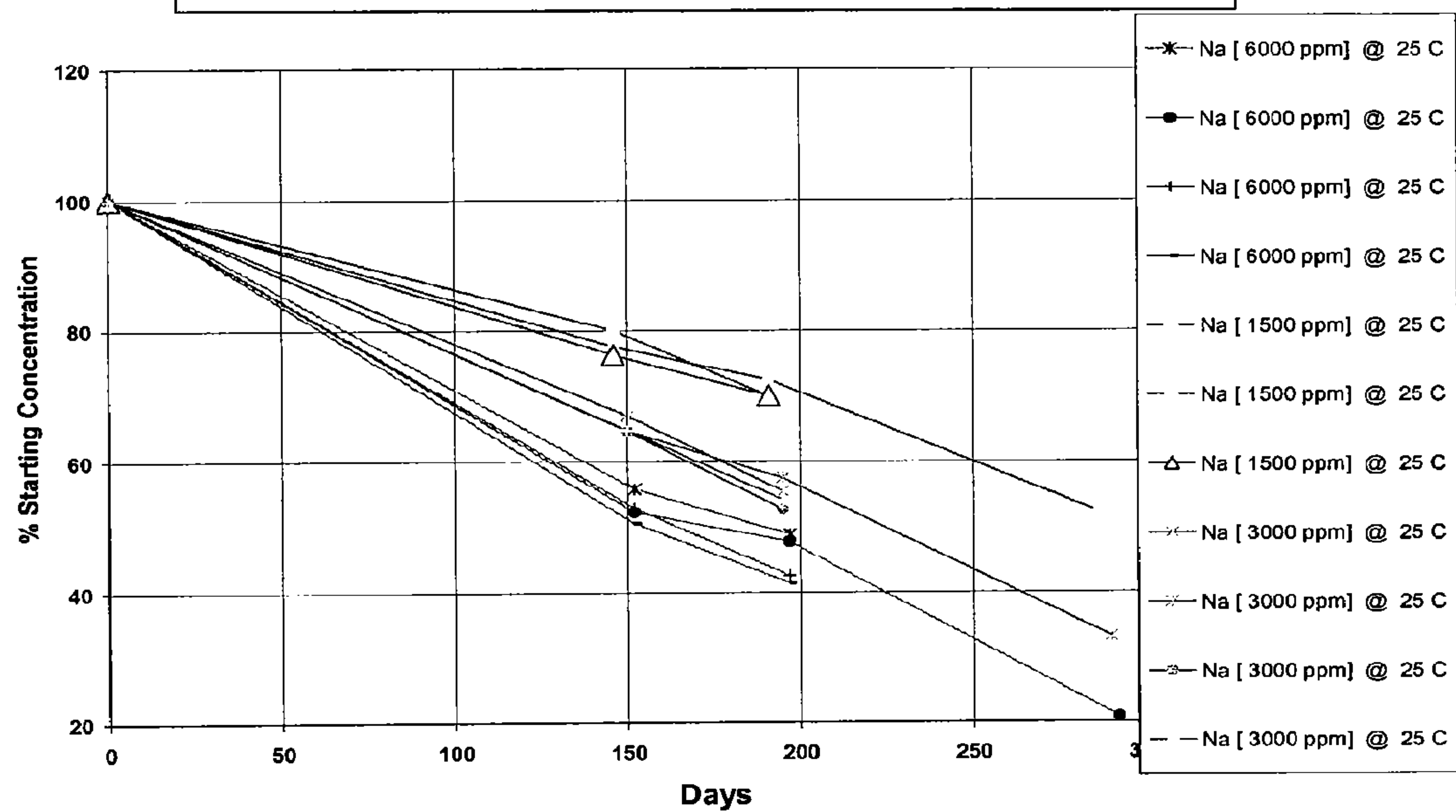
Figure 4 - High Levels of NaCl in Deionized Water
