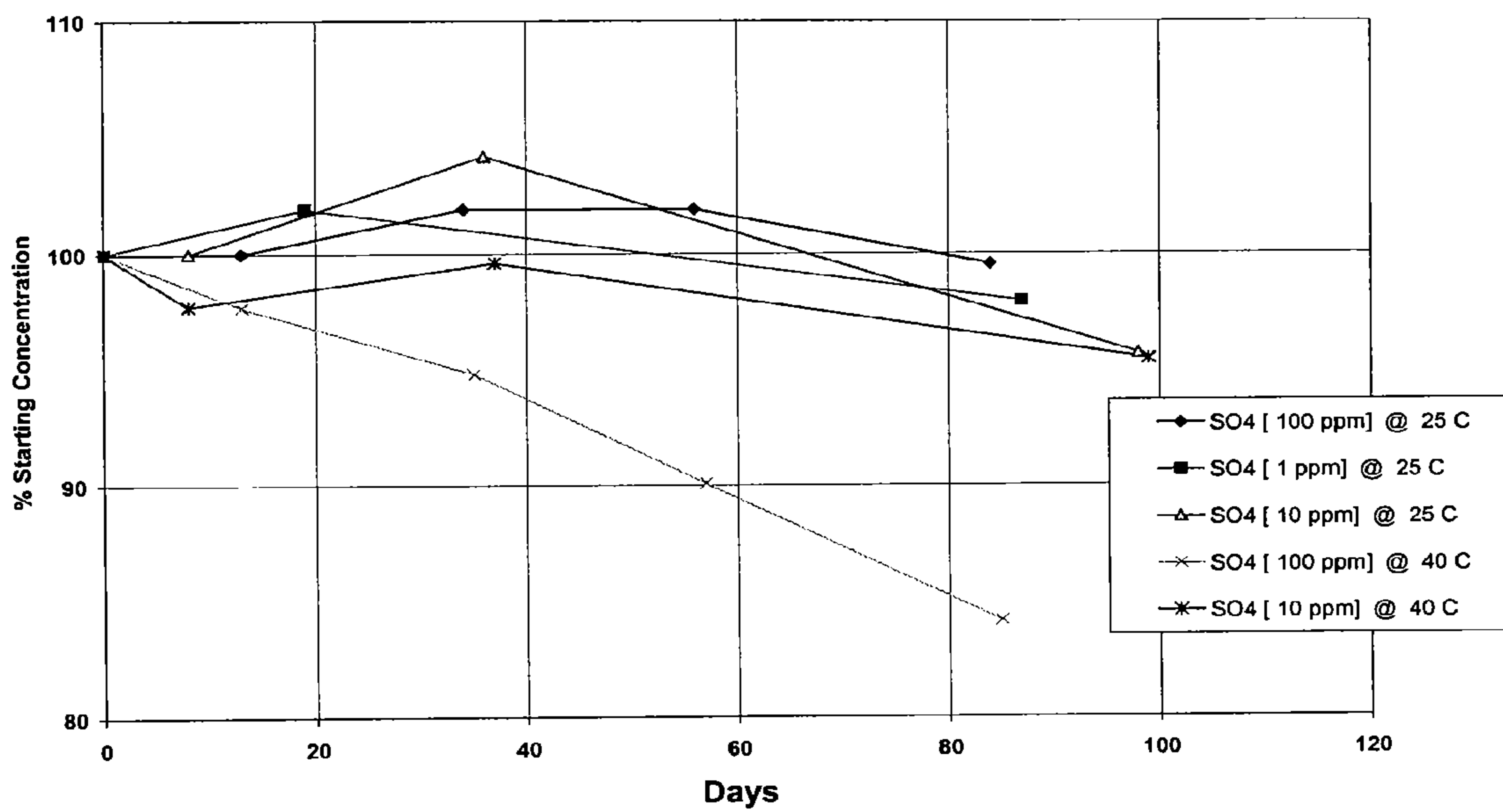
Figure 9 -Low Levels of Na2SO4 in Deionized Water
