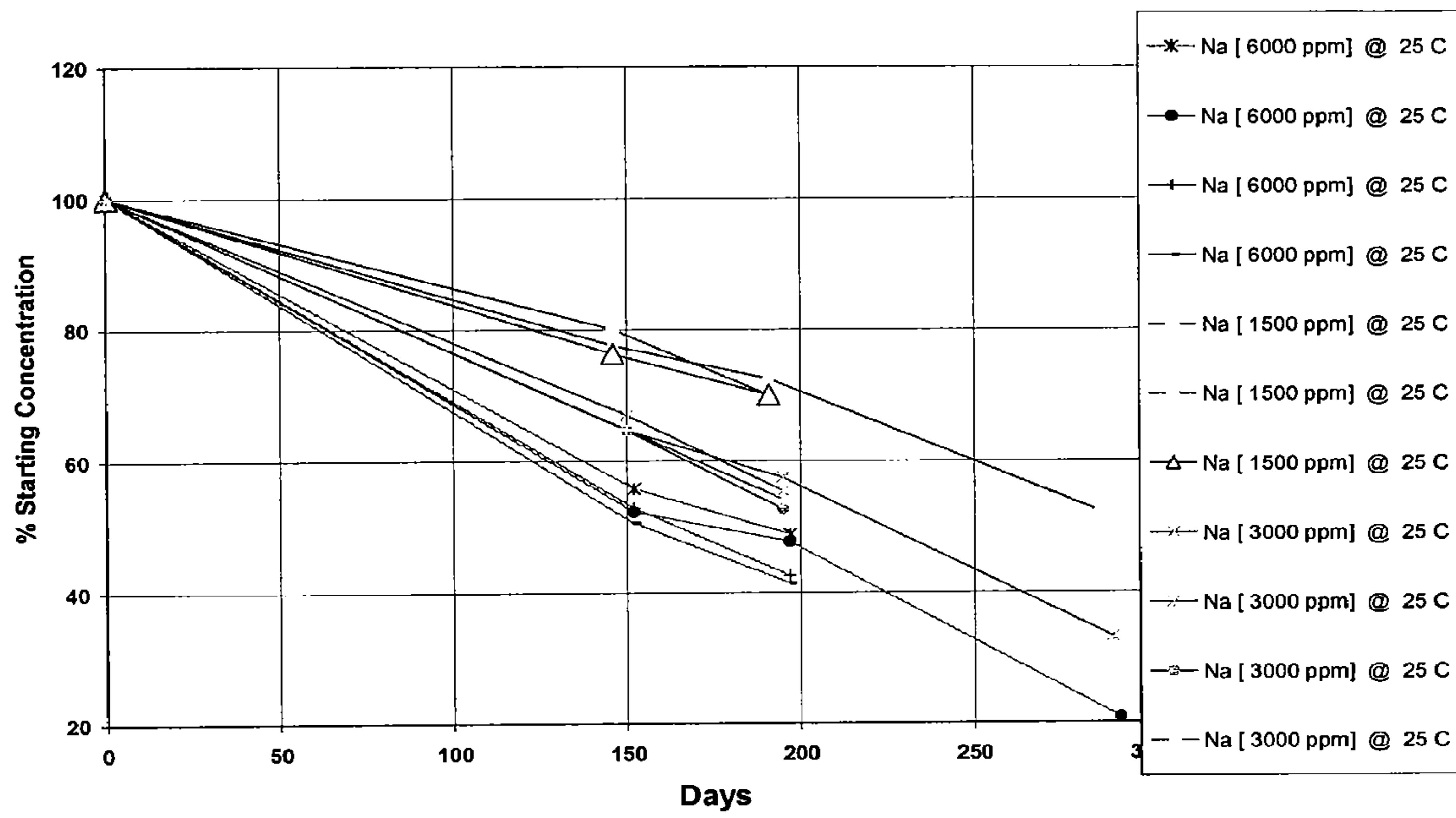
Figure 4 - High Levels of NaCl in Deionized Water
