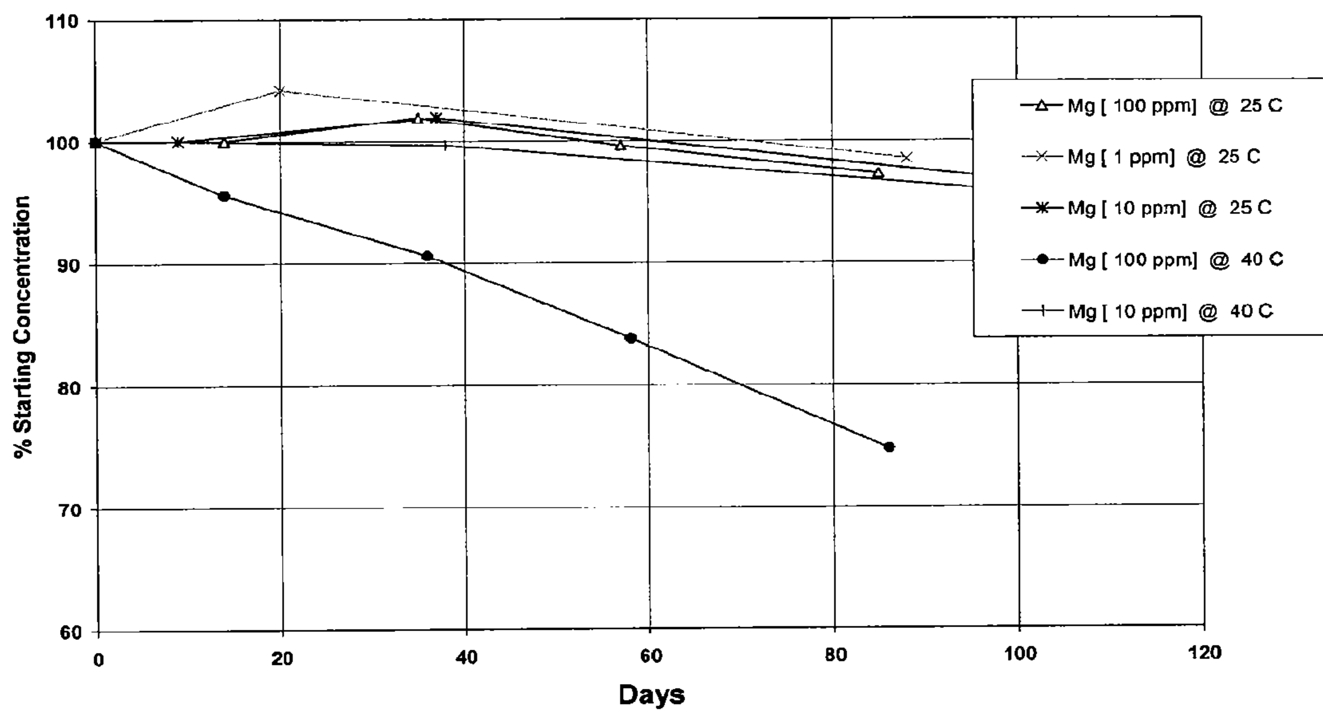
Figure 7 - Low Levels of MgCl 2 in Deionized Water
