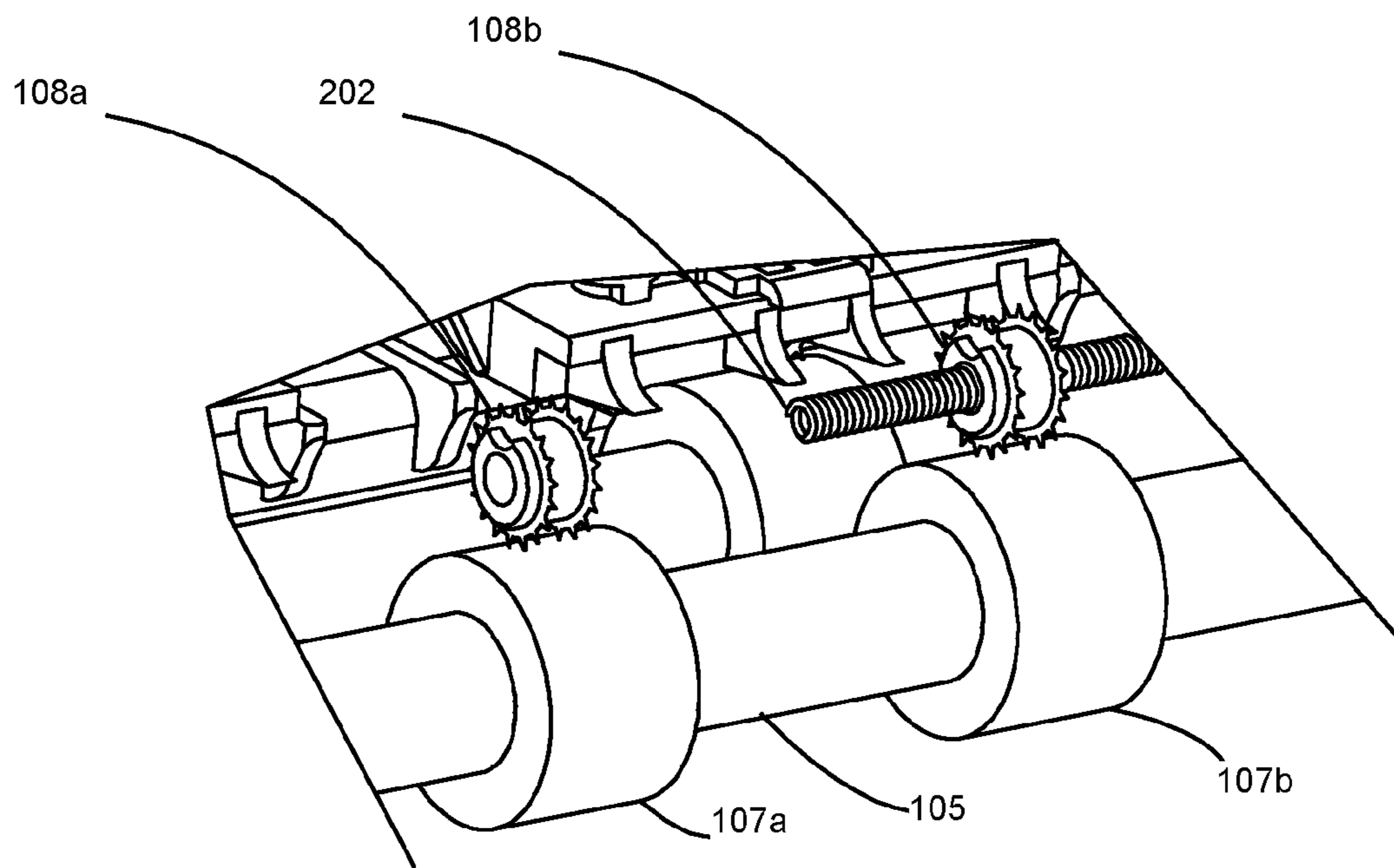
Figure 2 Prior Art
