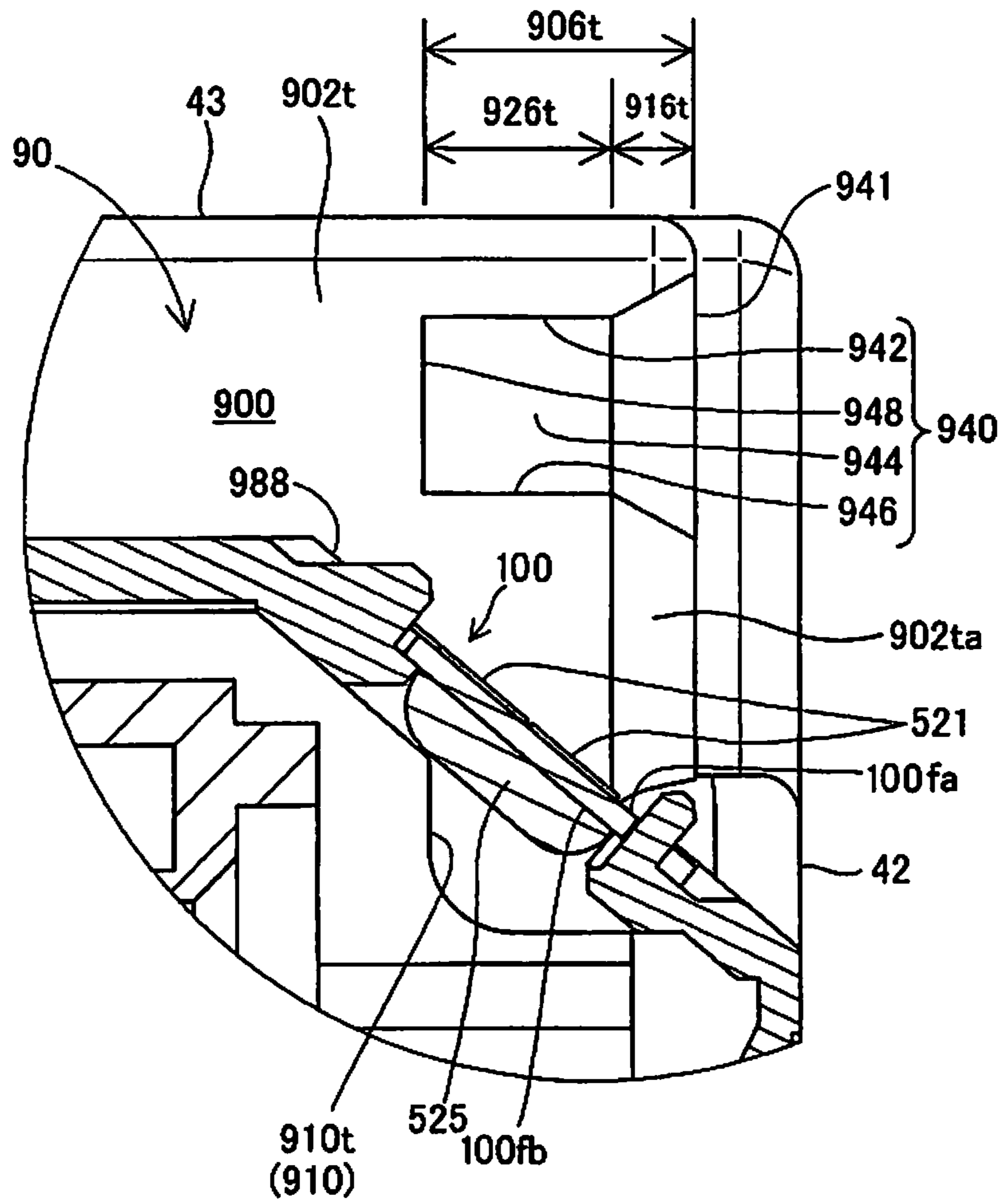
19b-19b CROSS SECTION VIEW
