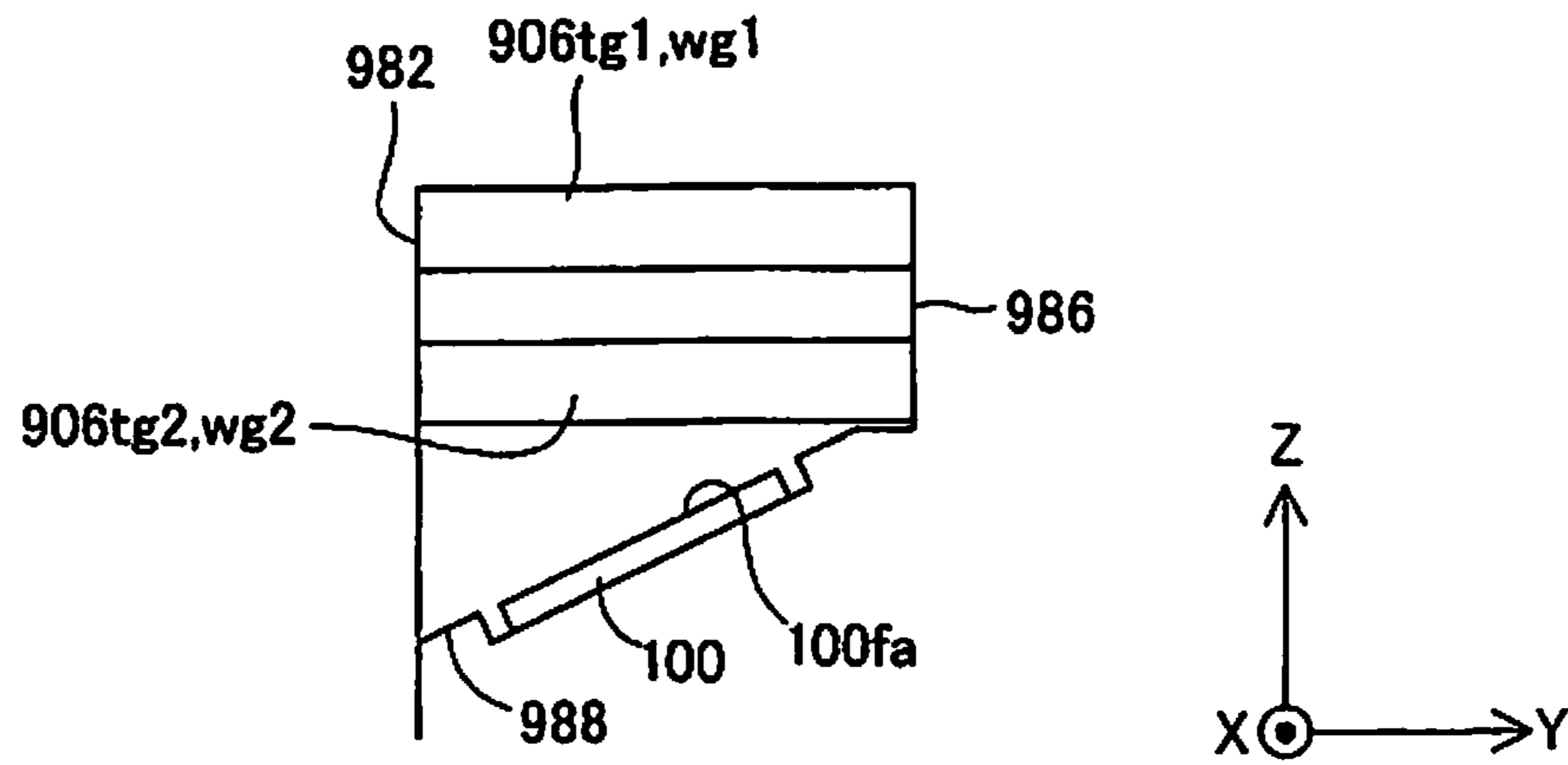
32-32 CROSS SECTION VIEW
