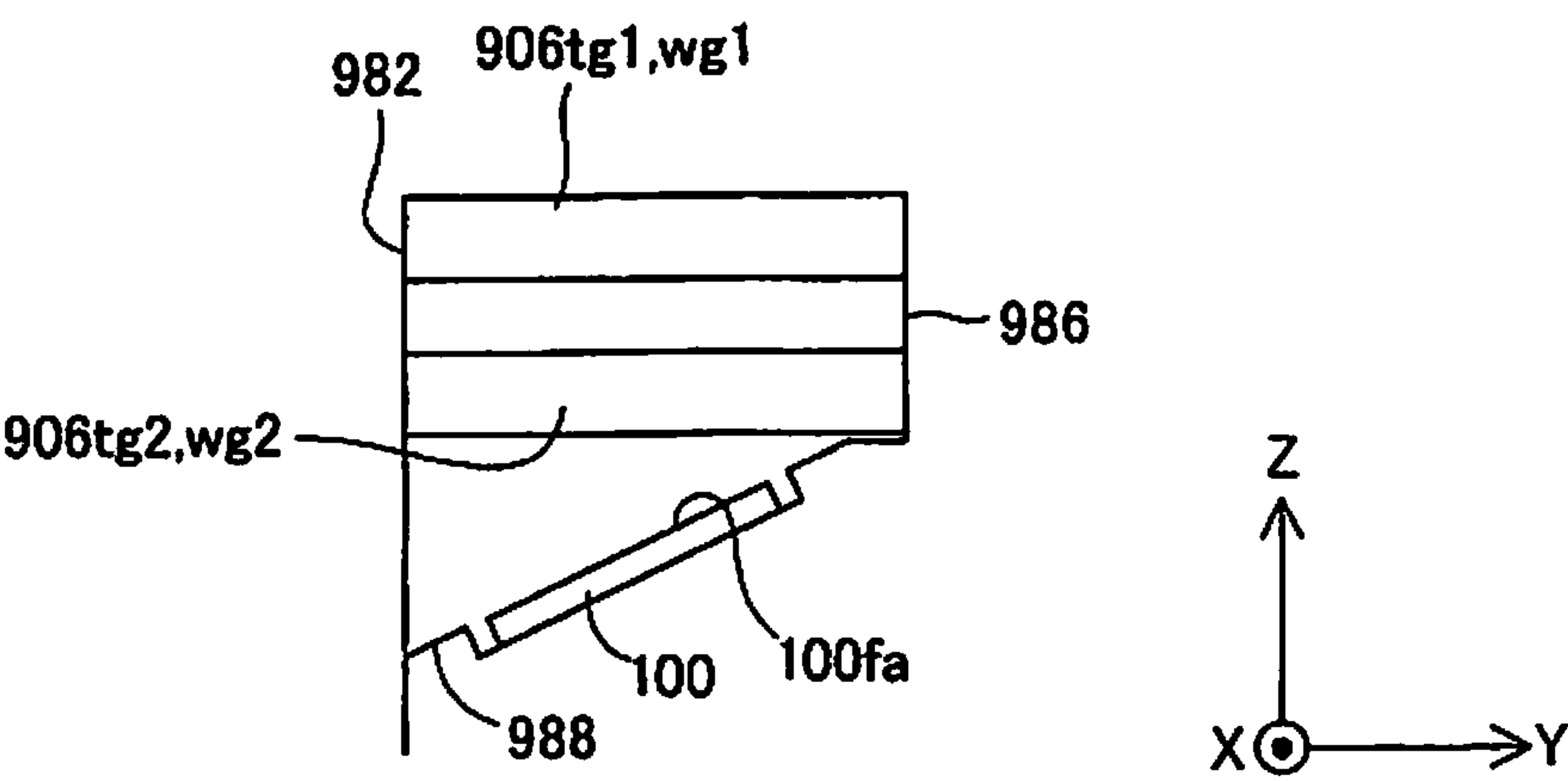
32-32 CROSS SECTION VIEW
