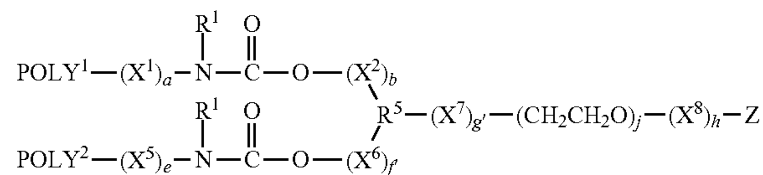
(Formula III)
