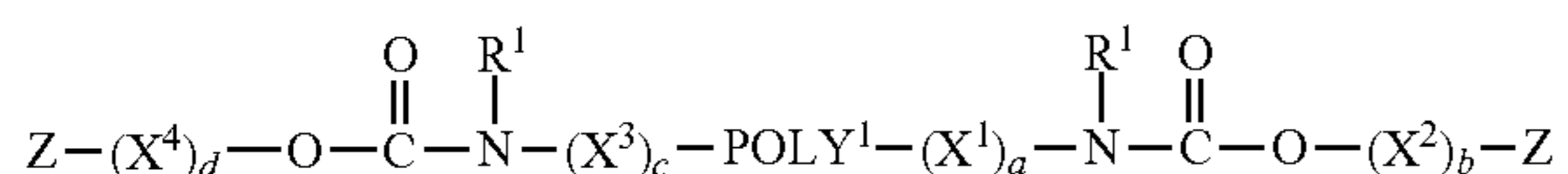
(Formula IIa)
