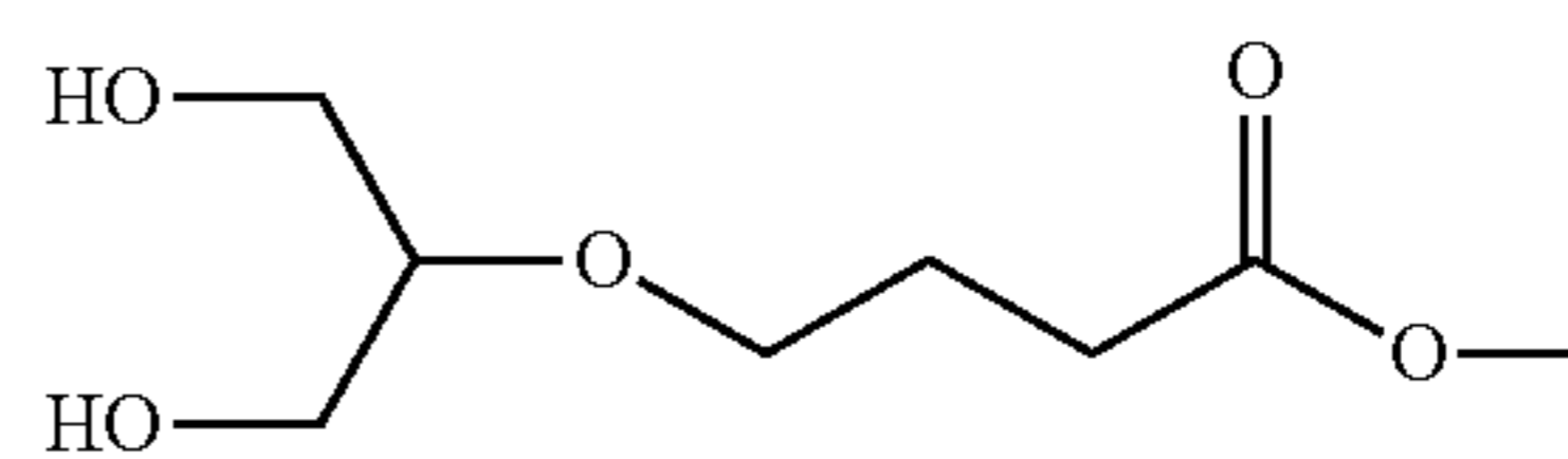
a glycerol-based precursor molecule (Compound 8-02)
