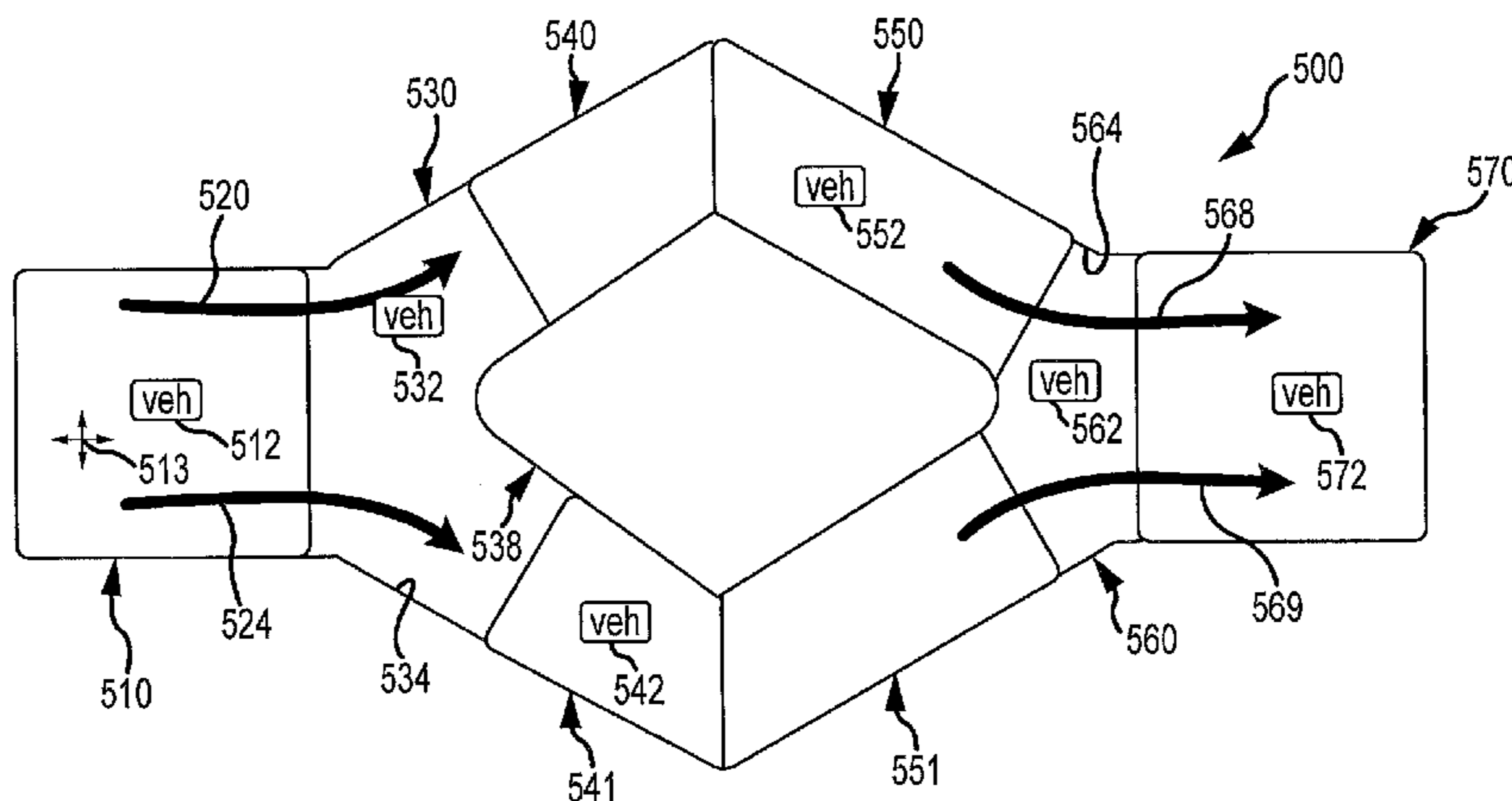
DYNAMIC BOUNDARIES SPLITTING AND MERGING AROUND BRANCHING ELEMENTS
