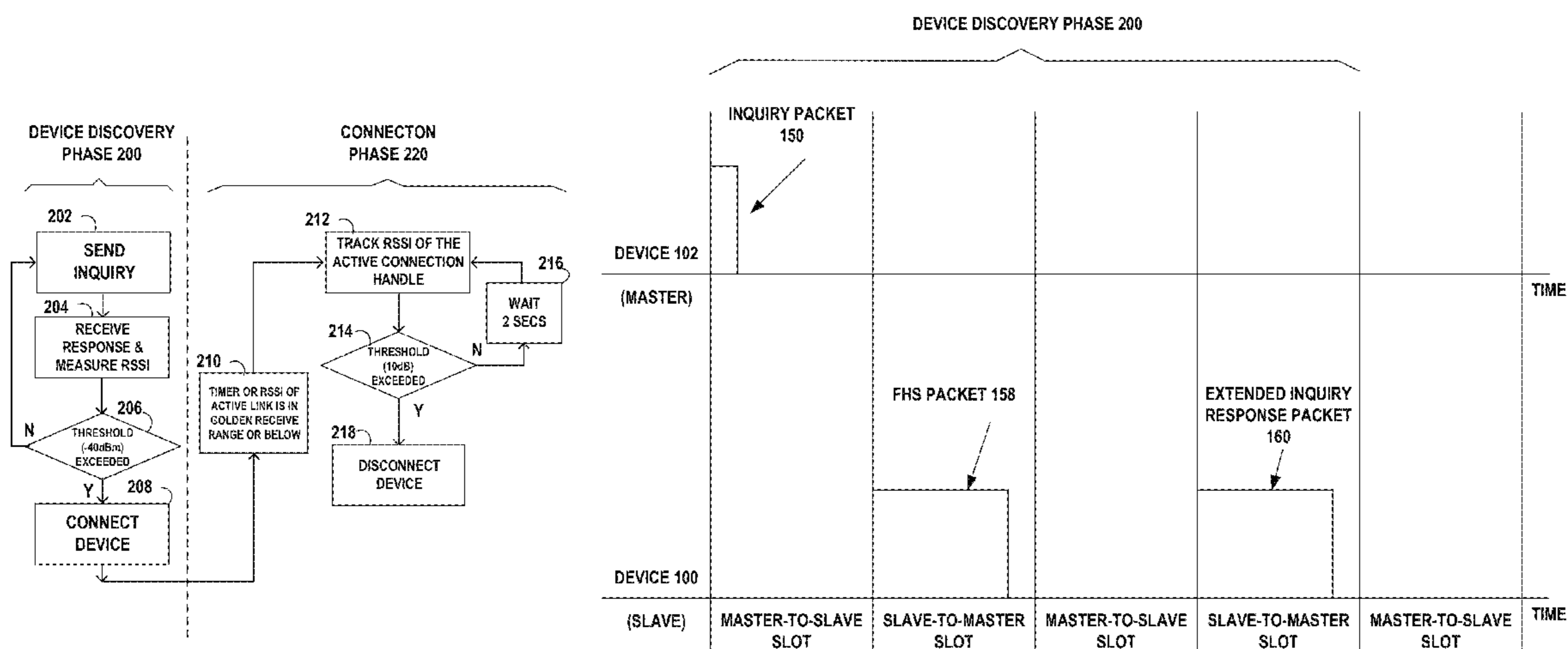
TIMING DURING A DEVICE DISCOVERY PROCESS, FOR EXAMPLE A BLUETOOTH INQUIRY PROCESS
