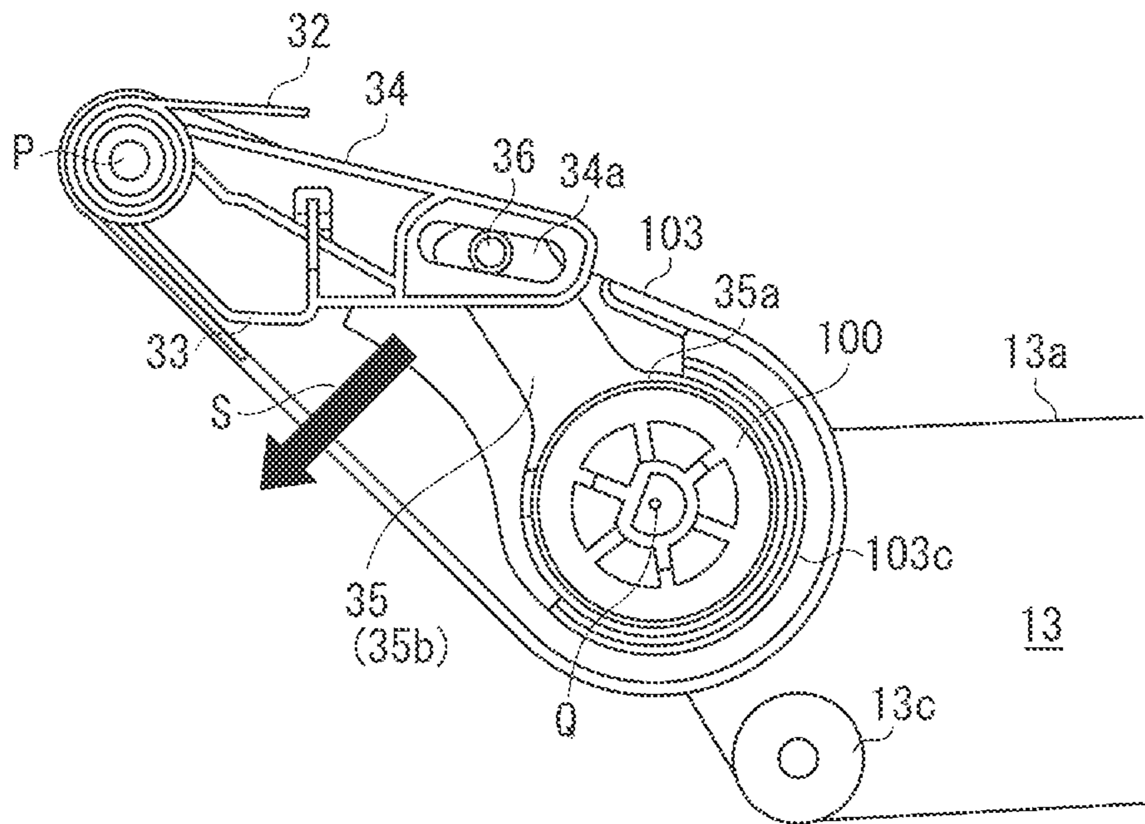
FIG. 9B DOOR CLOSED STATE
