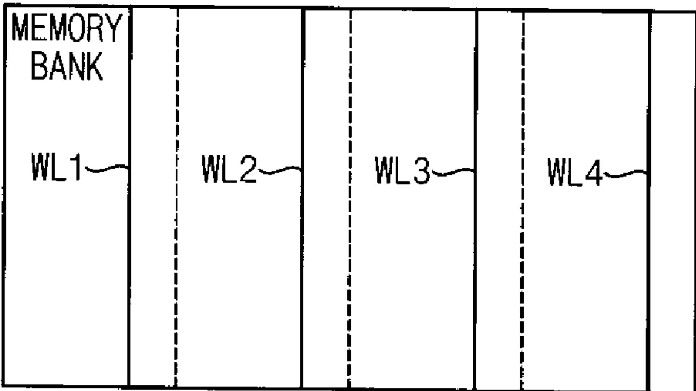
COUNTER-BASED REFRESH
