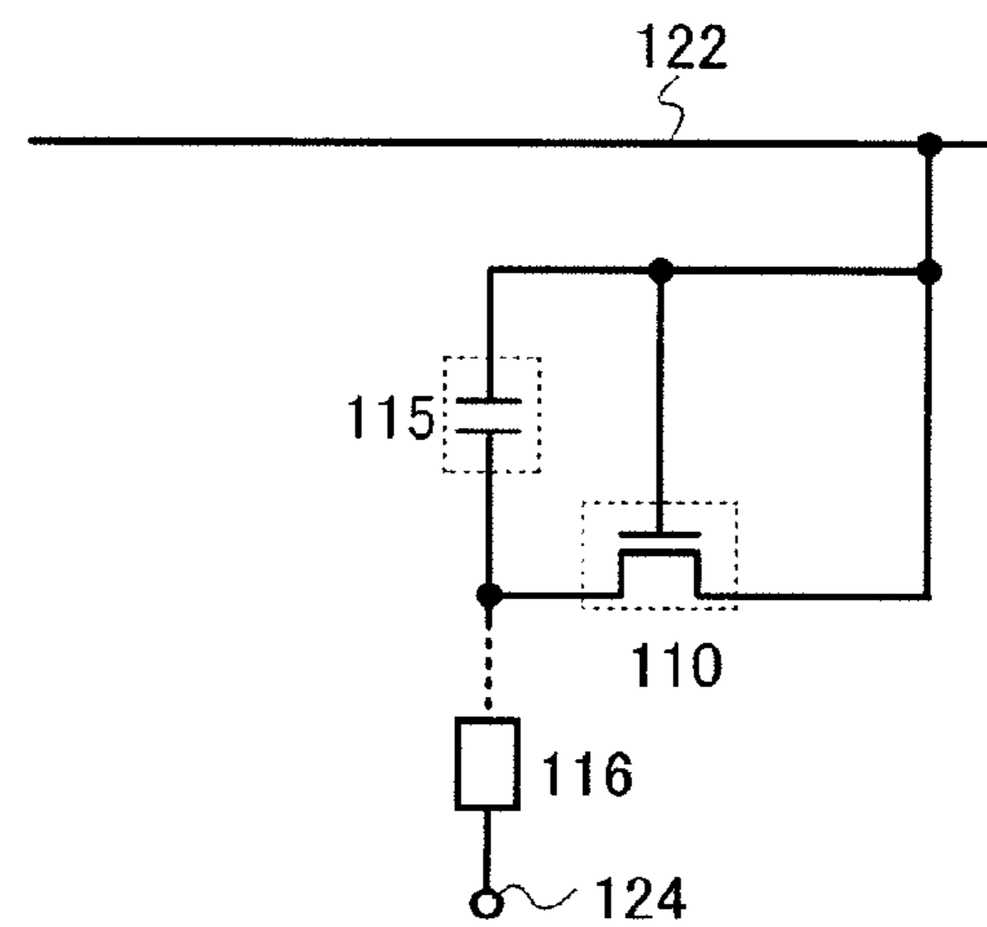
FIG. 44B threshold voltage writing
