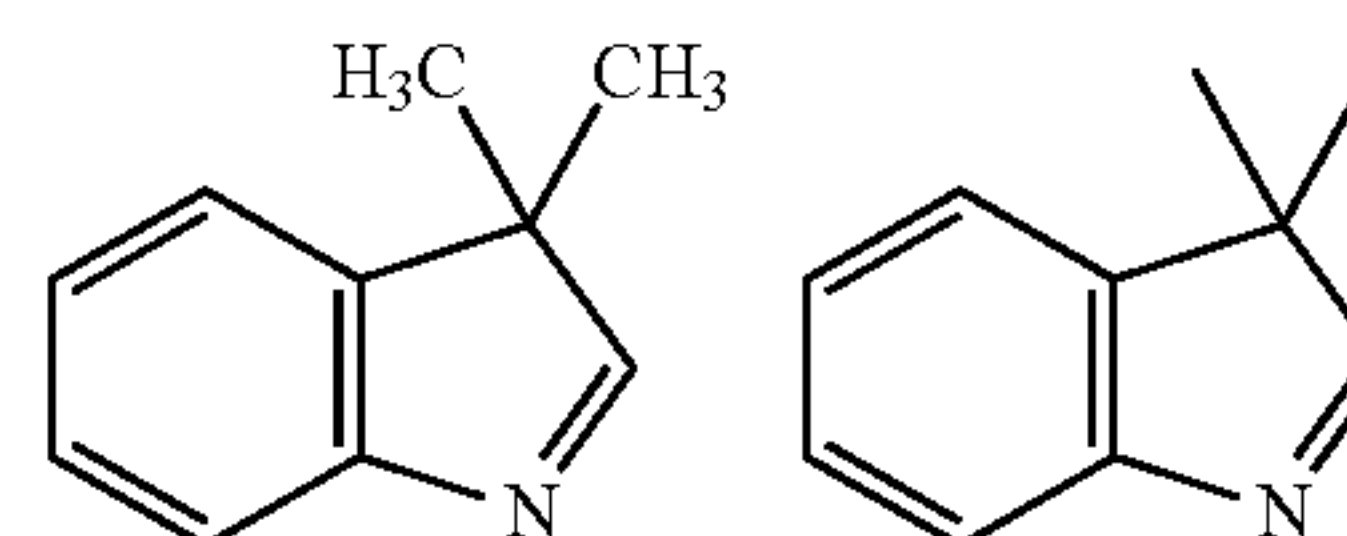
3,3-Dimethylindolenine (3,3-Dimethyl-3H-indole)
