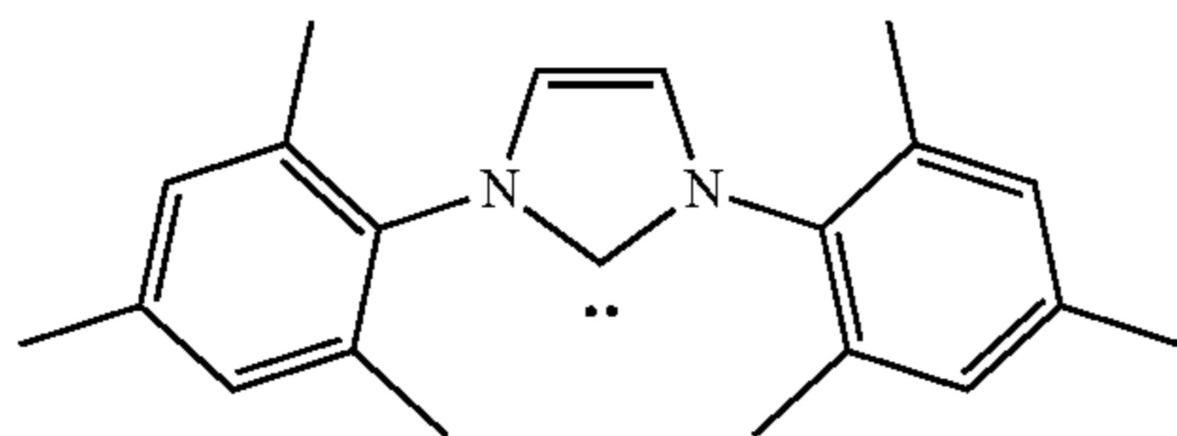
1,3-Bis(2,4,6-trimethylphenyl)imidazol-2-ylidene (Im-2)
