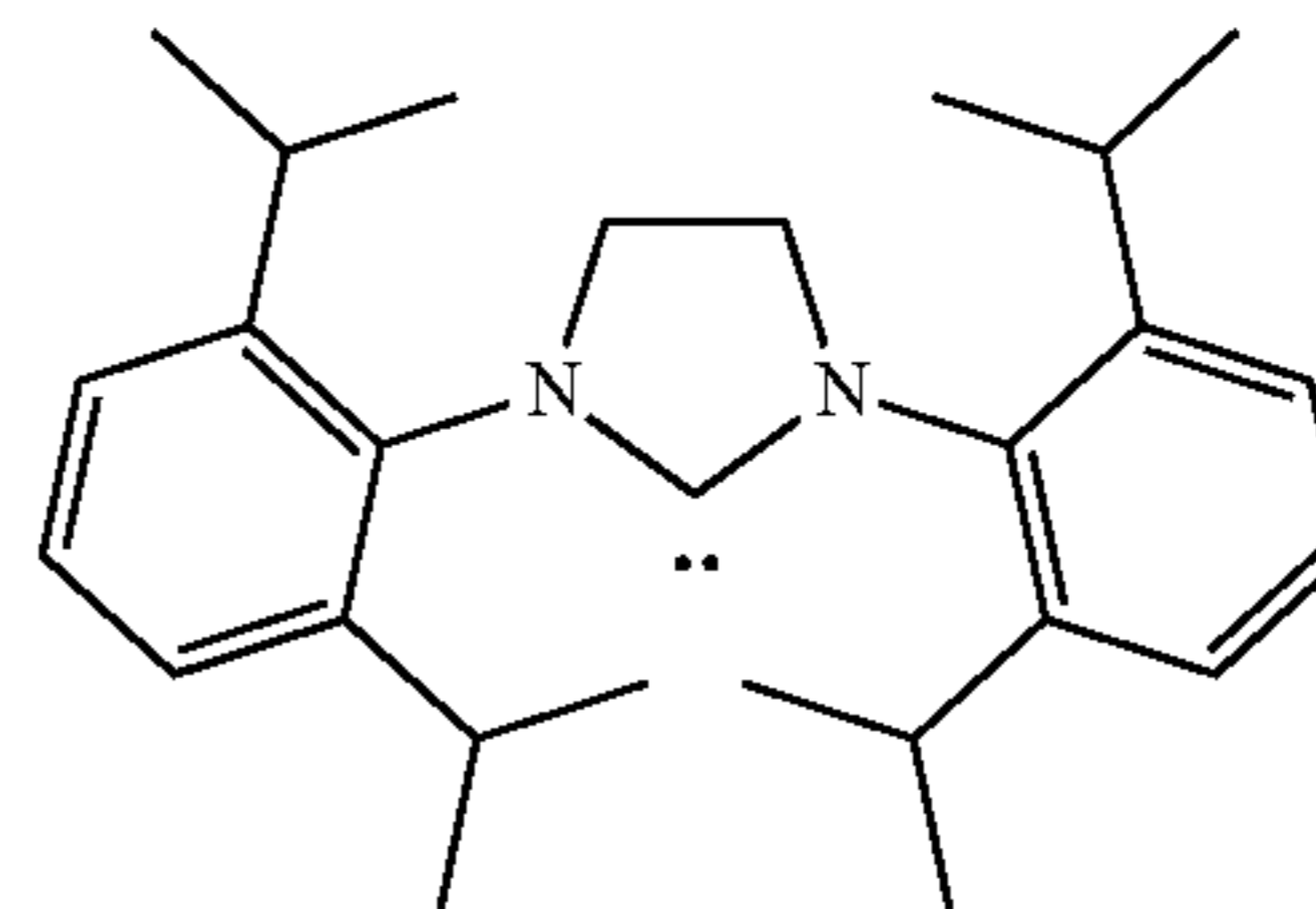
1,3-Bis(2,6-di-i-propylphenyl)-4,5-dihydroimidazol-2-ylidene (Im-8)
