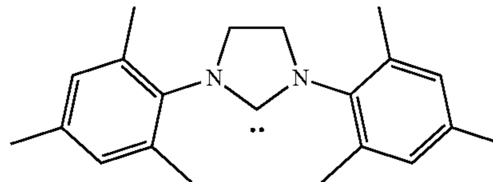
1,3-Bis(2,4,6-trimethylphenyl)-4,5-dihydroimidazol-2-ylidene (Im-7)
