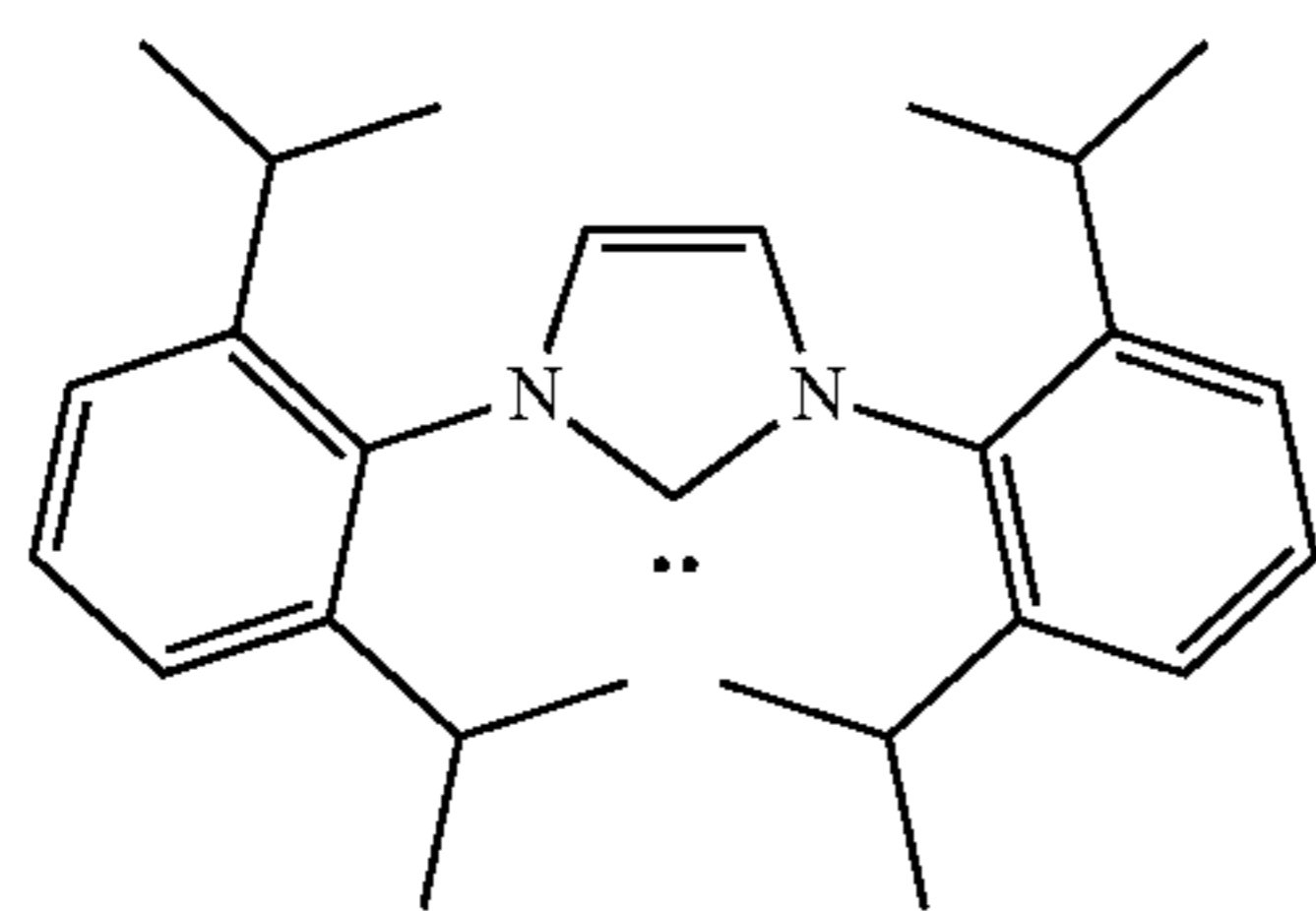
1,3-Bis(2,6-di-i-propylphenyl)imidazol-2-ylidene (Im-3)
