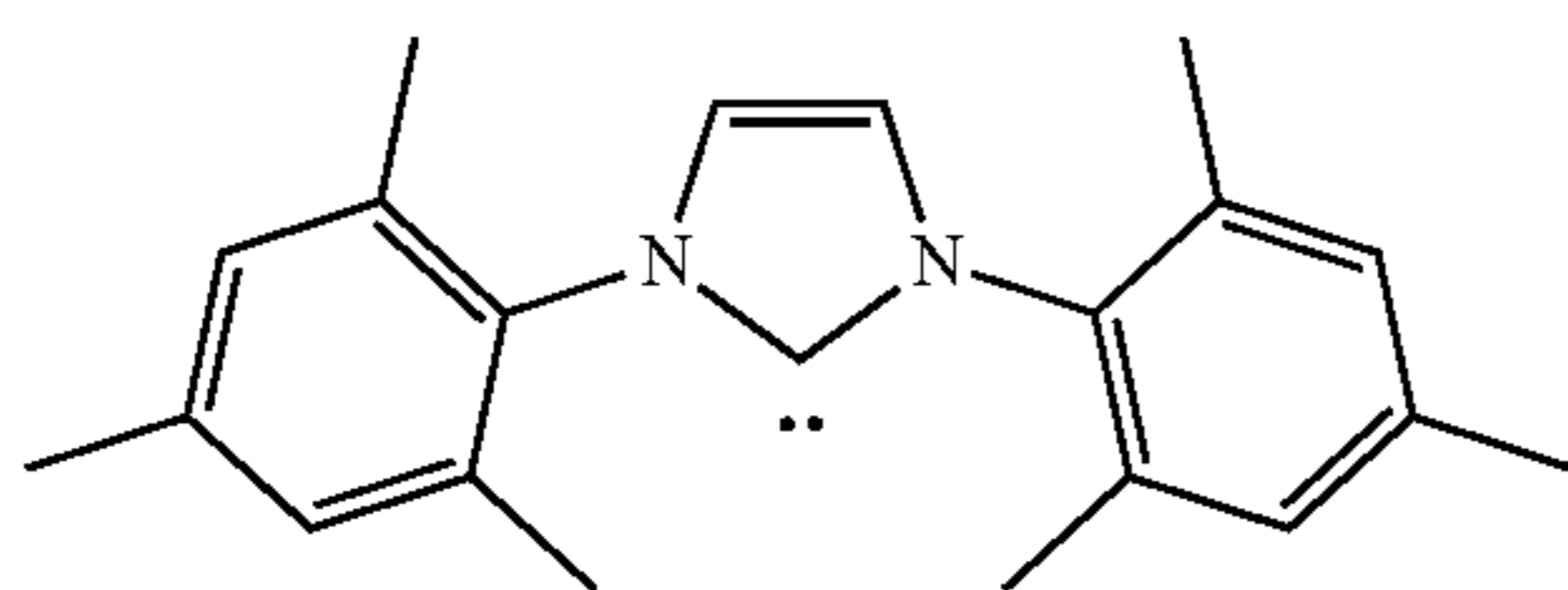
1,3-Bis(2,4,6-trimethylphenyl)imidazol-2-ylidene (Im-2)
