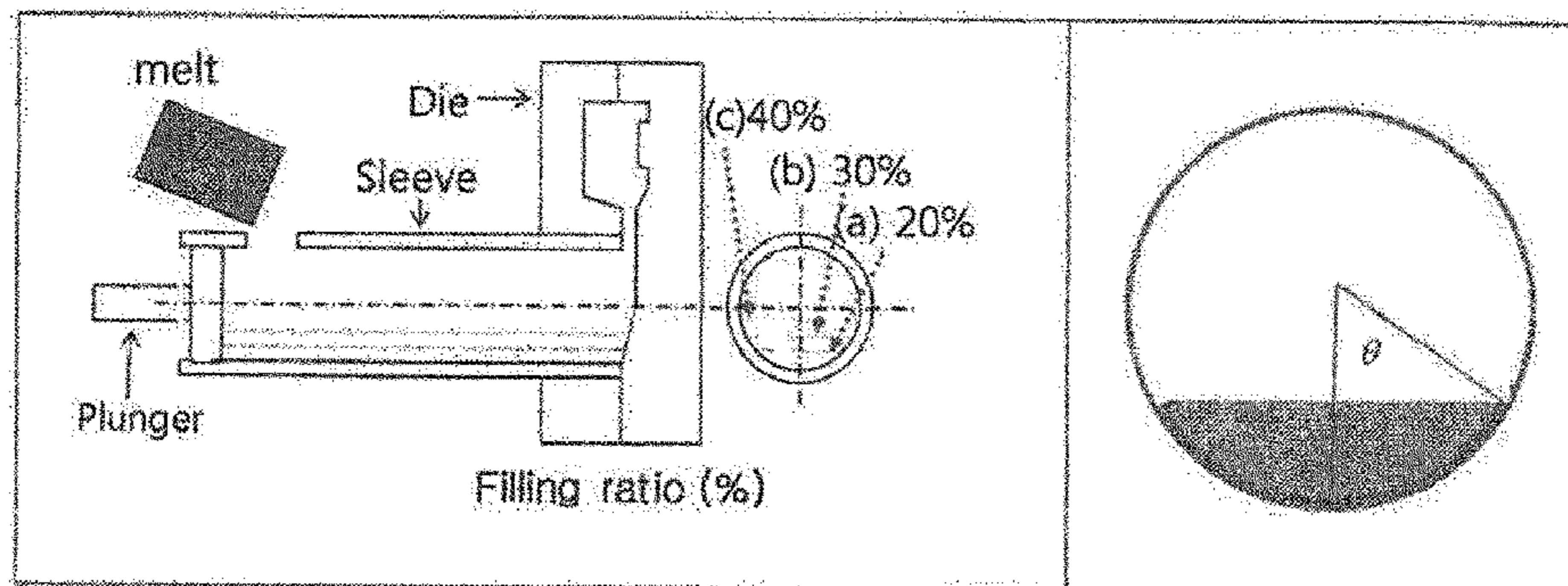
Filling Proportion of Melt in a Space of Sleeve
