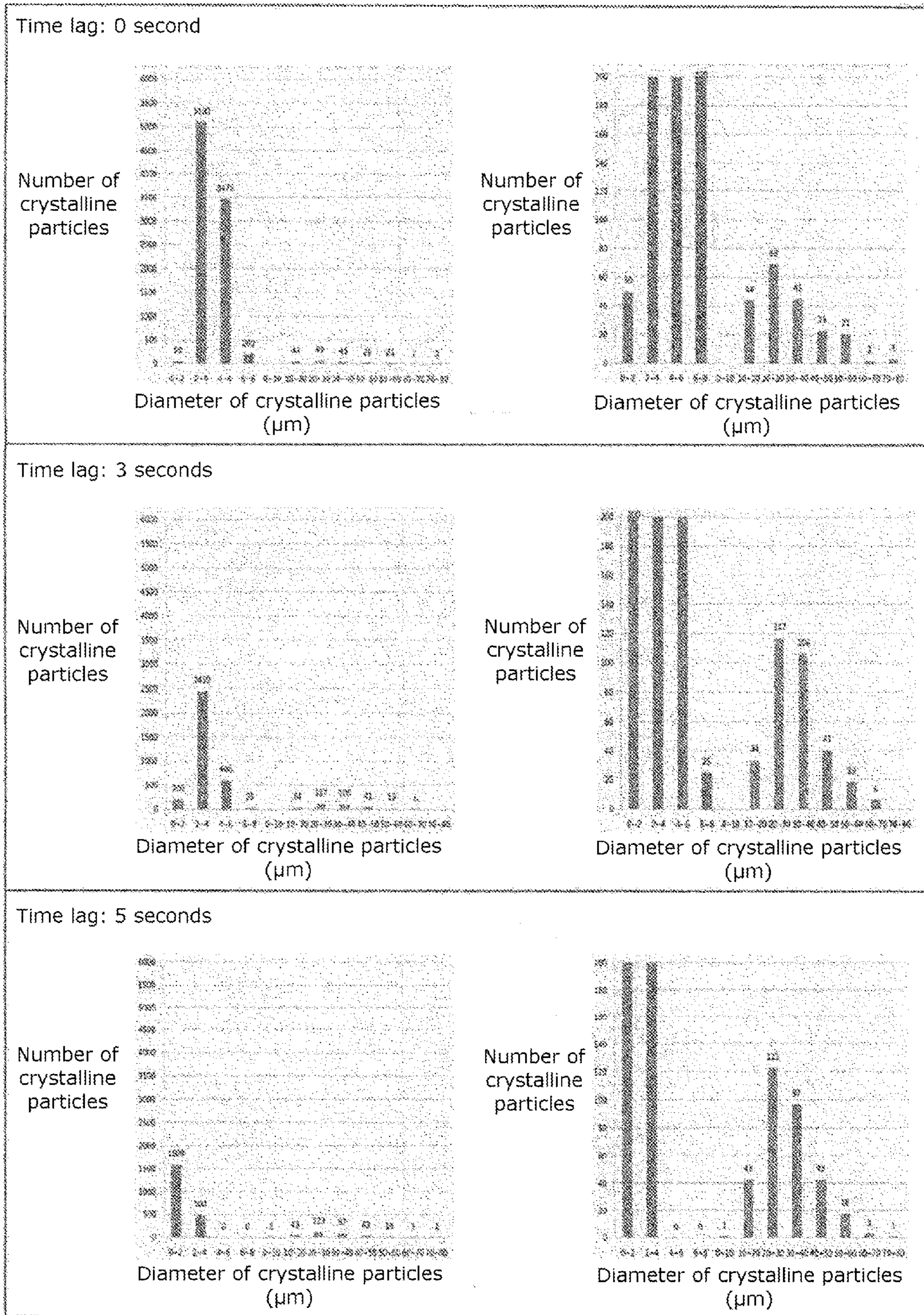
Relation between Injection Time Lag and Crystalline Particle Size (sleeve filling factor: 25 %)
