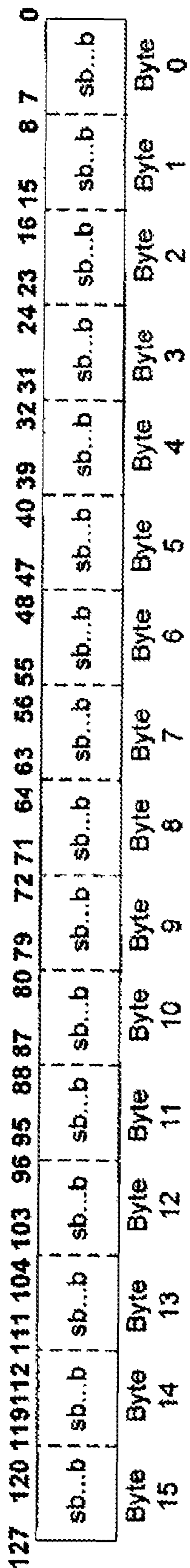
Signed packed byte in-register representation 511
