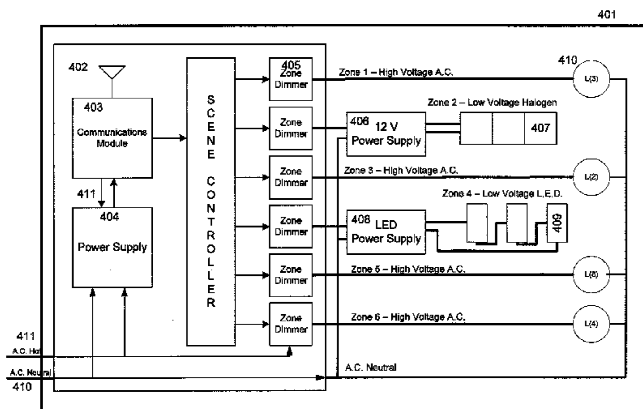
Master Dimmer Controller - Generic Wiring Example
