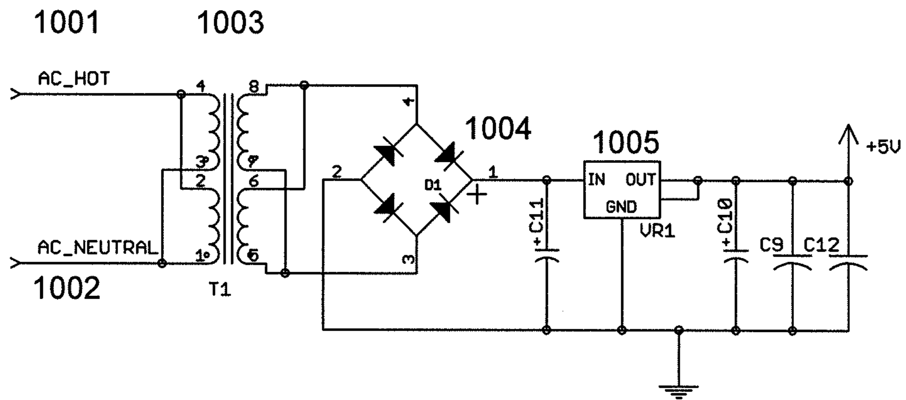
KEYPAD POWER SUPPLY
