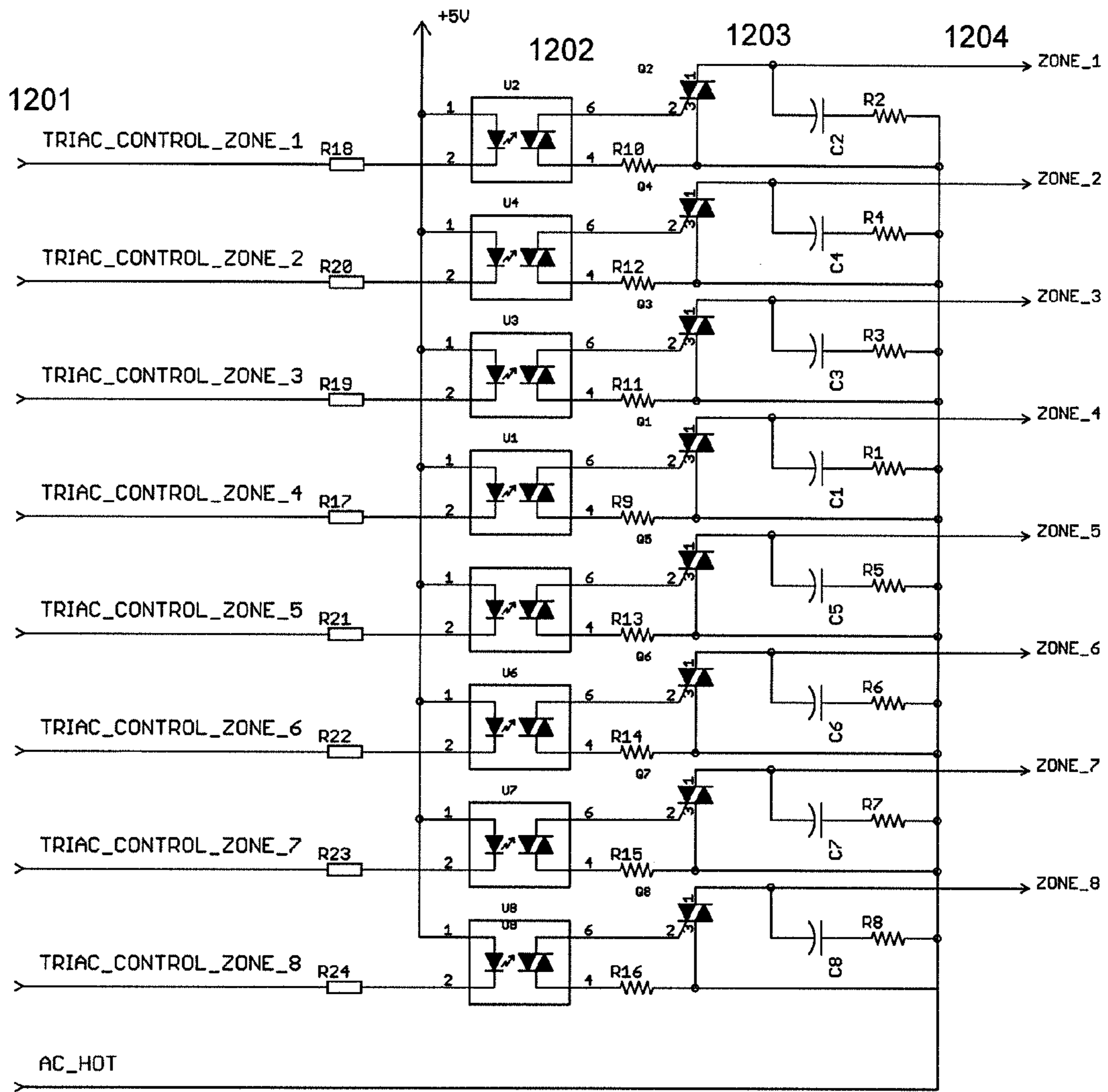
MASTER DIMMING CONTROLLER ZONE DIMMER CIRCUITS
