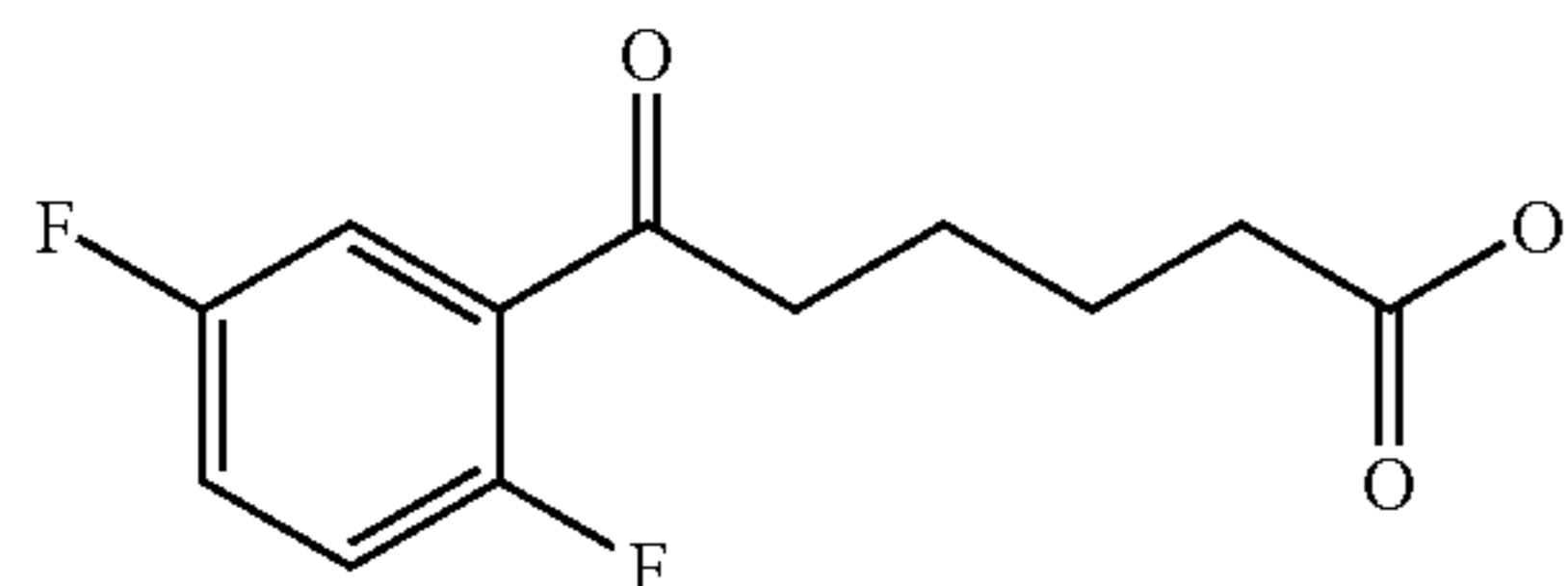
6-(2,5-Difluoro-phenyl)-6-oxo-hexanoic acid
