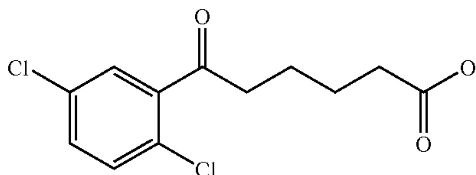
6-(2,5-Dichloro-phenyl)-6-oxo-hexanoic acid
