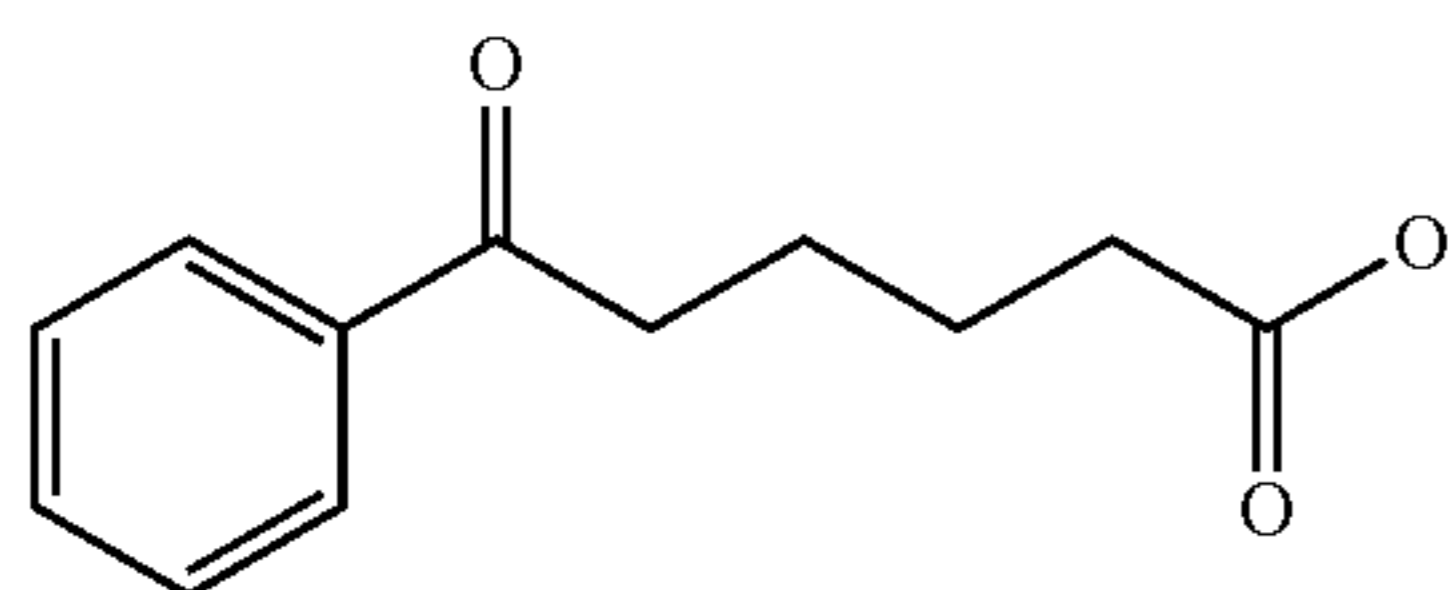
6-Oxo-6-phenyl-hexanoic acid
