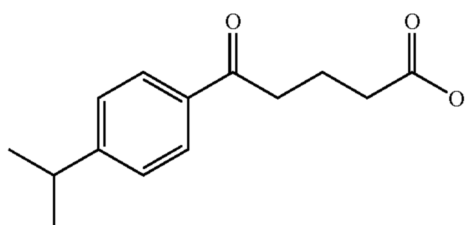
5-(4-Isopropyl-phenyl)-5-oxo-pentanoic acid
