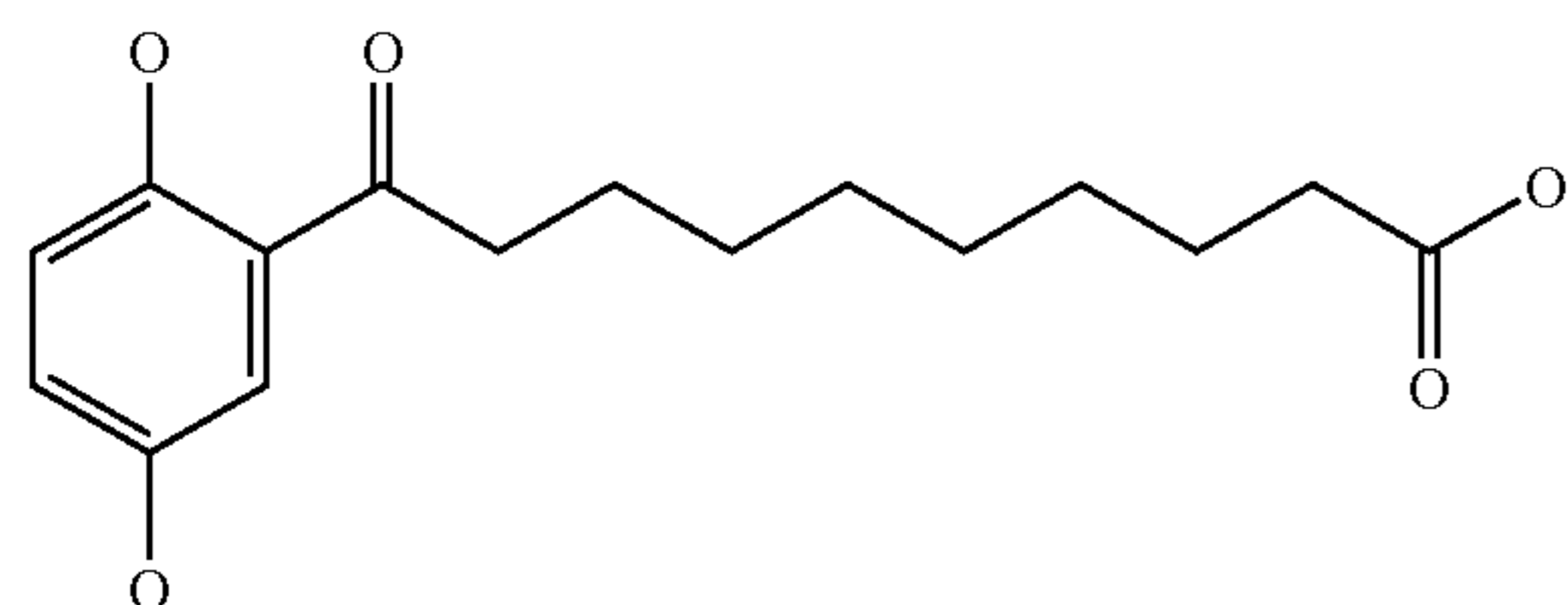
10-(2,5-Dihydroxy-phenyl)-10-oxo-decanoic acid
