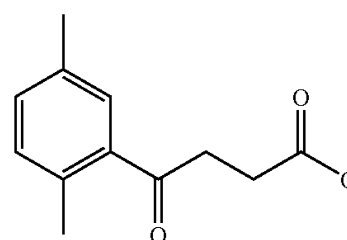
4-(2,5-Dimethyl-phenyl)-4-oxo-butyrac acid
