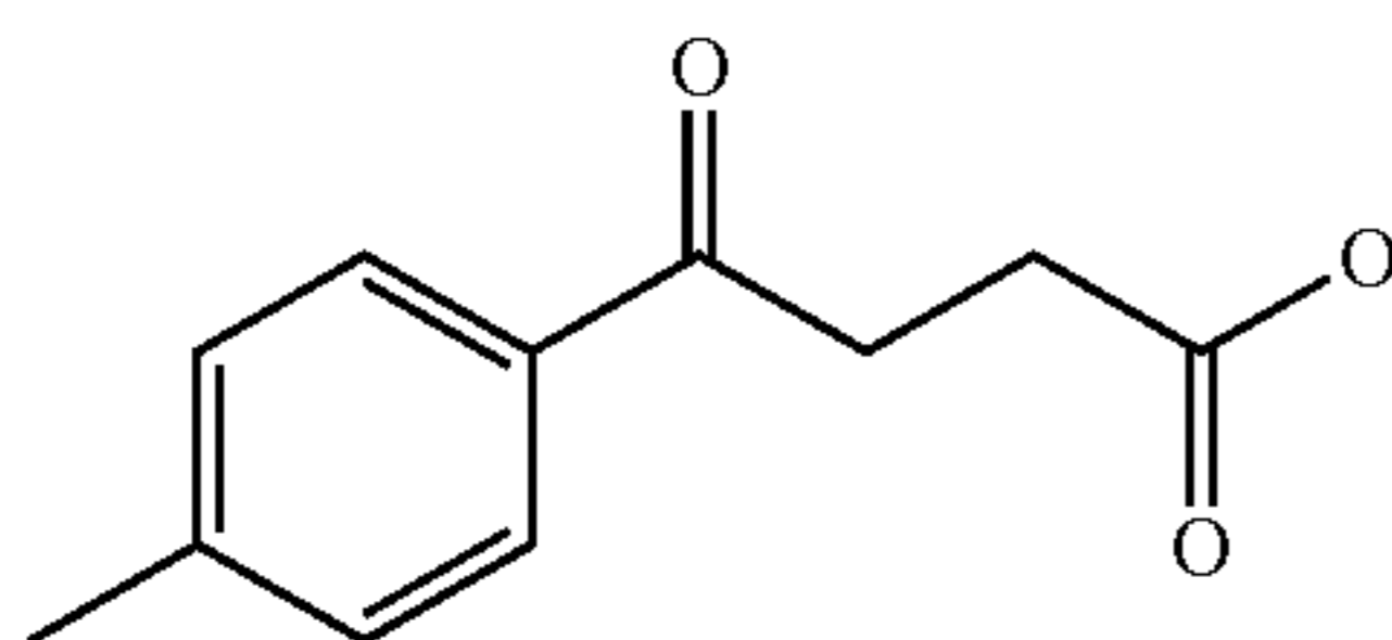
4-Oxo-4-p-tolyl-butanoic acid
