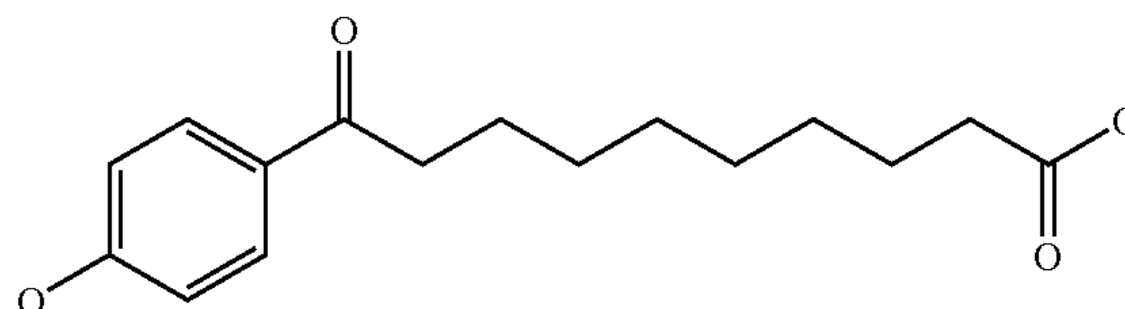
10-(4-hydroxyphenyl)-10-oxodecanoic acid
