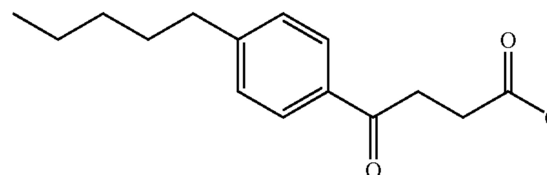
4-Oxo-4-(4-pentyl-phenyl)-butyric acid
