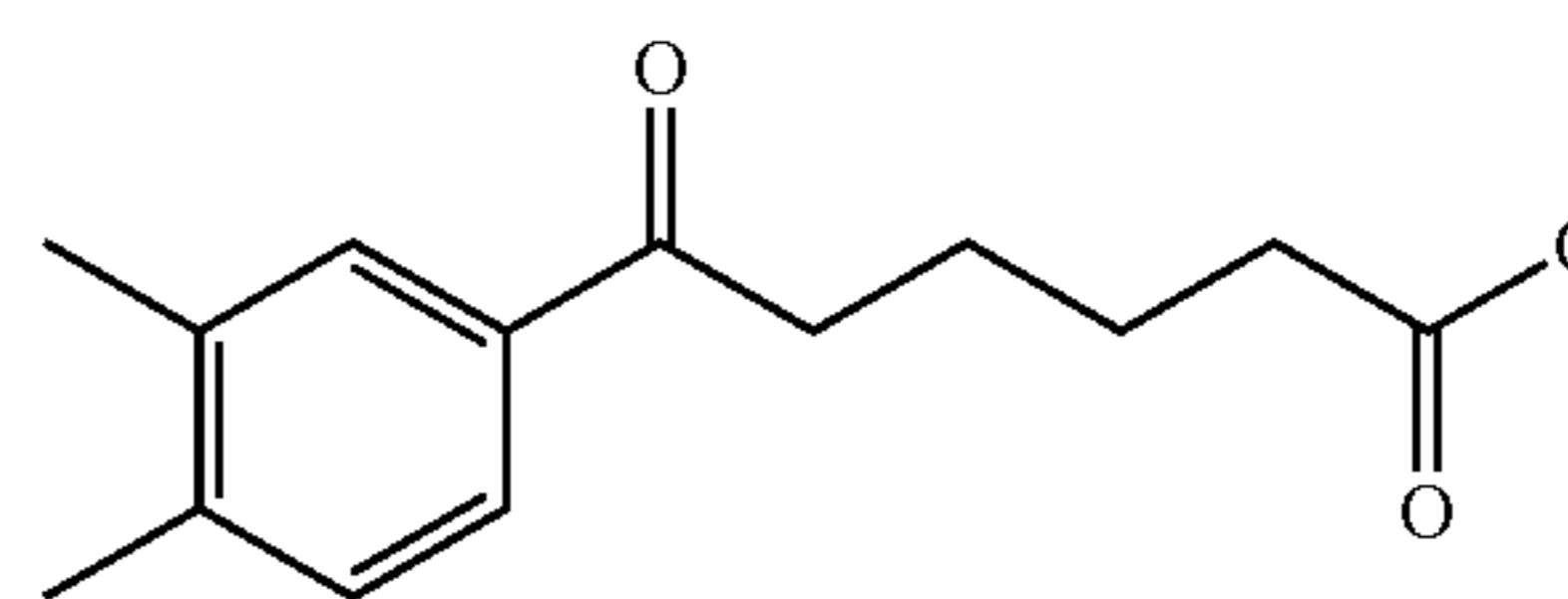
6-(3,4-Dimethyl-phenyl)-6-oxo-hexanoic acid
