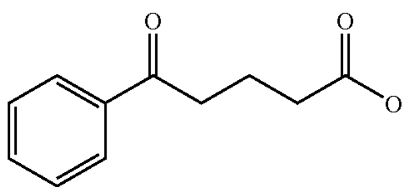
5-Oxo-5-phenyl-pentanoic acid
