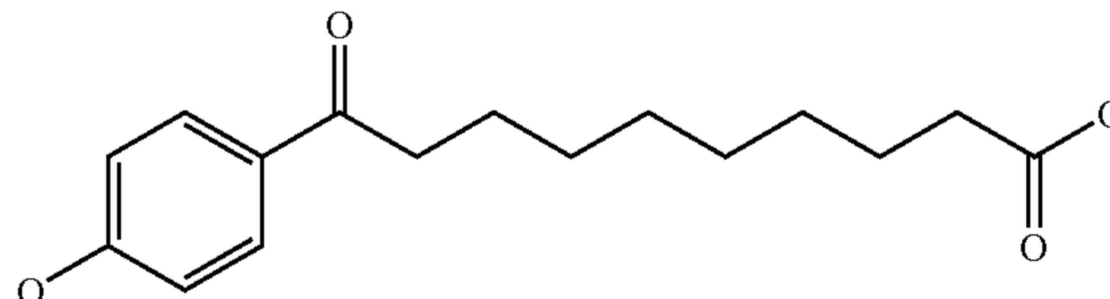
10-(4-hydroxyphenyl)-10-oxodecanoic acid
