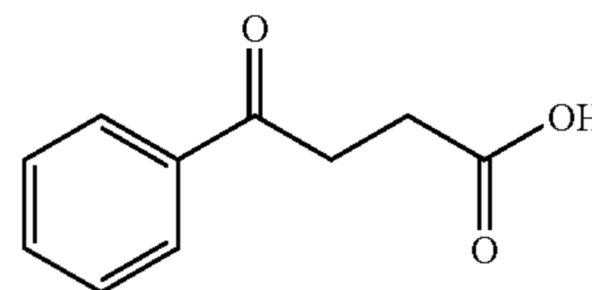
4-Oxo-4-phenyl-butyric acid
