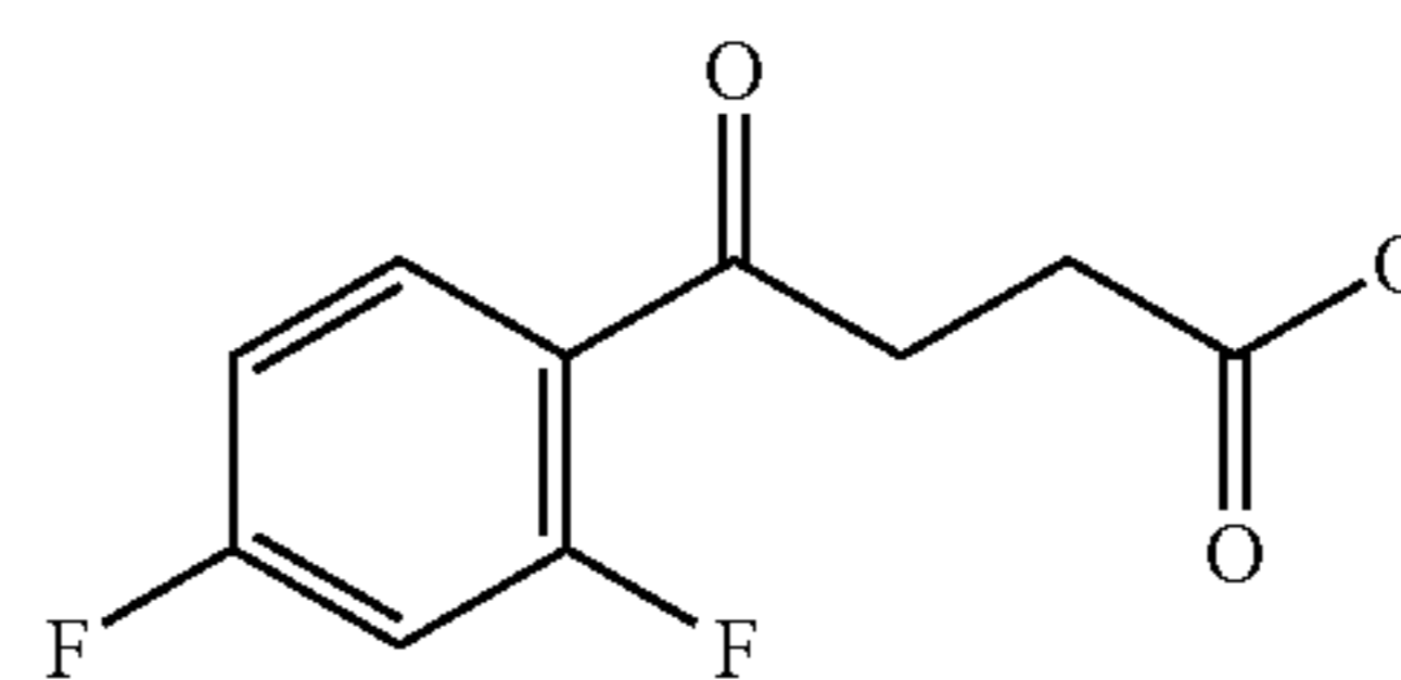
4-(2,4-Difluoro-phenyl)-4-oxo-butyric acid
