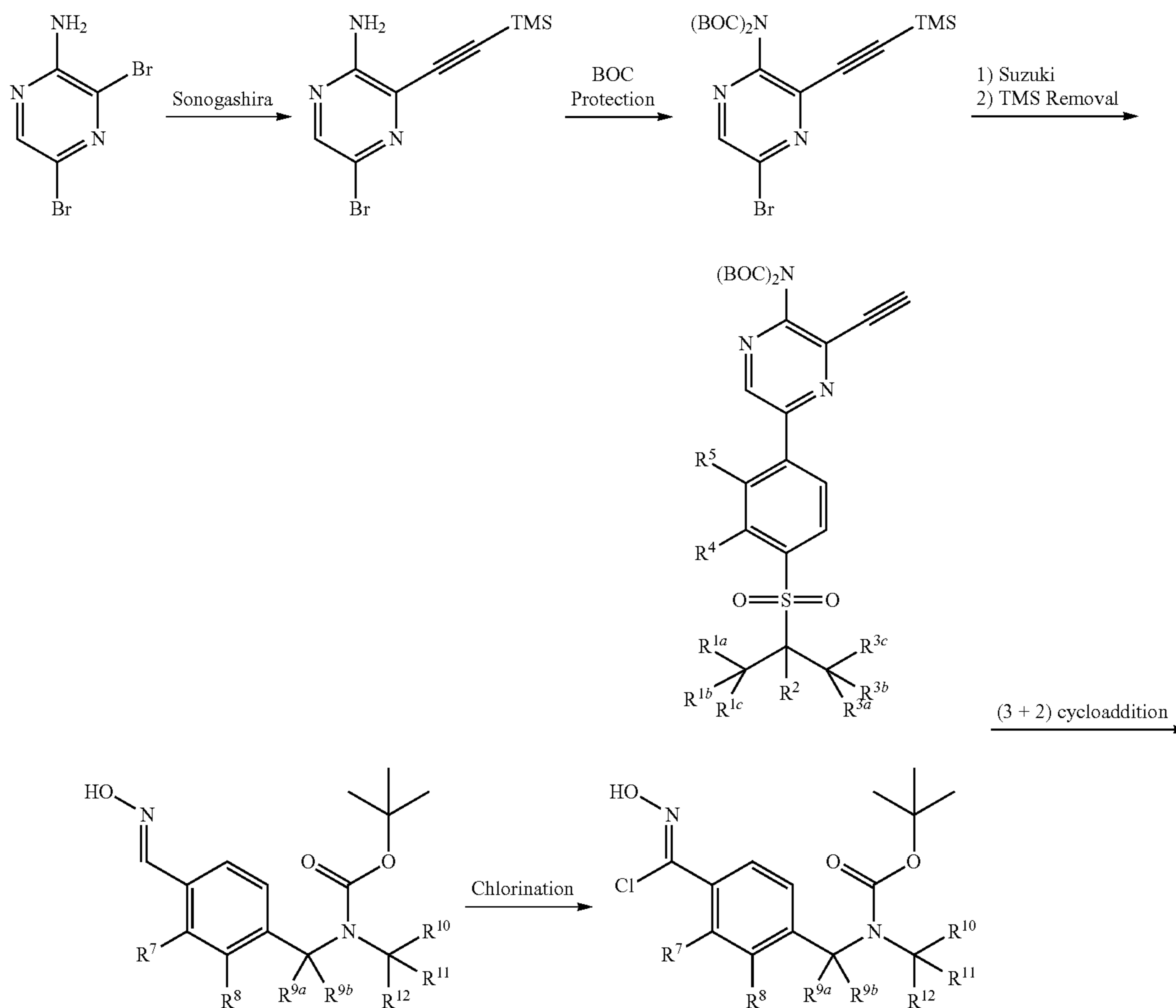
SCHEME P: Formation of isoxazole derivatives
