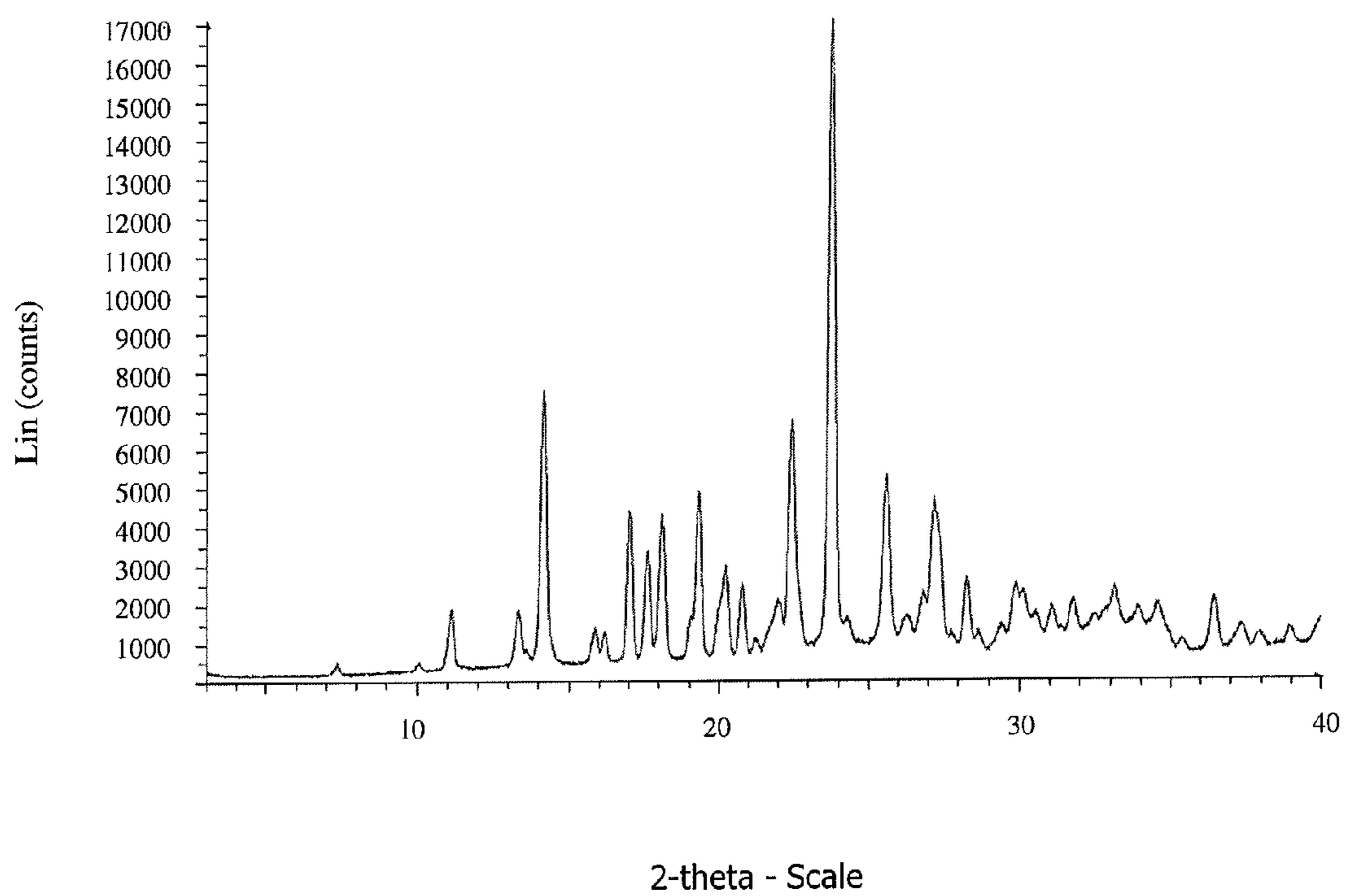
FIGURE 1a: XRPD Compound I-2 free base
