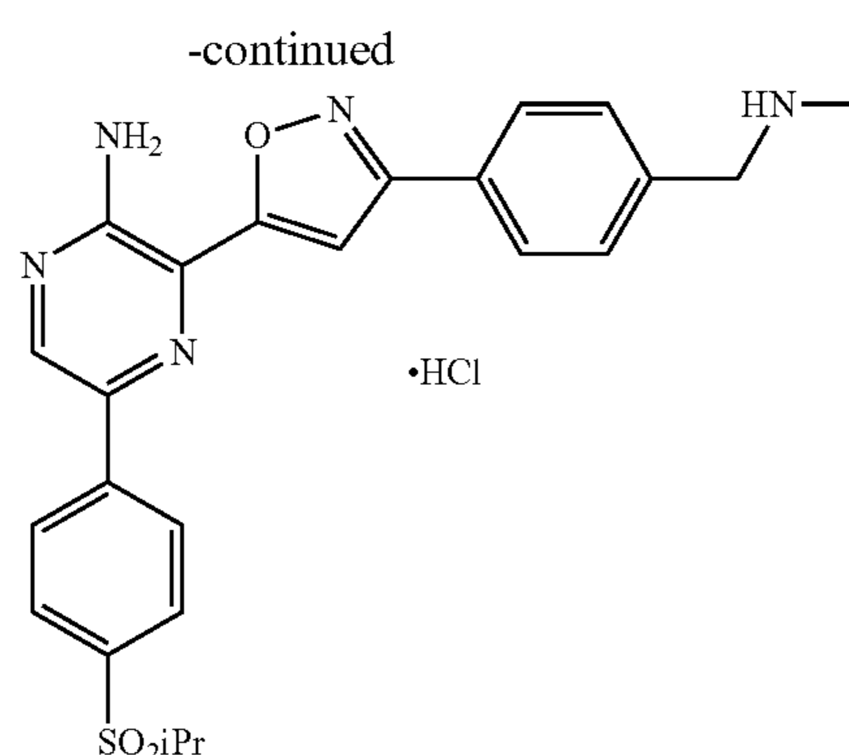
Compound I-2.HCl
