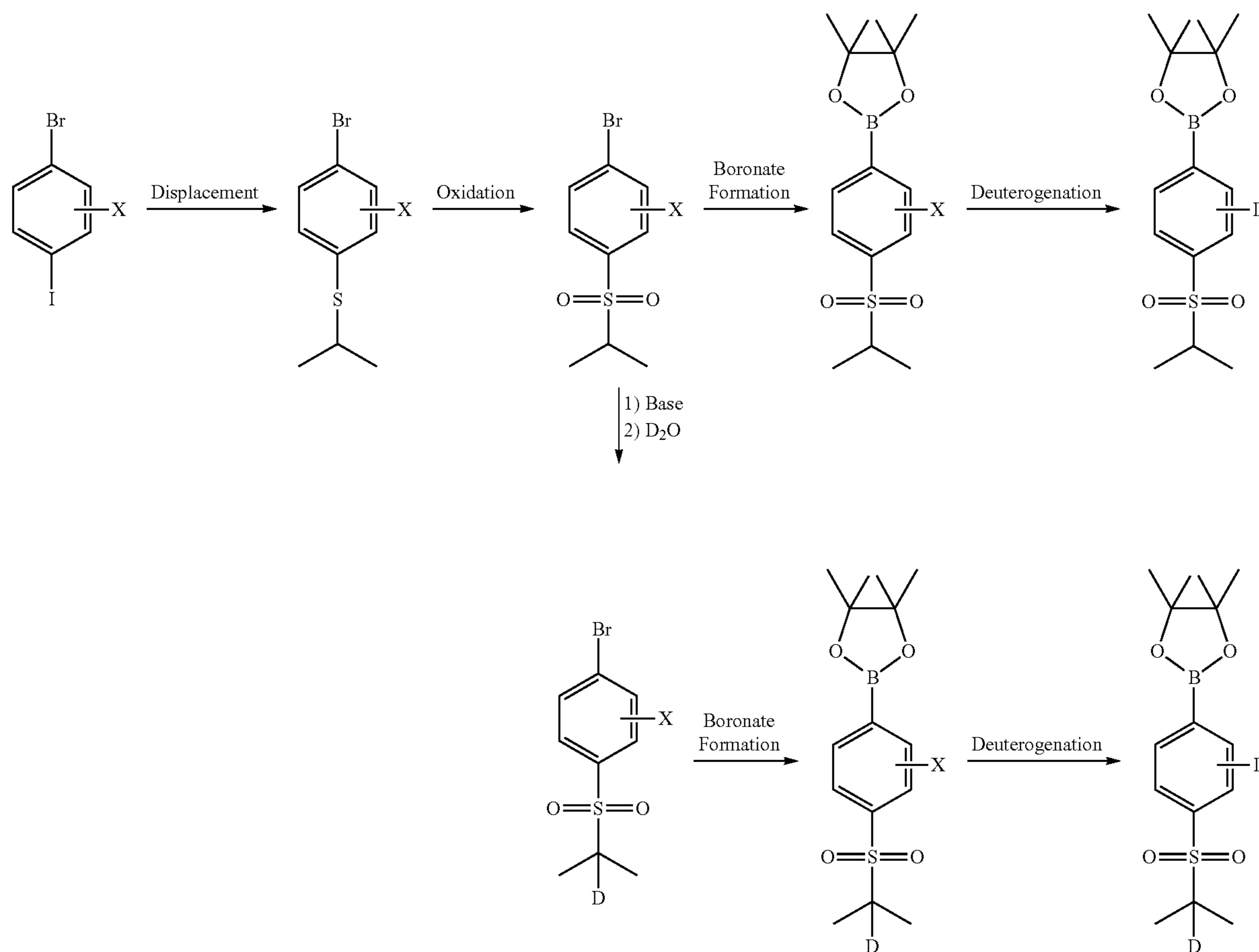
SCHEME E: Formation of aryl ring deuterated boronate
