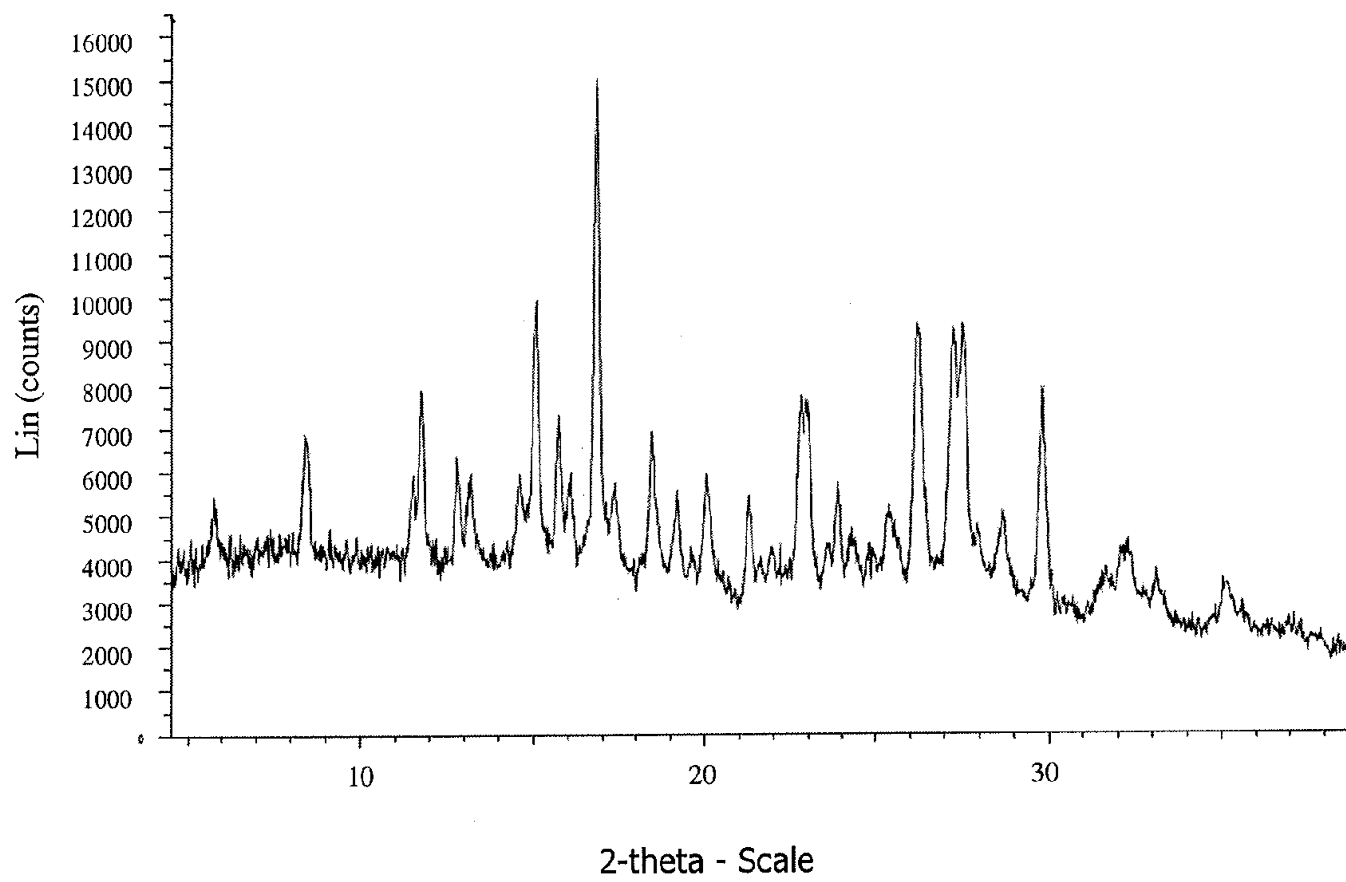
FIGURE 1c: XRPD Compound I-2 • 2HCl
