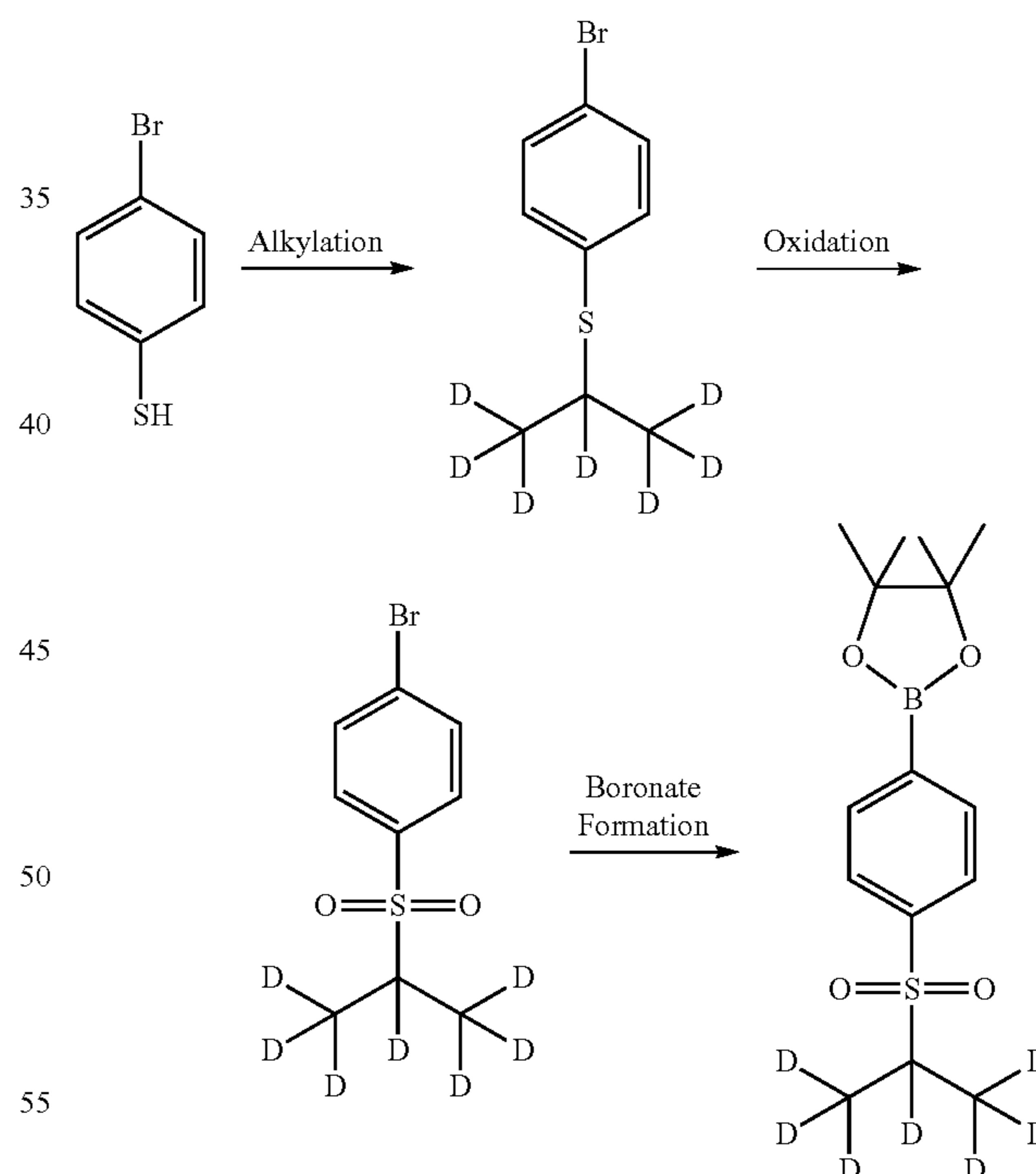
SCHEME D: Formation of d7-boronate
