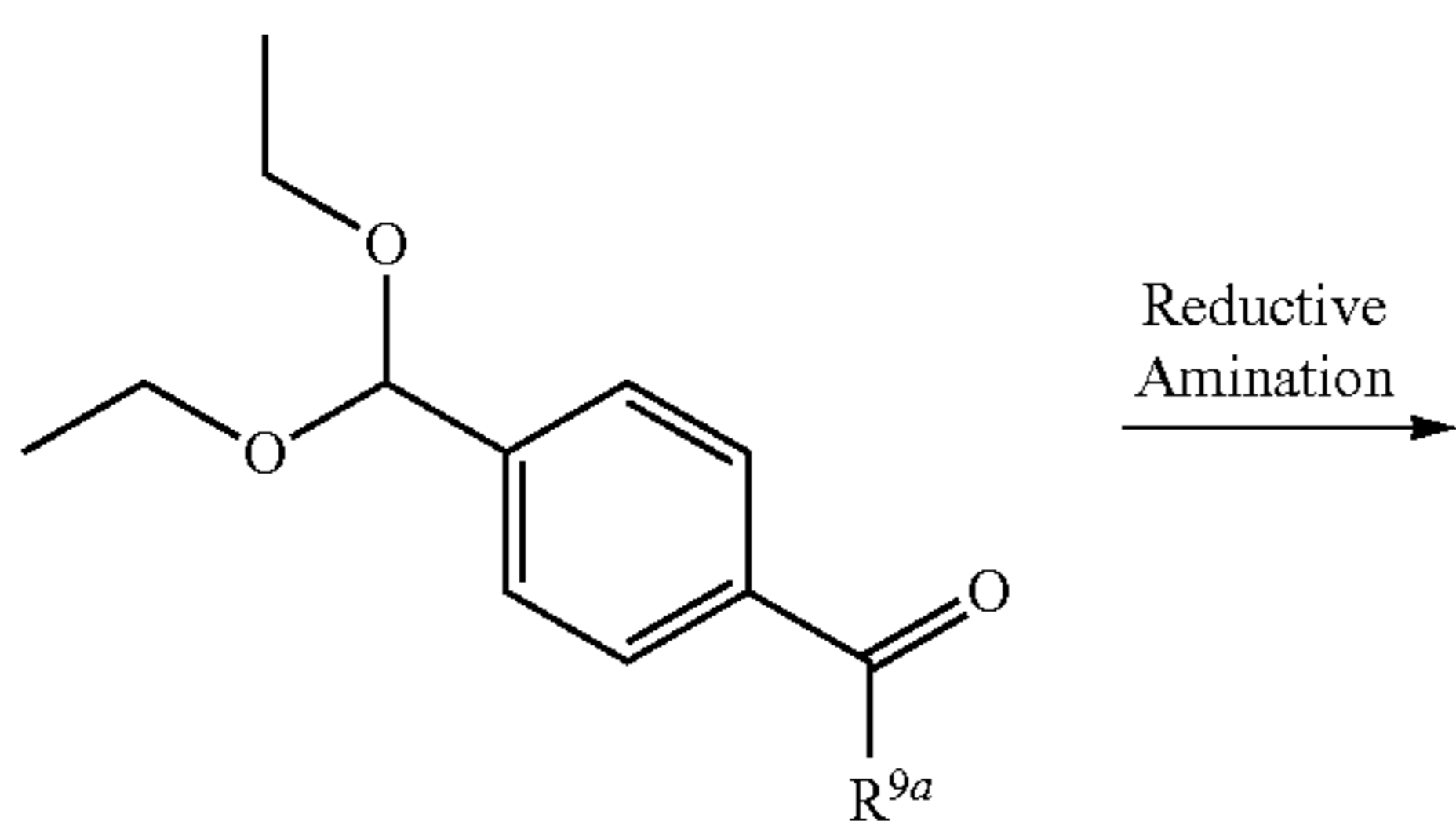
SCHEME L: Formation of deuterated oxime intermediates
