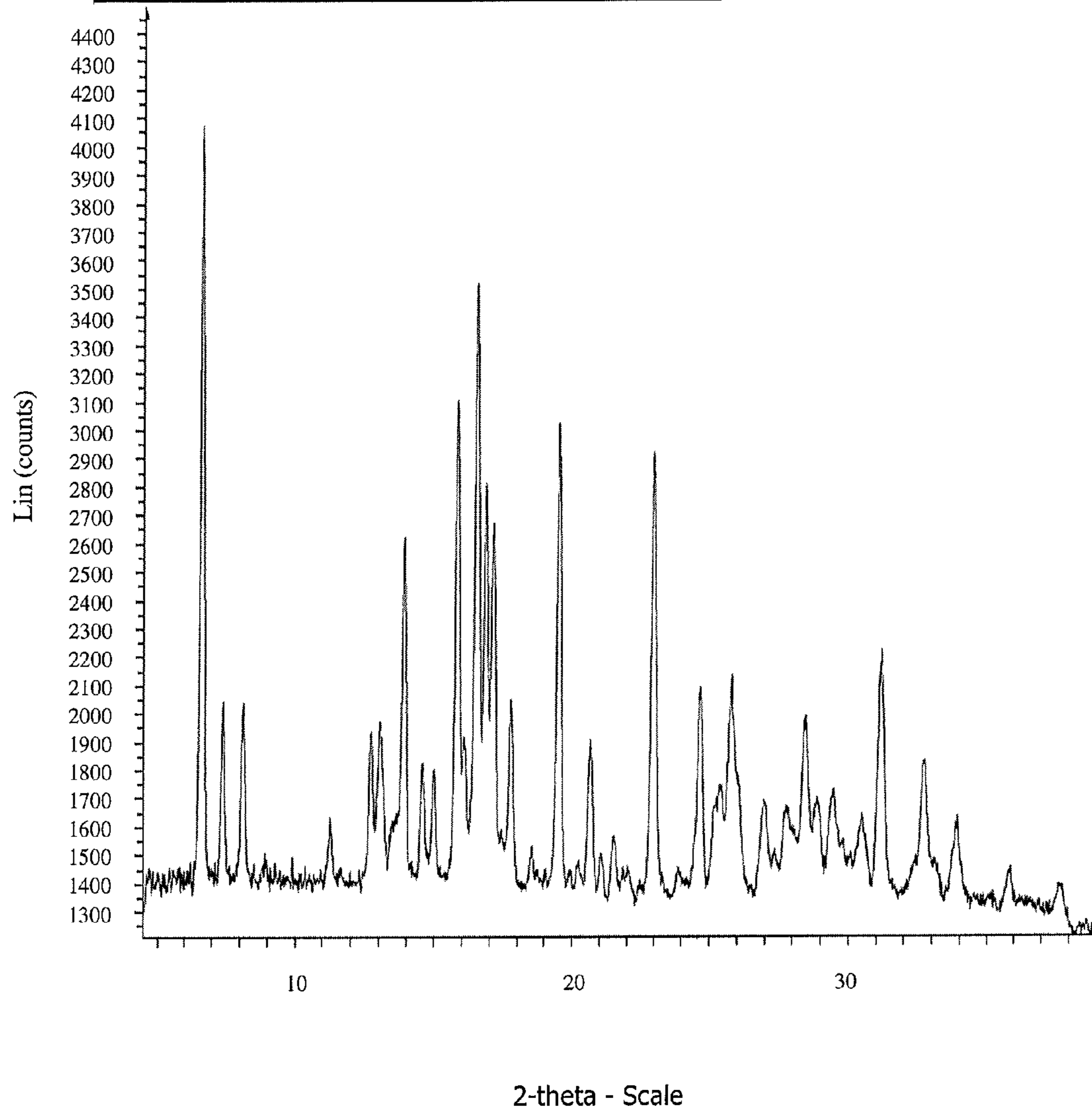
FIGURE 1d: XRPD Compound I-2 • HCl monohydrate
