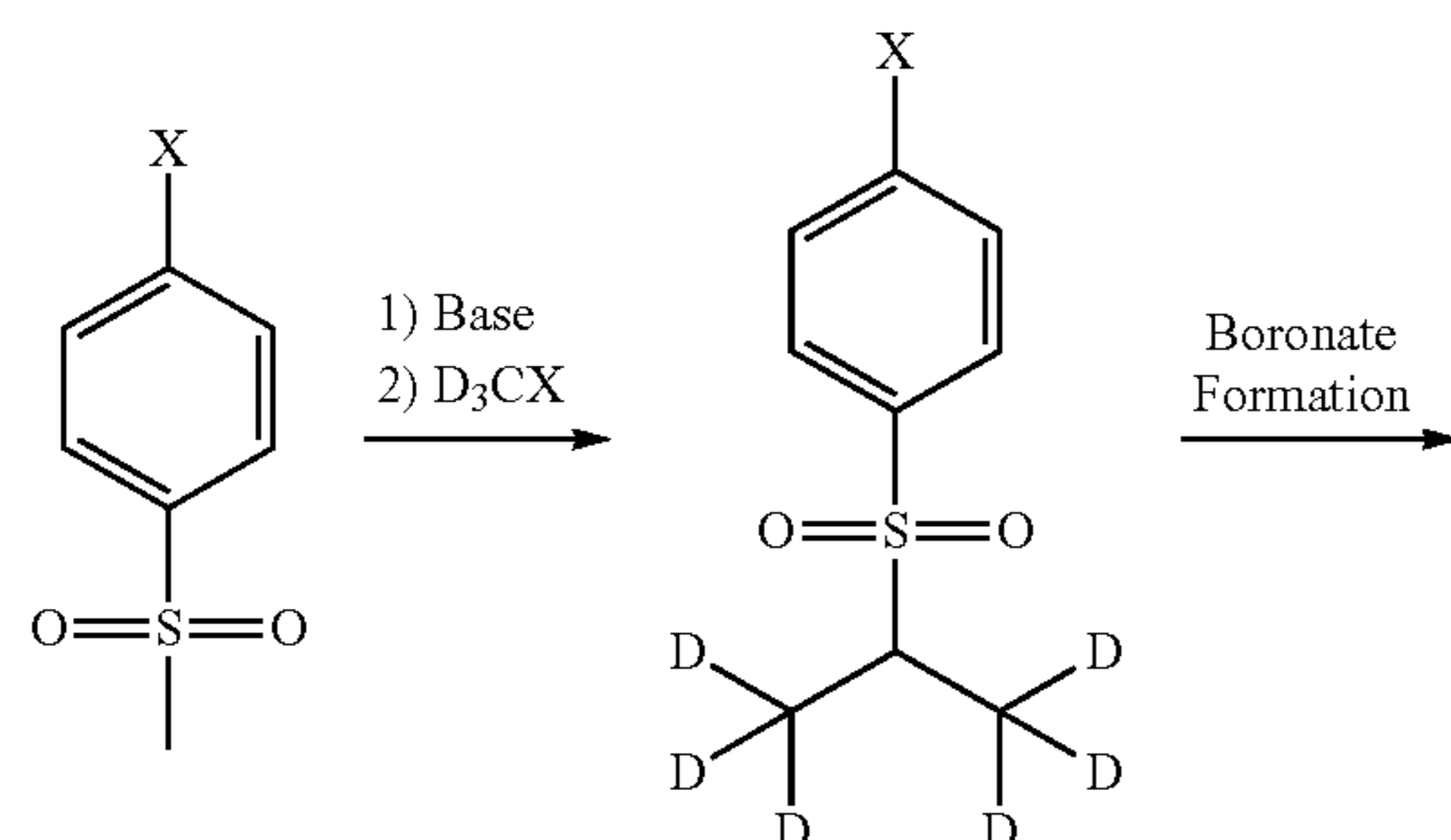
SCHEME C: Formation of d6-boronate
