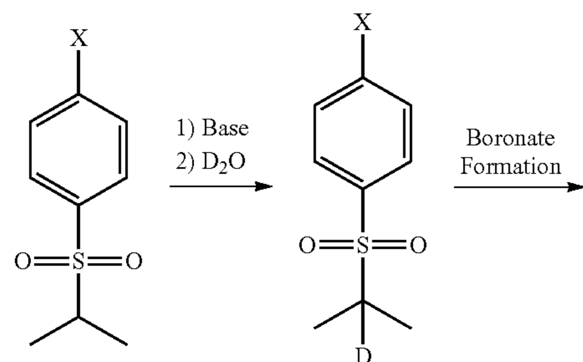
SCHEME B: Formation of d1-boronate
