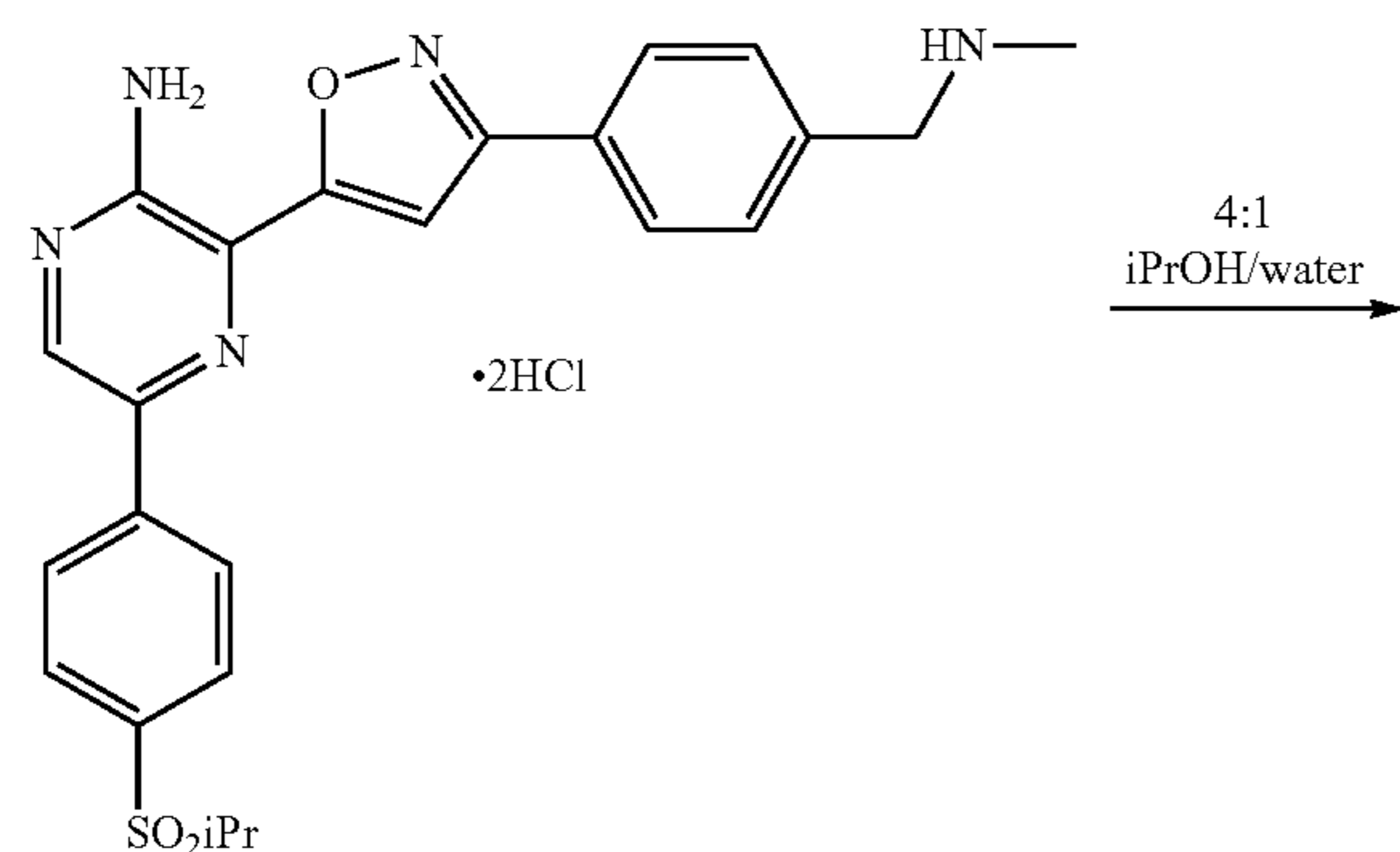
Compound I-2.HCl
