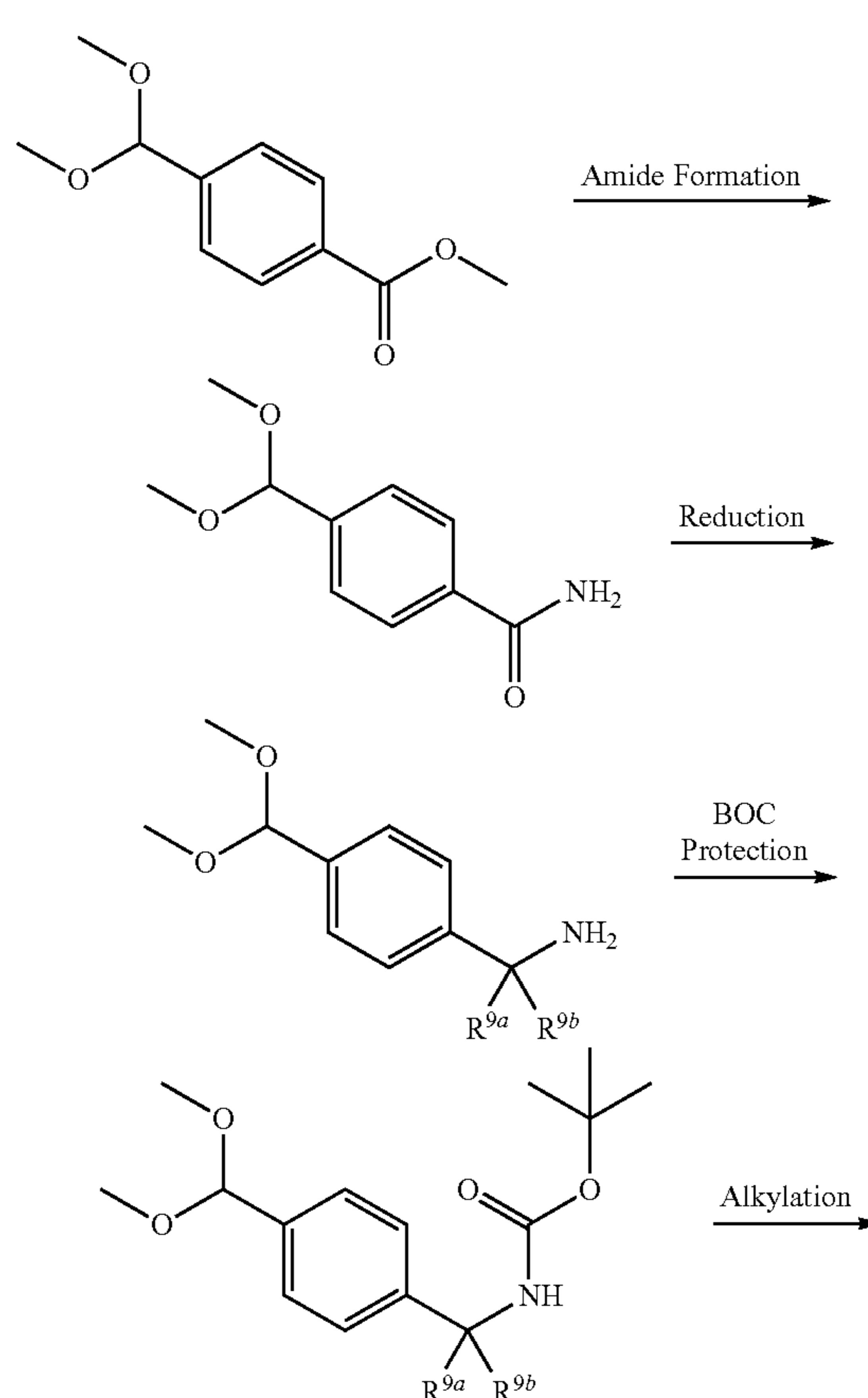
SCHEME M: Formation of deuterated oxime intermediates
