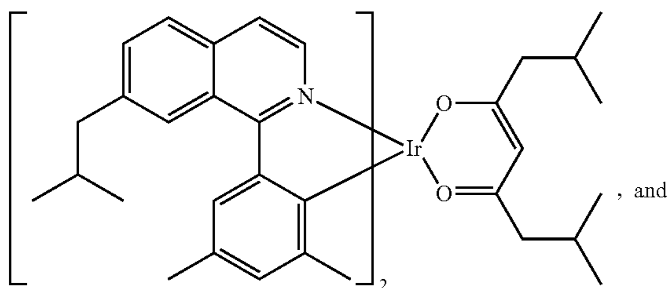
Compound 6
