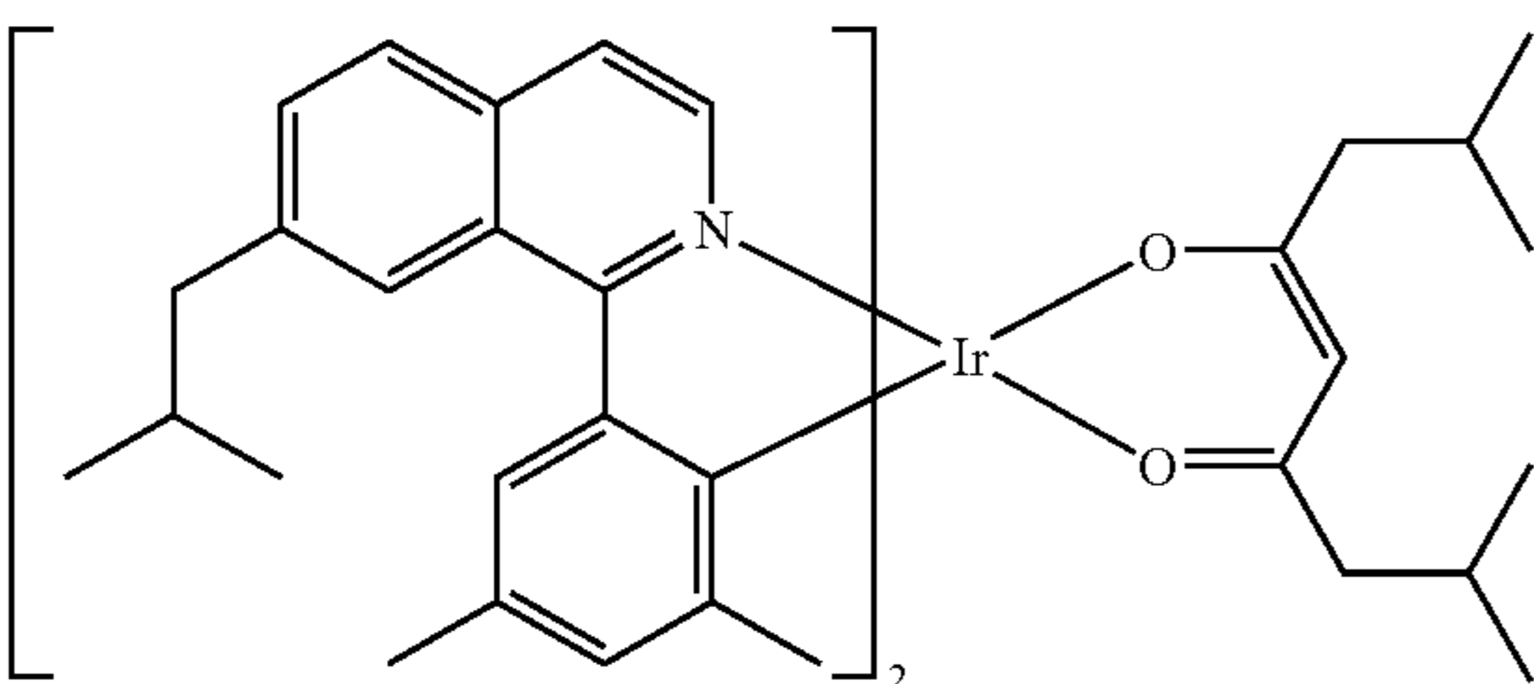
Compound 7
