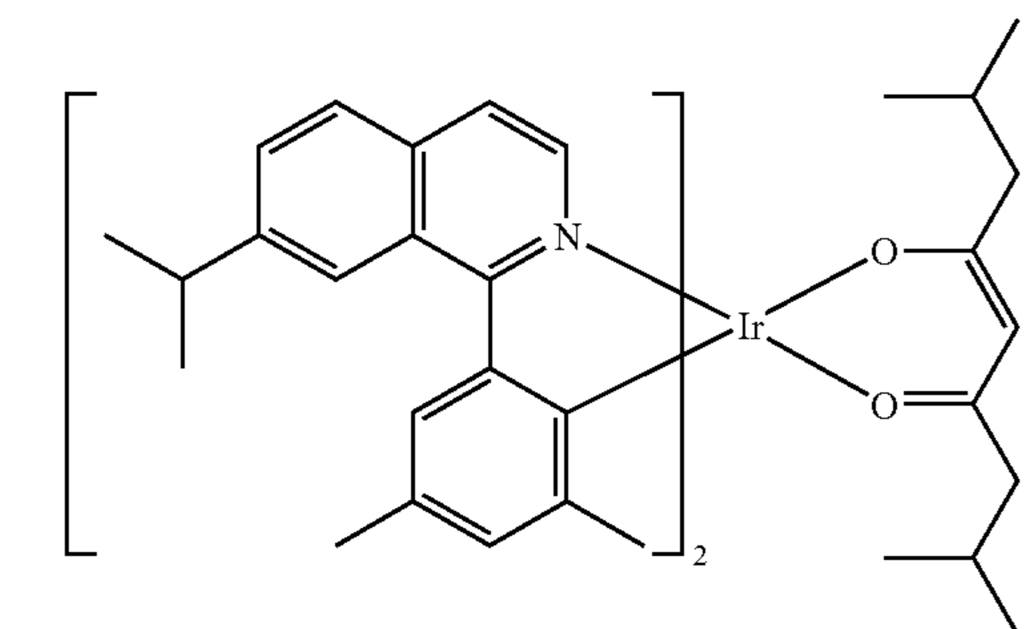
Compound 7
