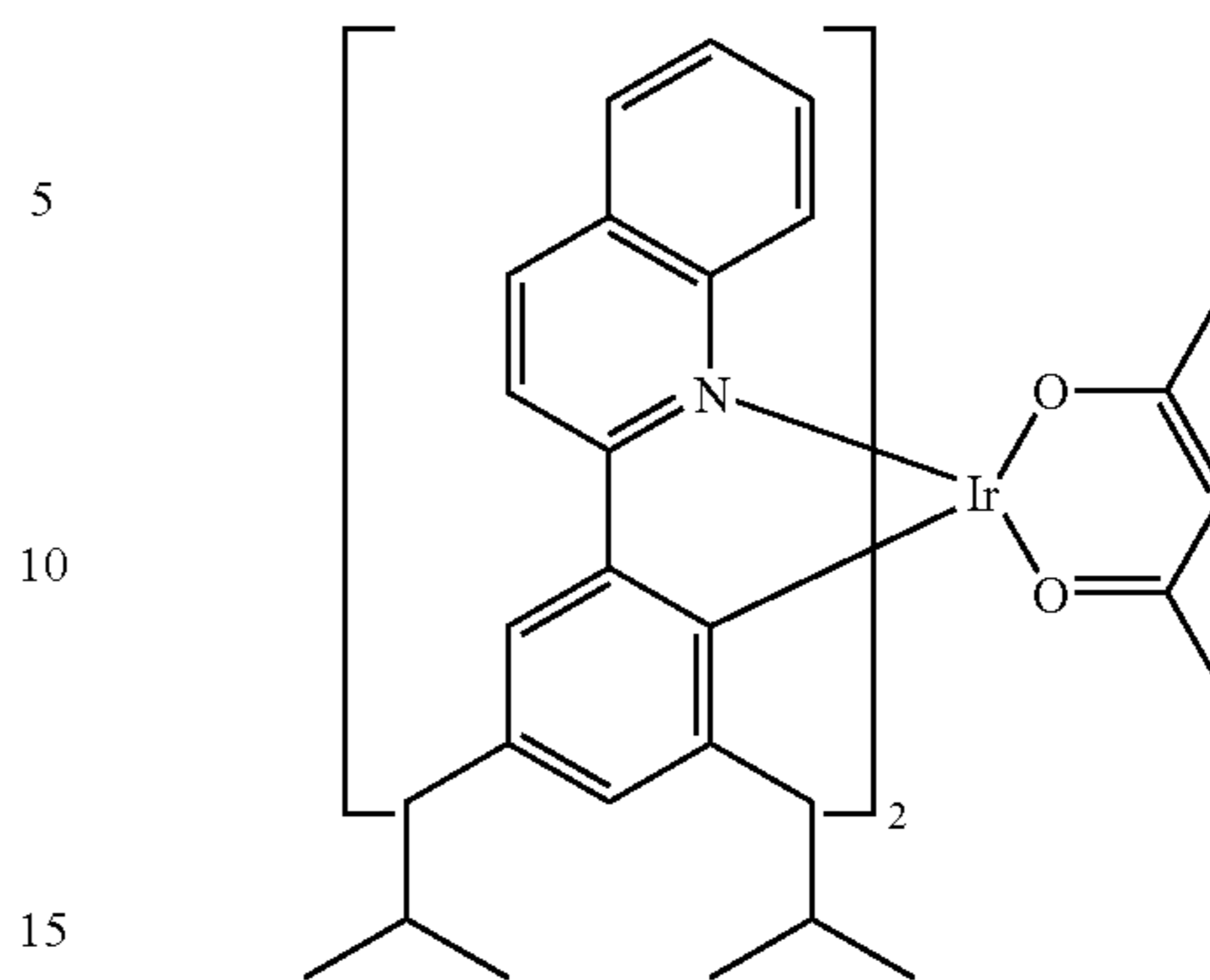
Compound 5
