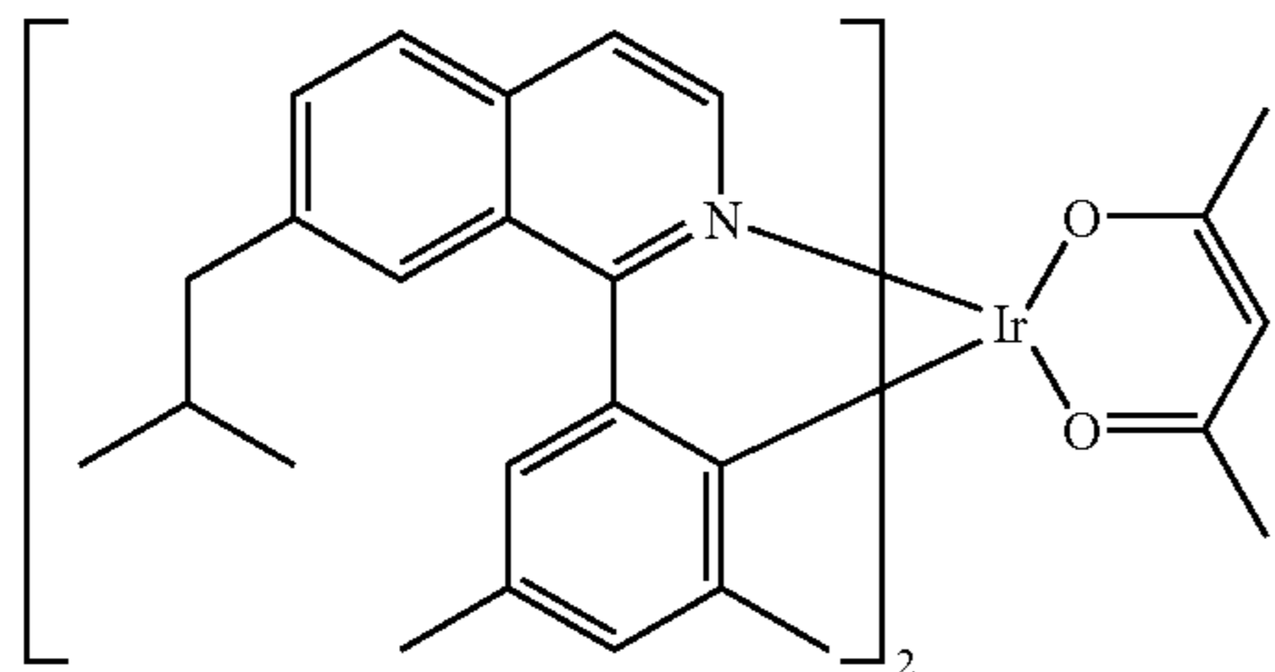
Compound 11
