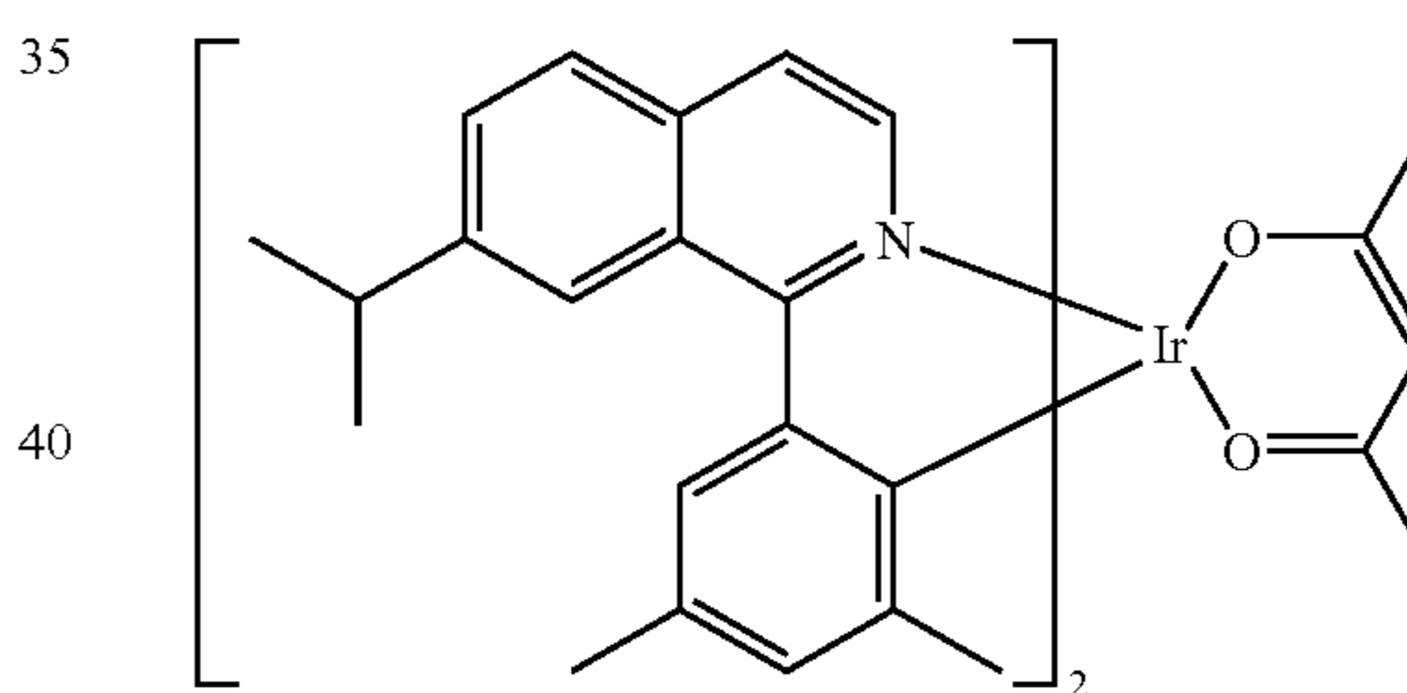
Compound 1
