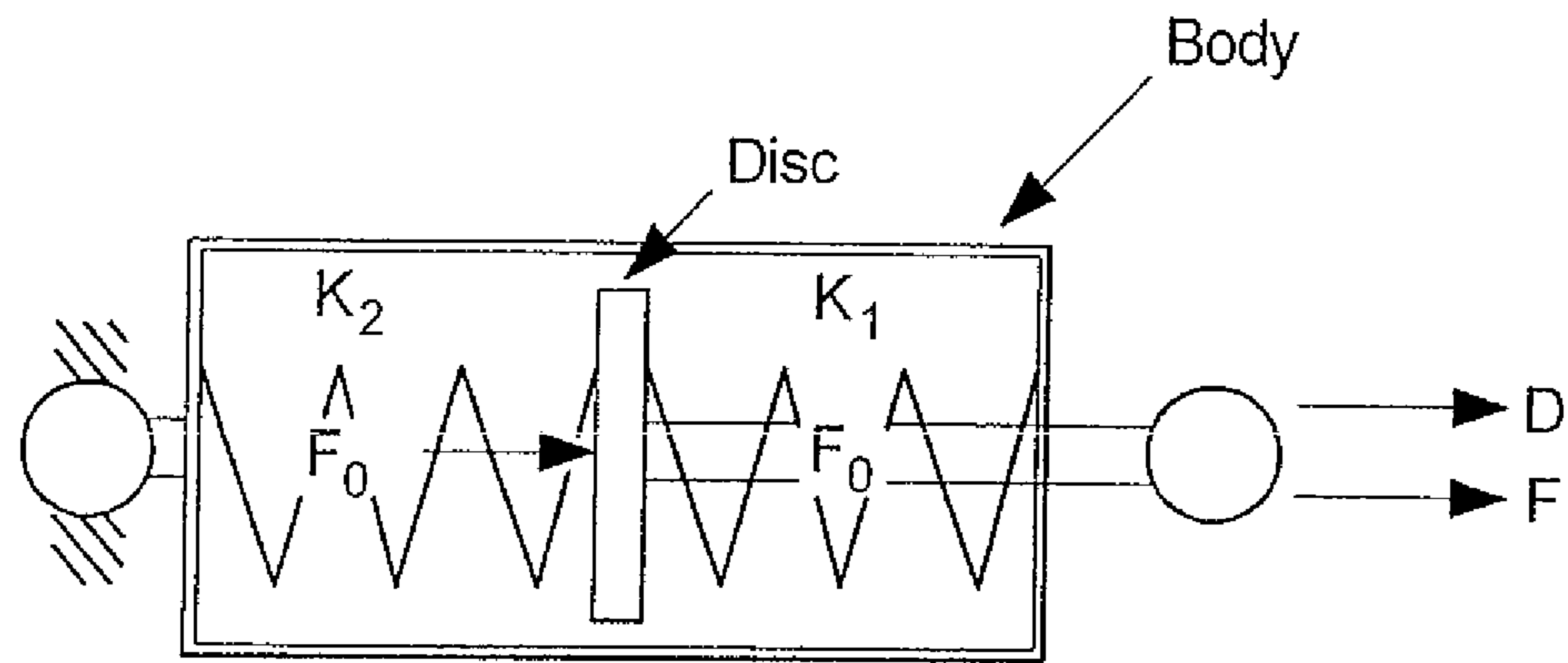
Free-body diagram
