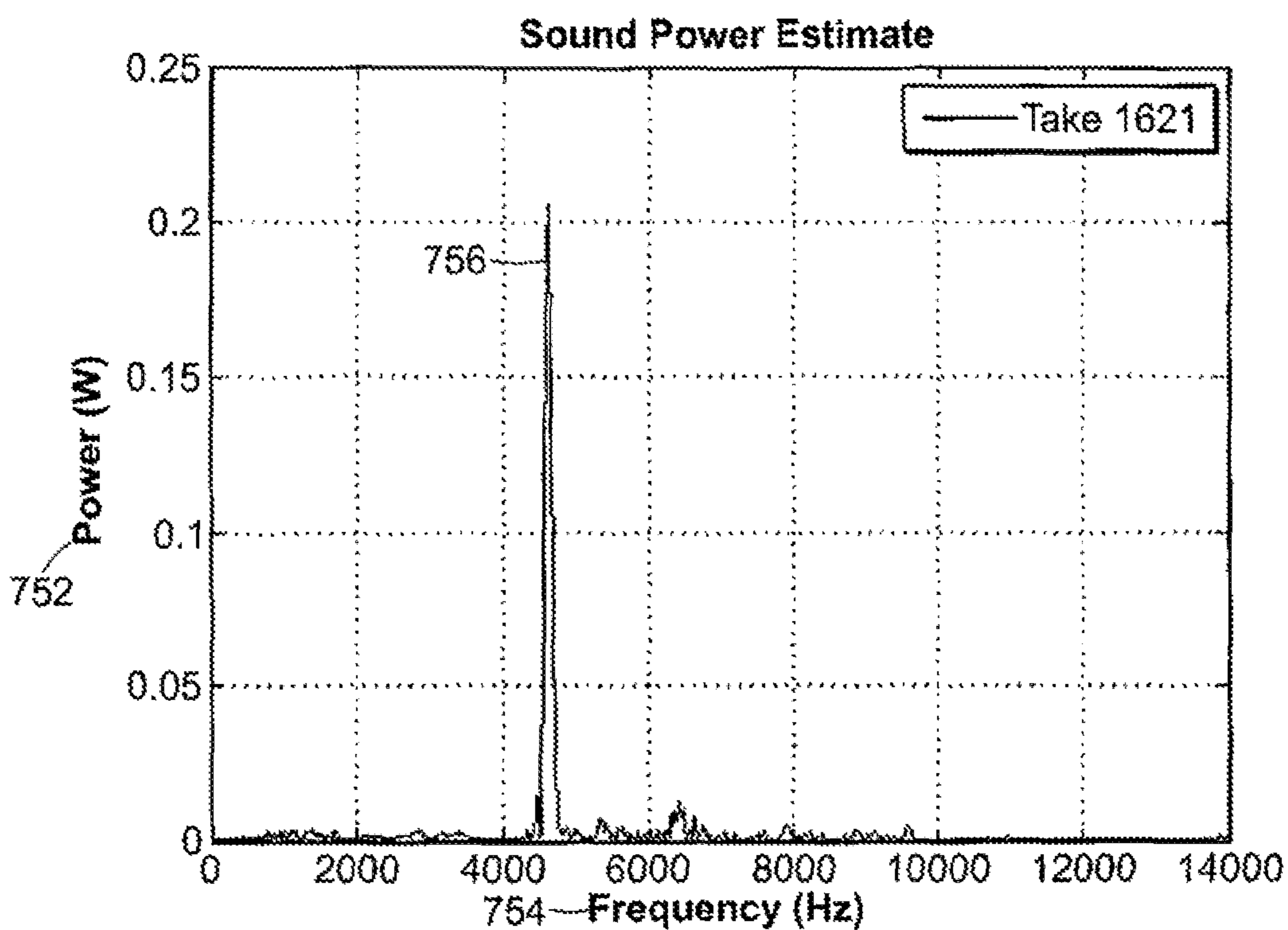
FIG. 7 (Prior Art)
