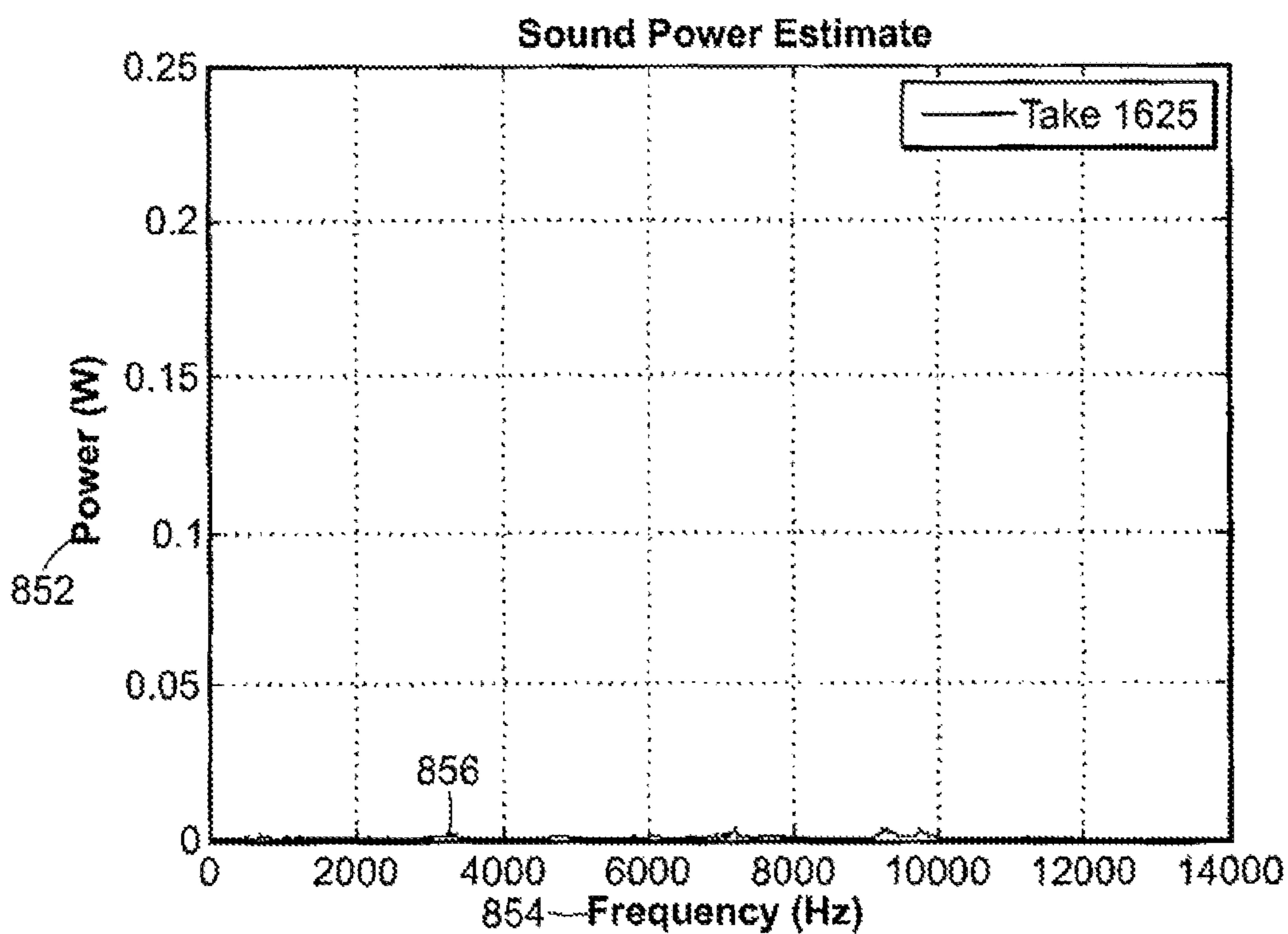
FIG. 8 (Prior Art)
