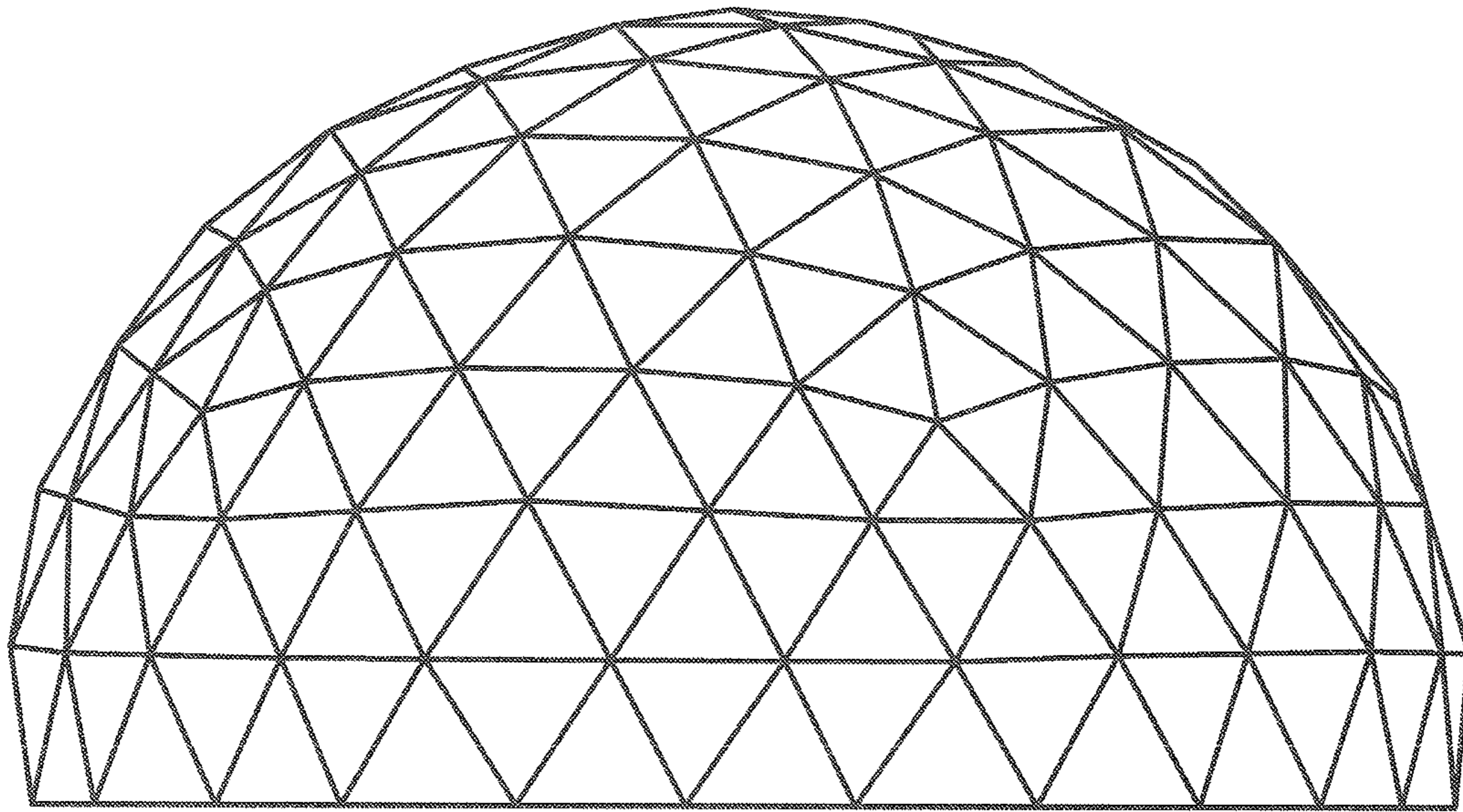
Geodesic 5V 8/15 Icosahedron Dome Pattern
