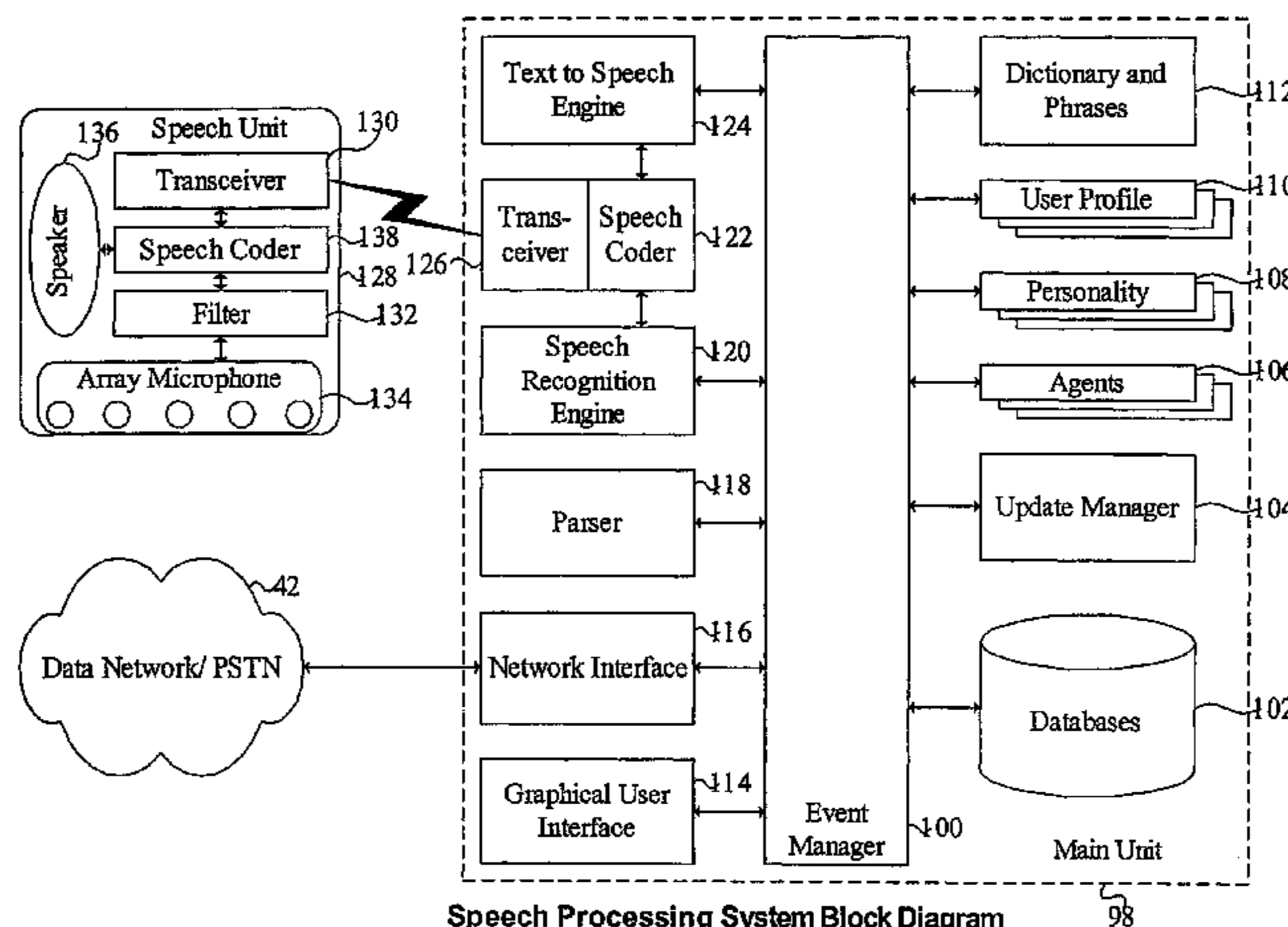
Speech Processing System Block Diagram 98
