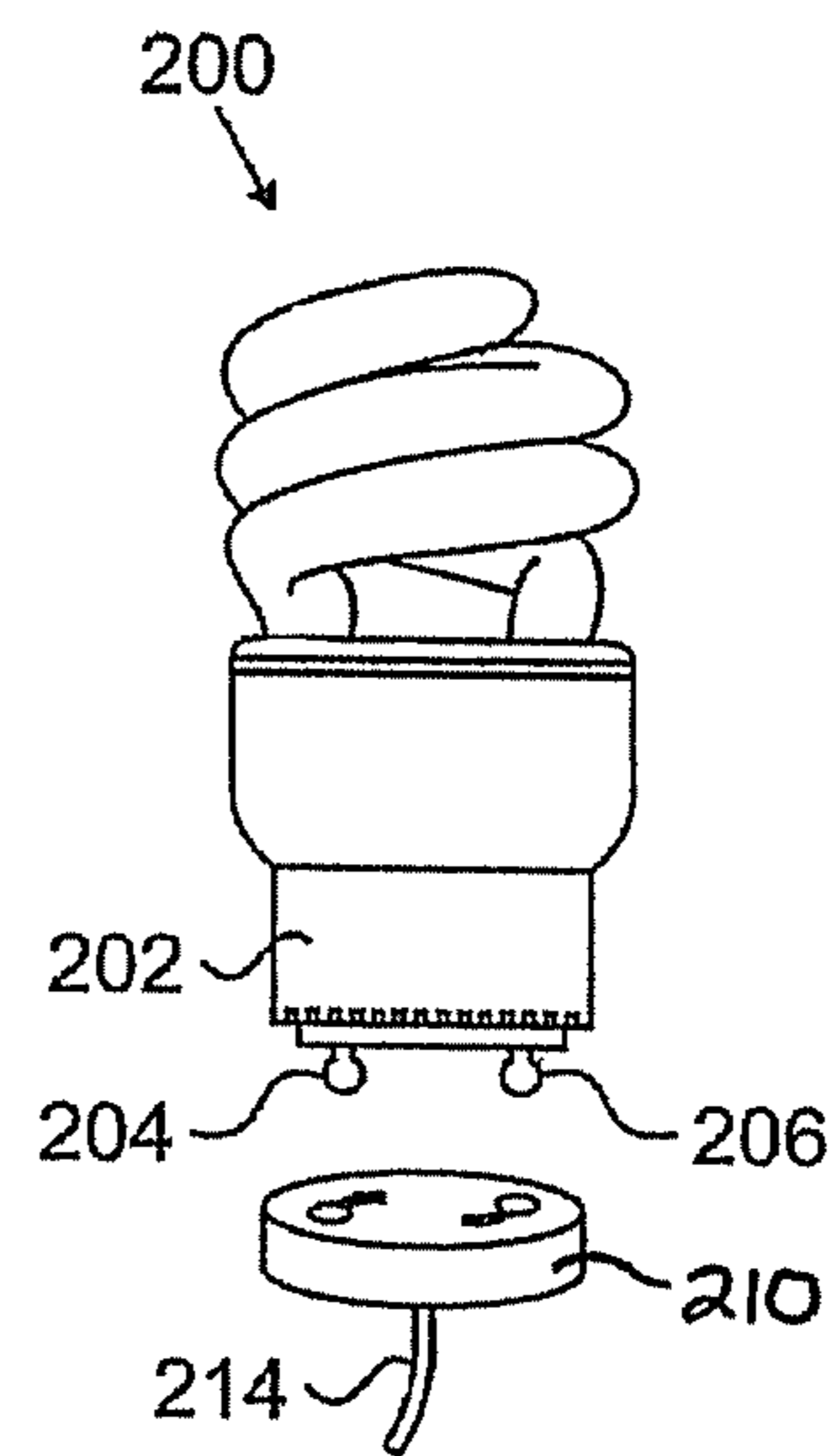
FIG. 2 (RELATED ART)
