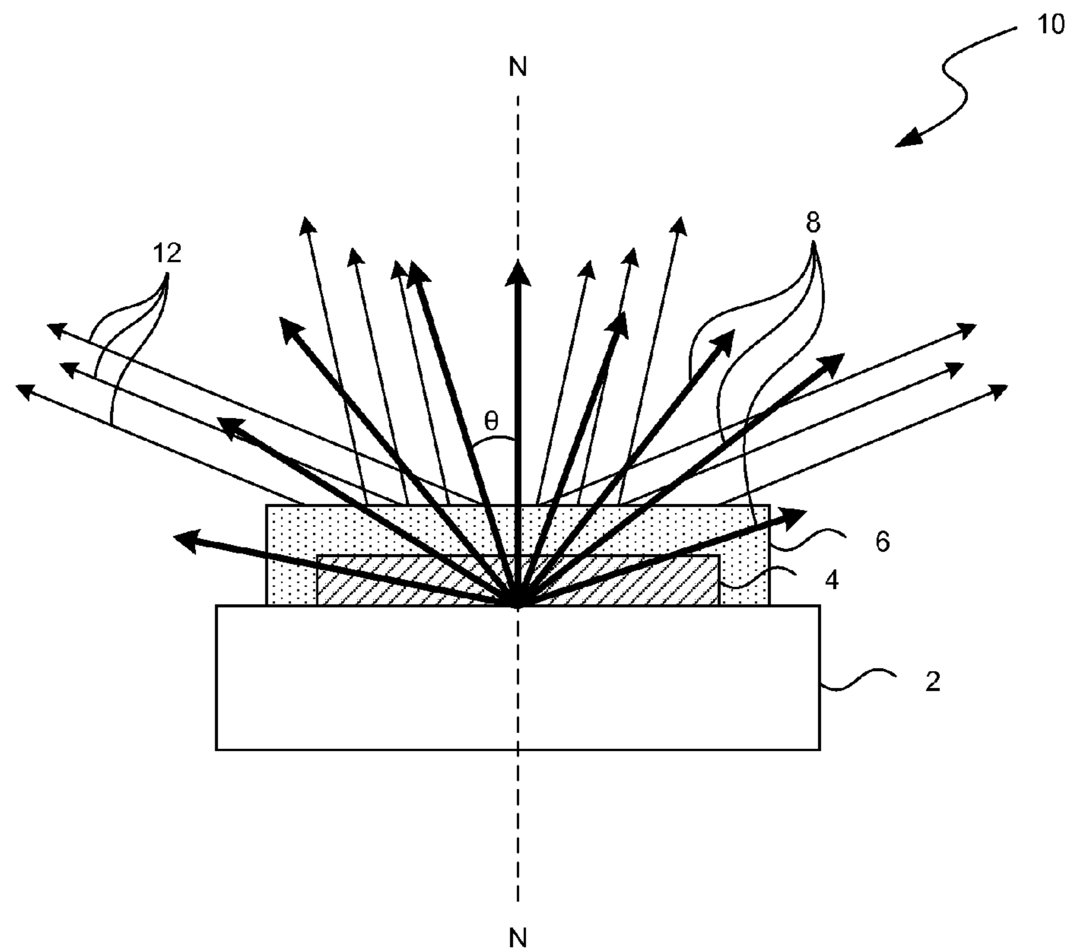
FIG. 1 (Prior Art)
