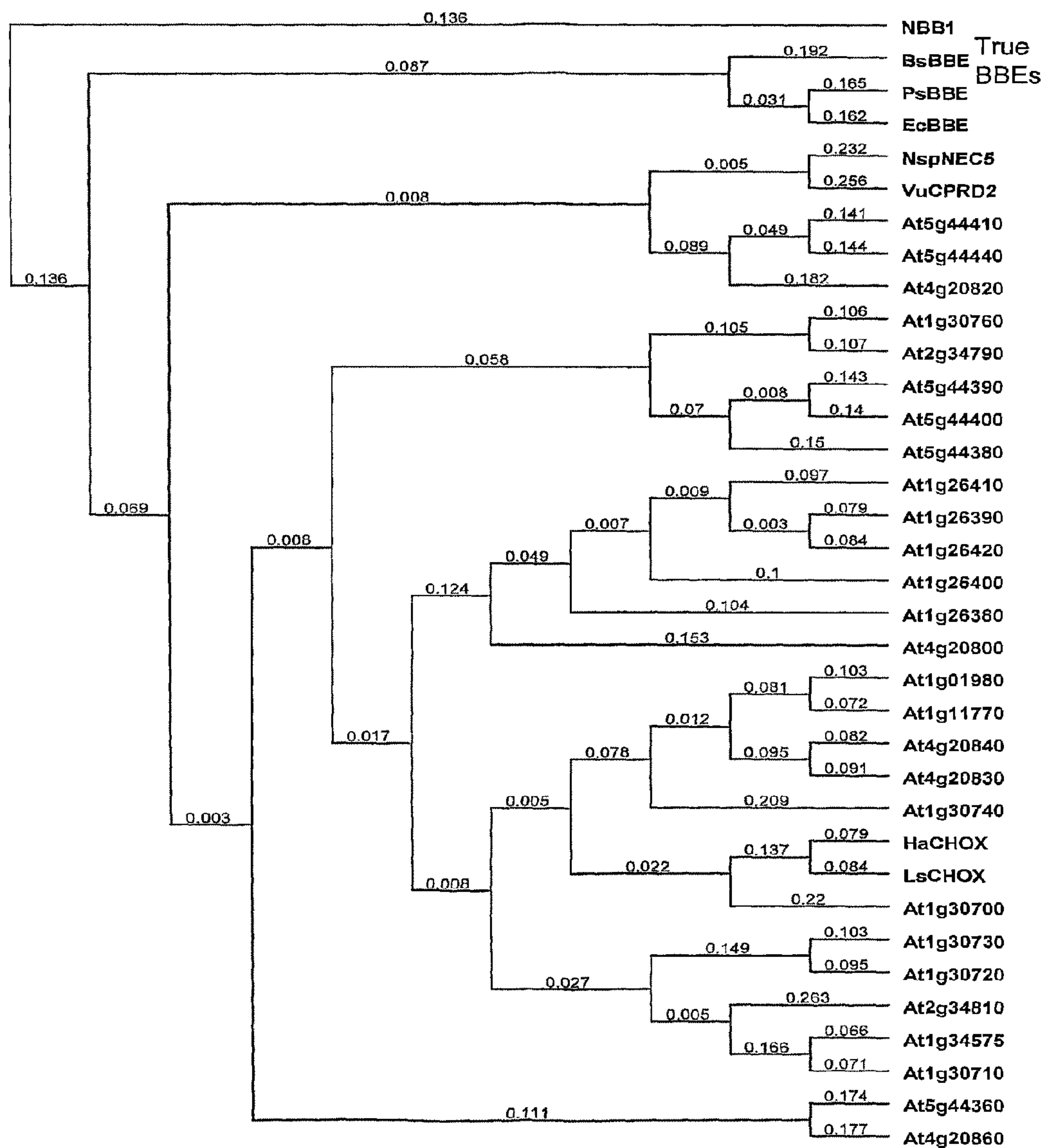
Phylogenetic tree constructed using the sequences of NBB1 polypeptide and plant BBE-like proteins
