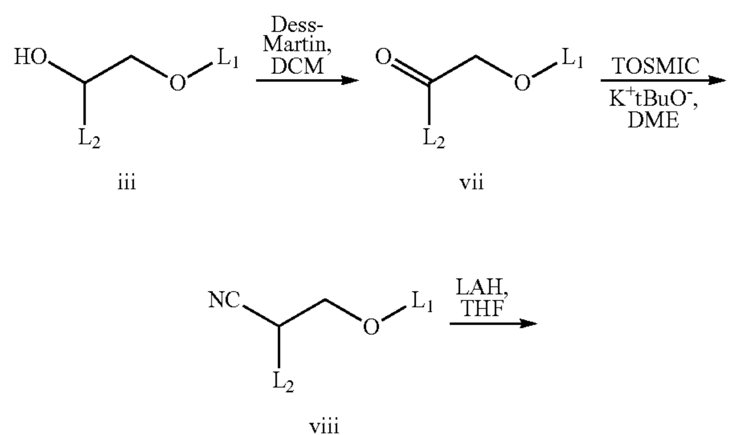
GENERAL SCHEME 3
