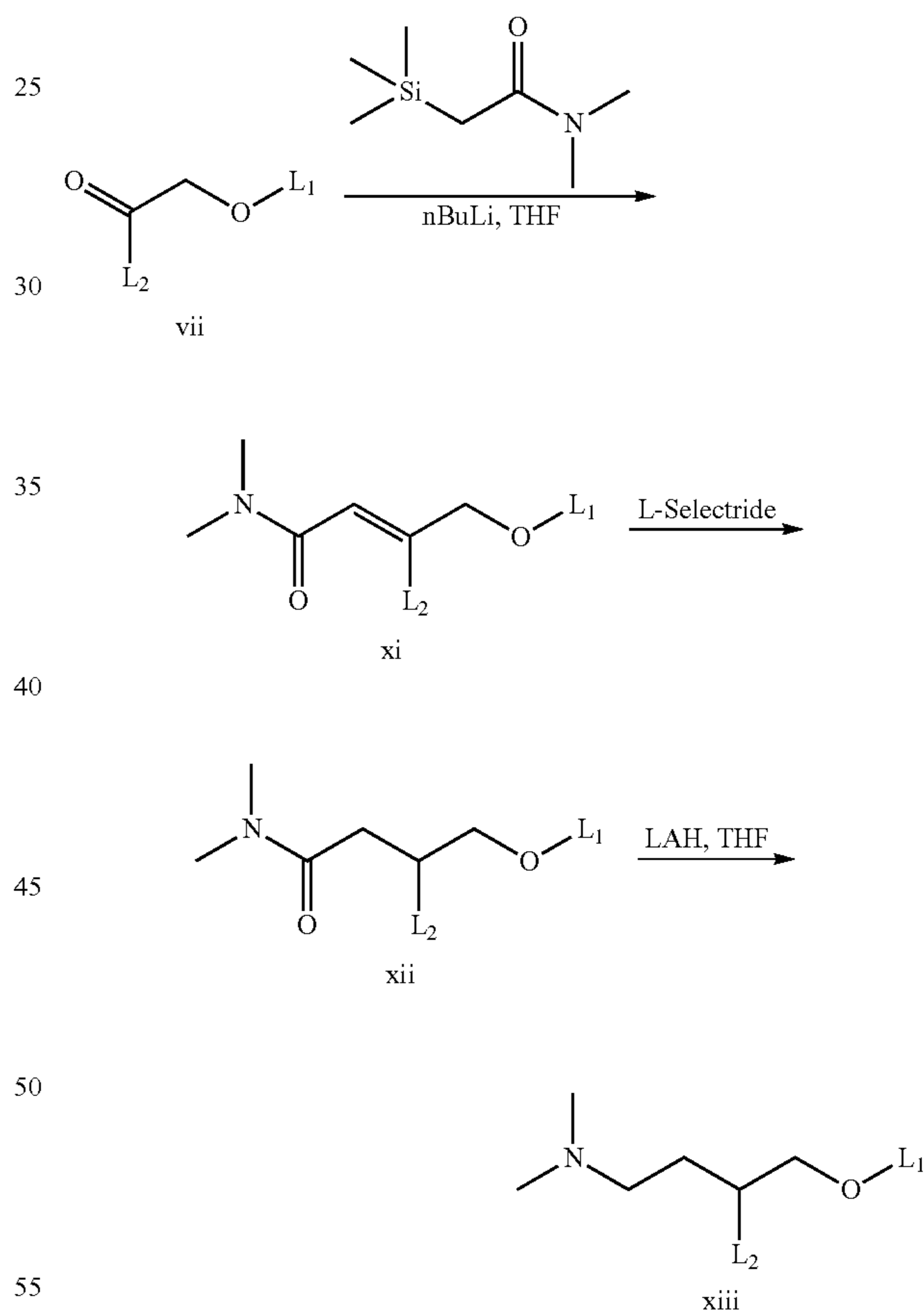
GENERAL SCHEME 4
