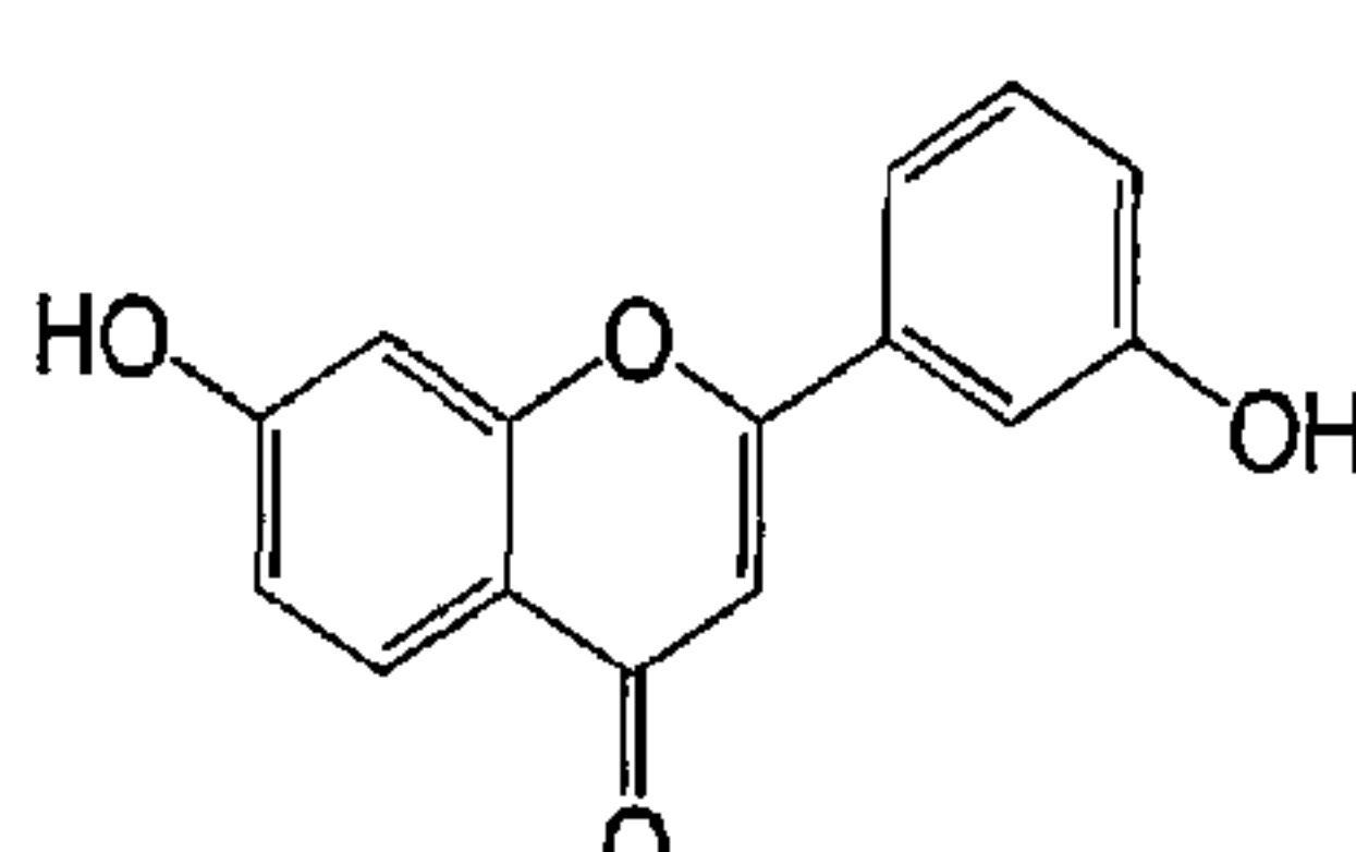
7, 3'-dihydroxyflavone
