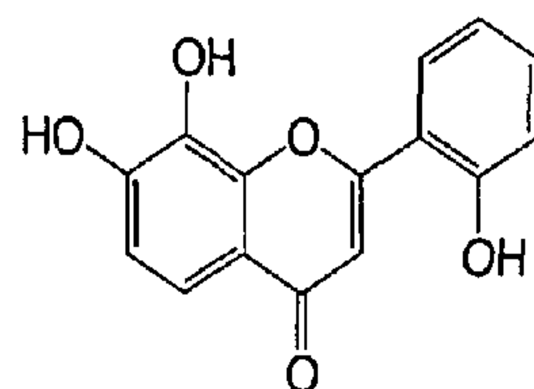
7, 8, 2'-trihydroxyflavone
