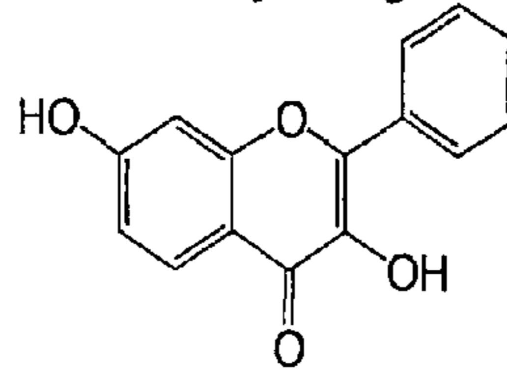
3, 7-dihydroxyflavone
