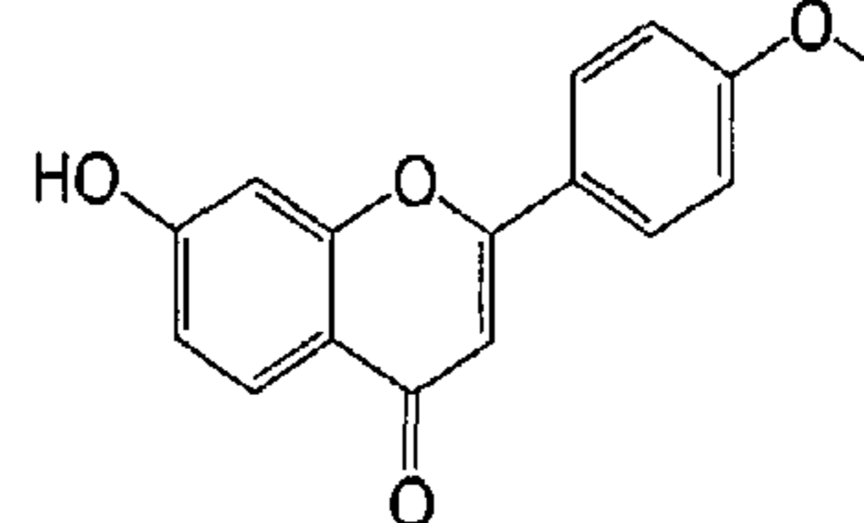
7-hydroxy-4'-methoxyflavone
