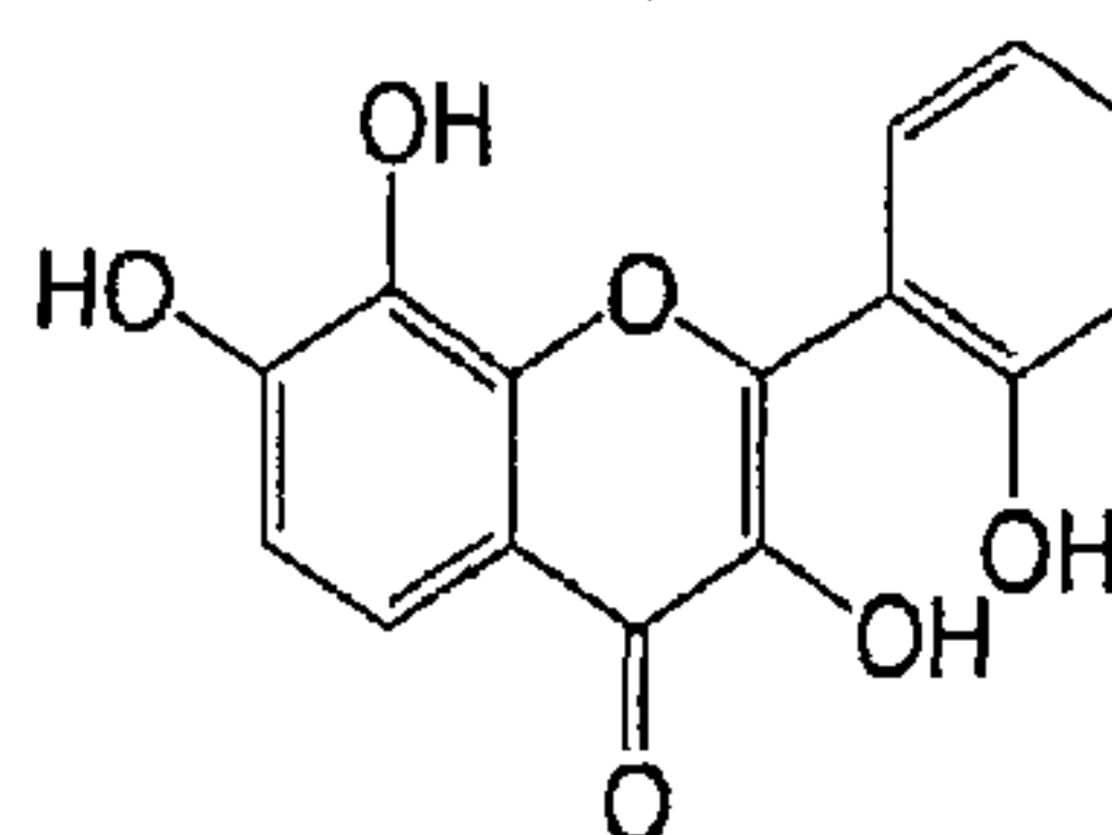
3, 7, 8, 2'-tetrahydroxyflavone
