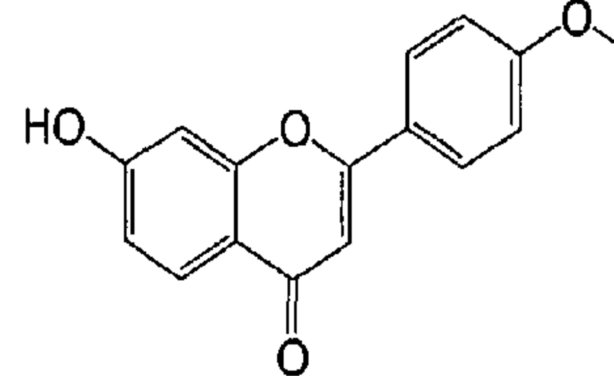
7-hydroxy-4'-methoxyflavone
