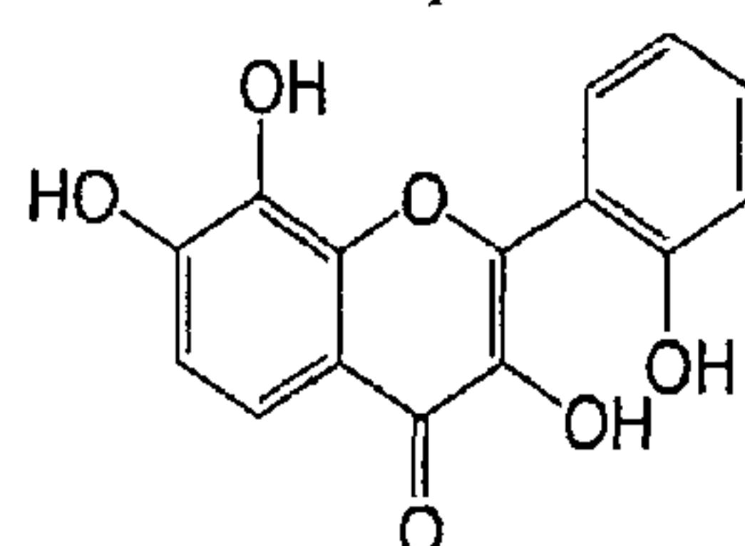
3, 7, 8, 2'-tetrahydroxyflavone
