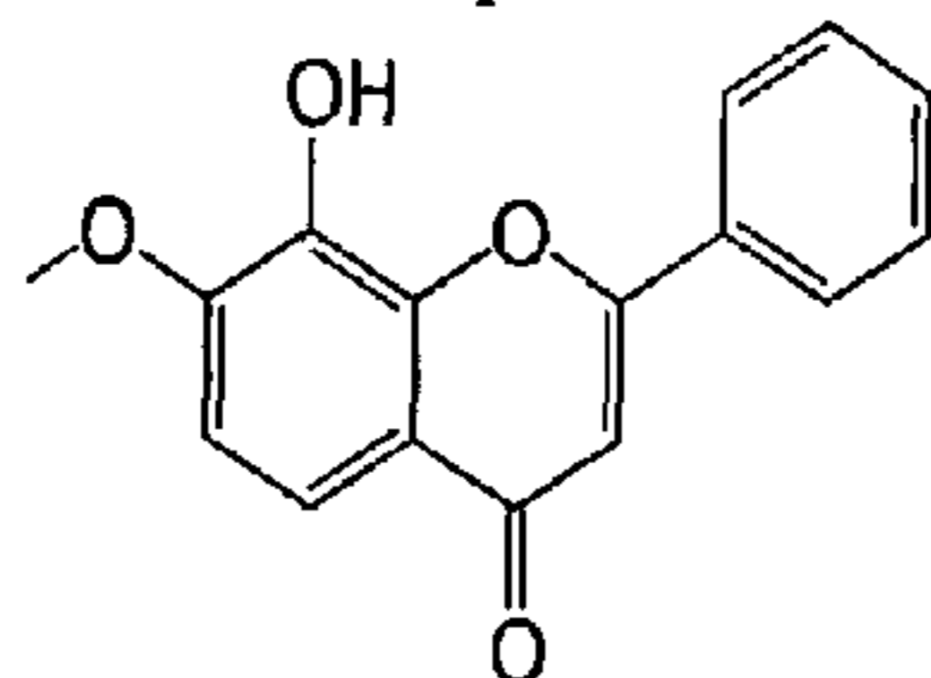
8-hydroxy-7-methoxyflavone
