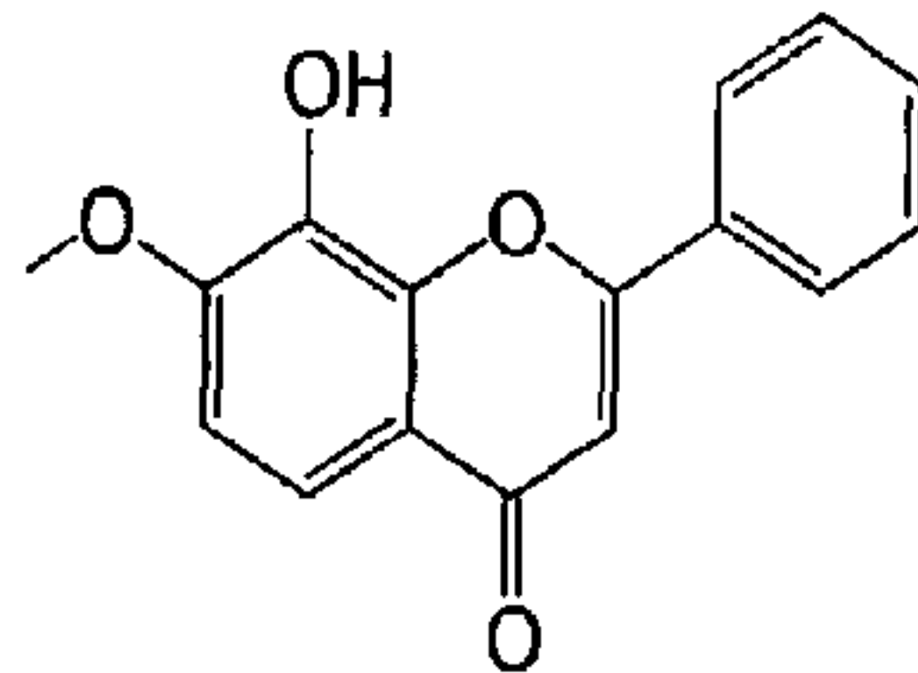
8-hydroxy-7-methoxyflavone
