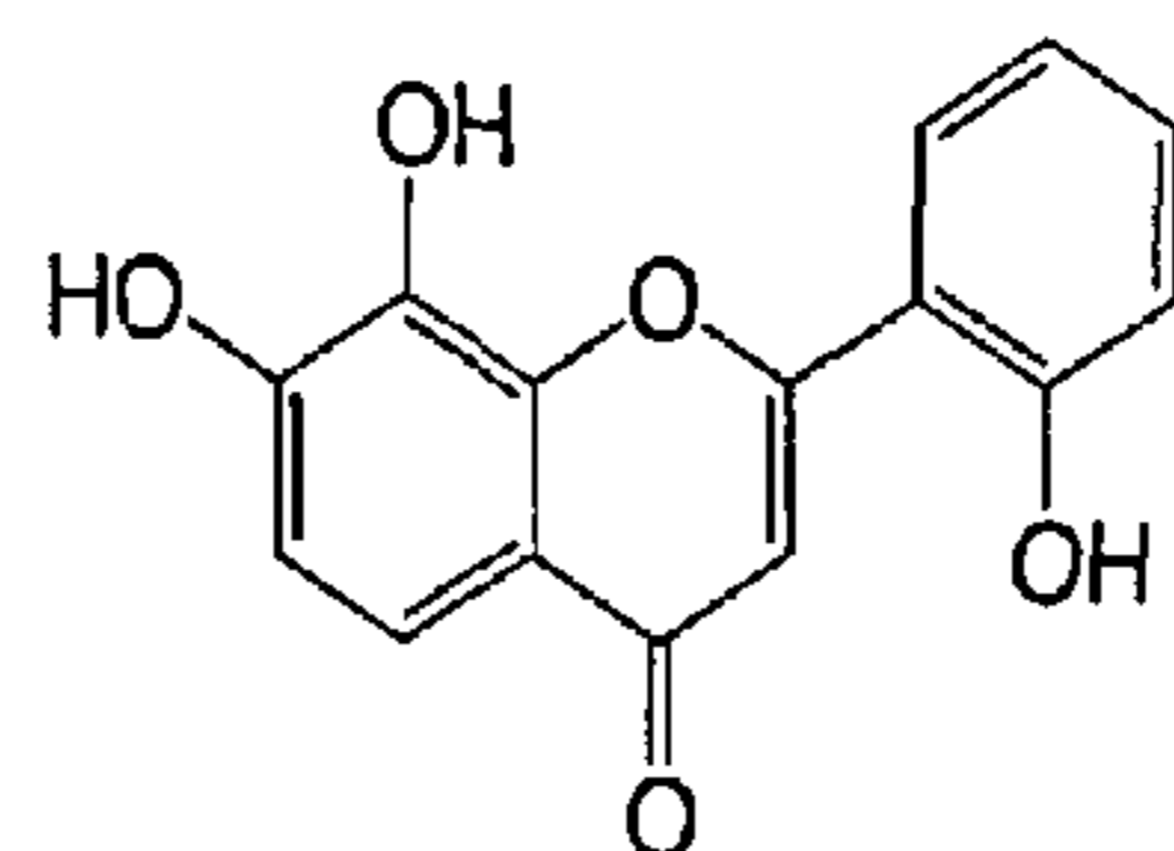
7, 8, 2'-trihydroxyflavone
