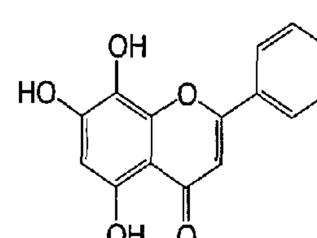
5, 7, 8-trihydroxyflavone
