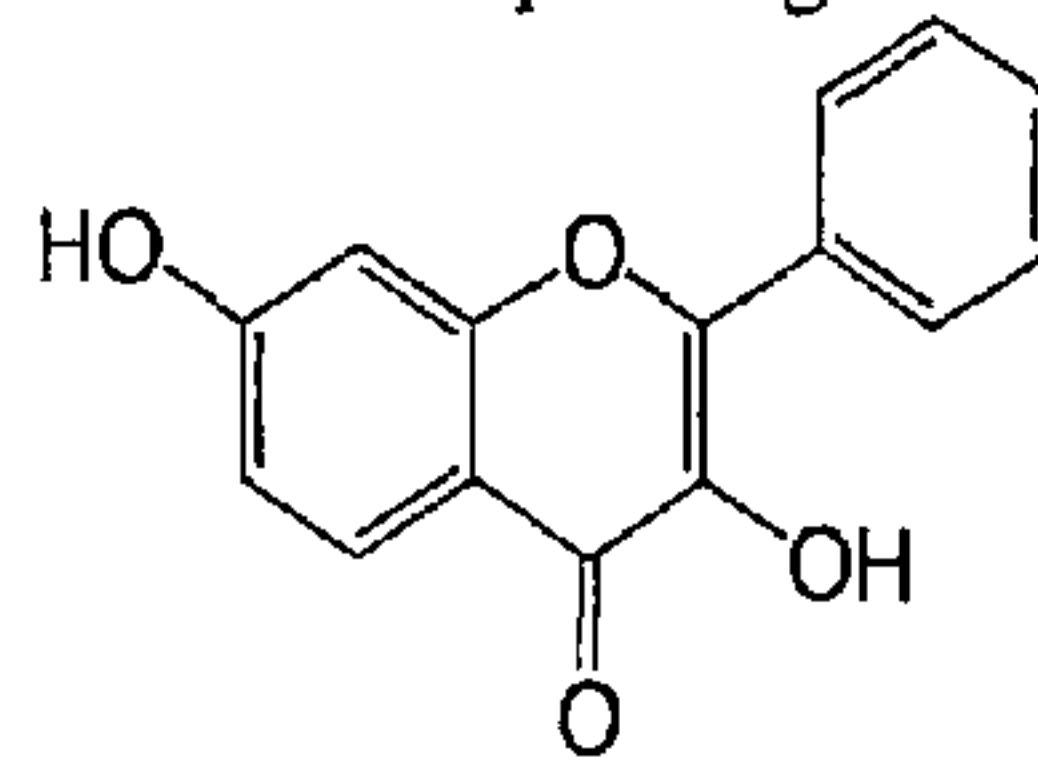
3, 7-dihydroxyflavone
