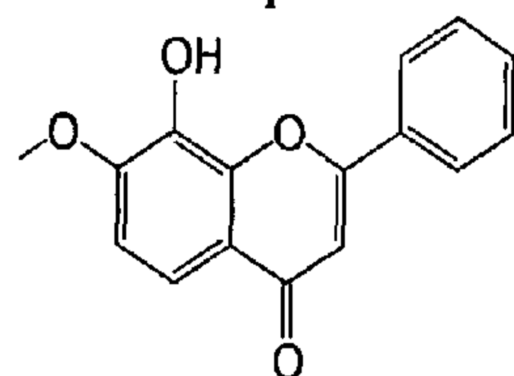
8-hydroxy-7-methoxyflavone
