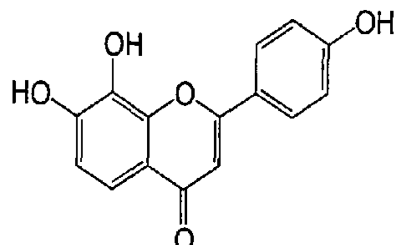
7, 8, 4'-trihydroxyflavone
