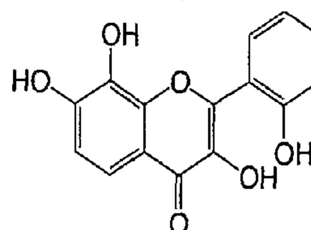
3, 7, 8, 2'-tetrahydroxyflavone
