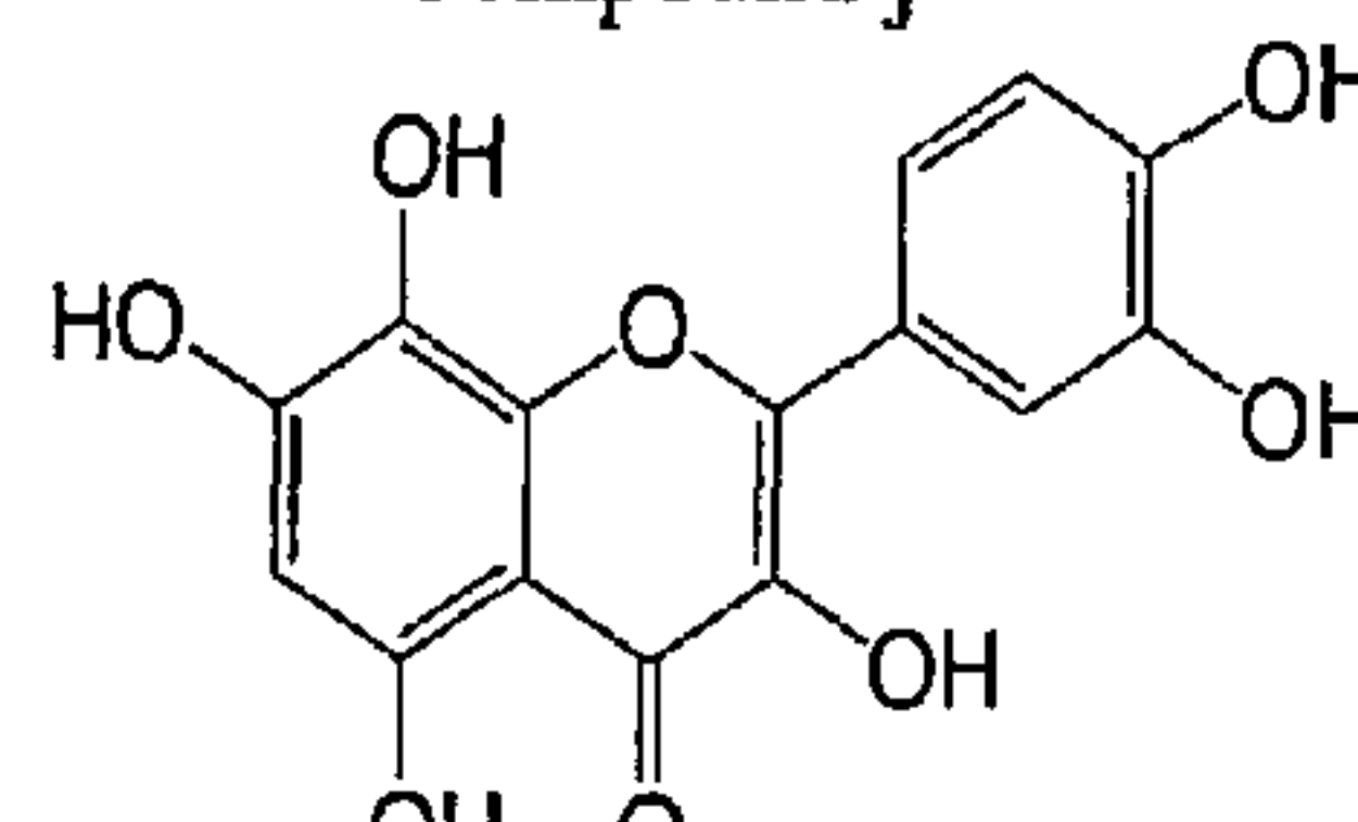
3, 5, 7, 8, 3', 4'-hexahydroxyflavone
