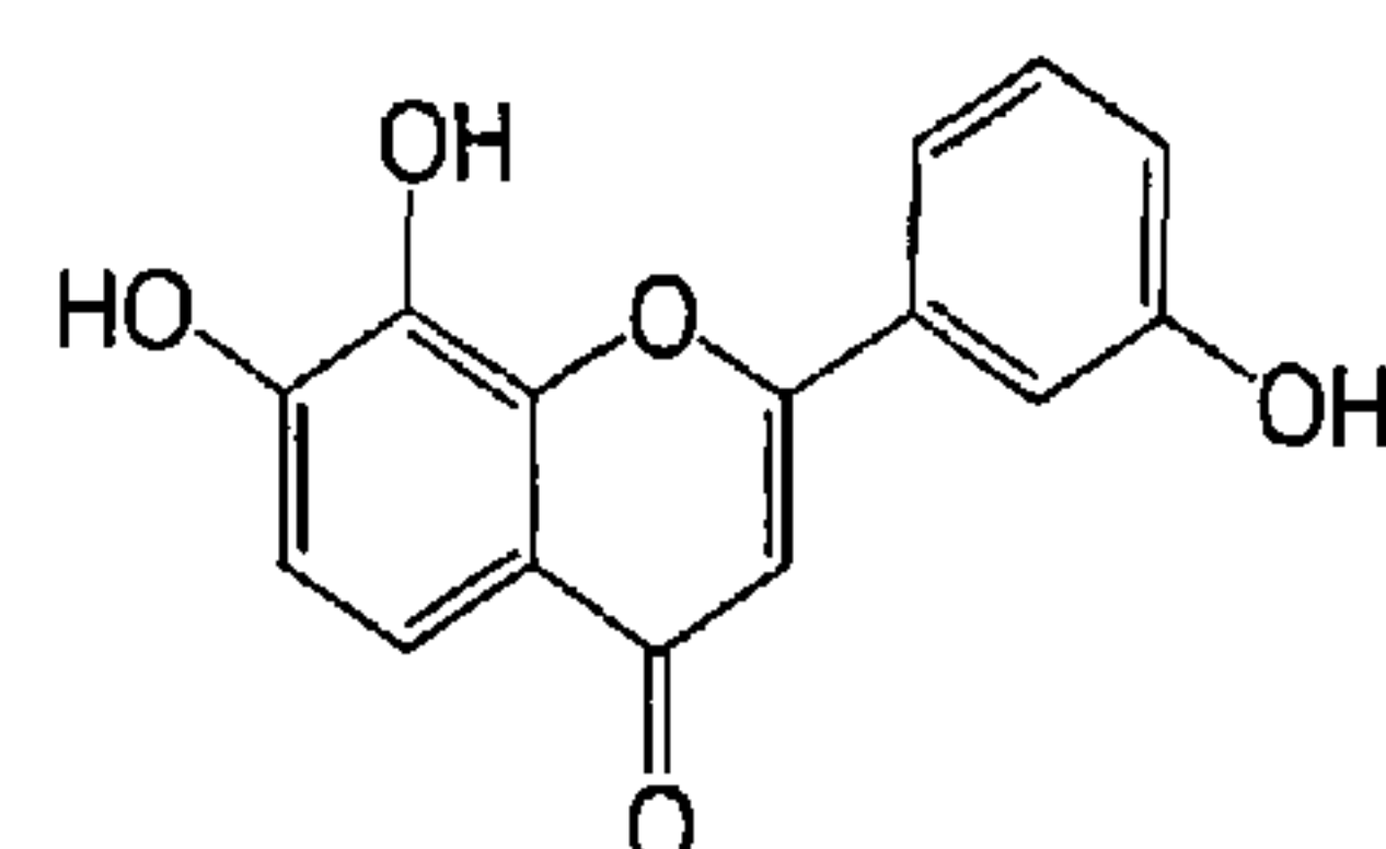
7, 8, 3'-trihydroxyflavone
