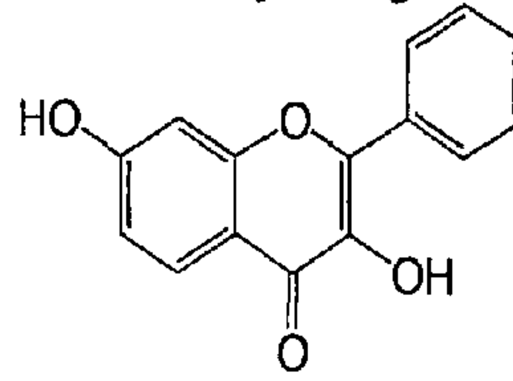
3, 7-dihydroxyflavone
