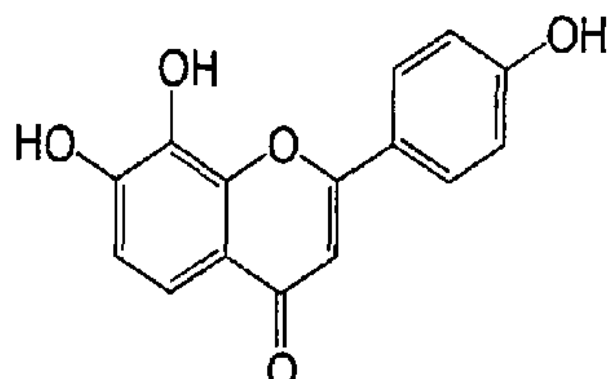
7, 8, 4'-trihydroxyflavone
