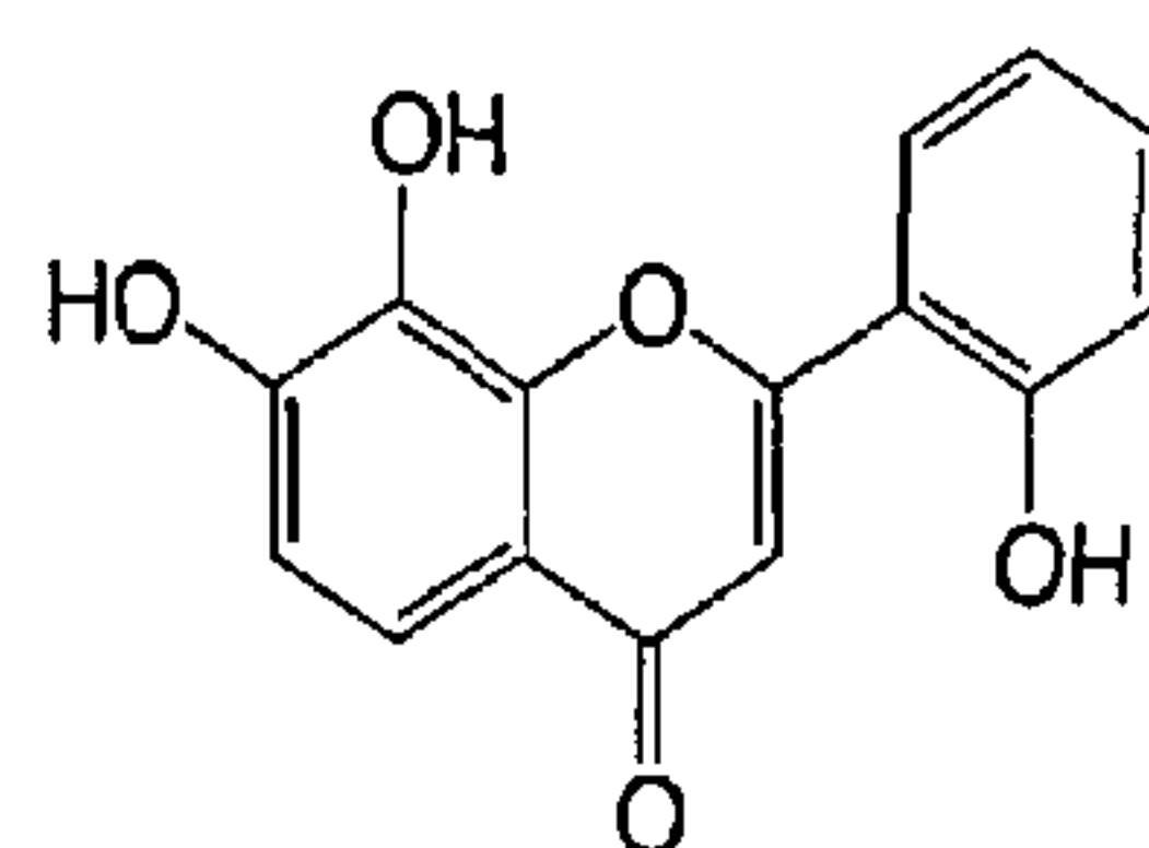
7, 8, 2'-trihydroxyflavone
