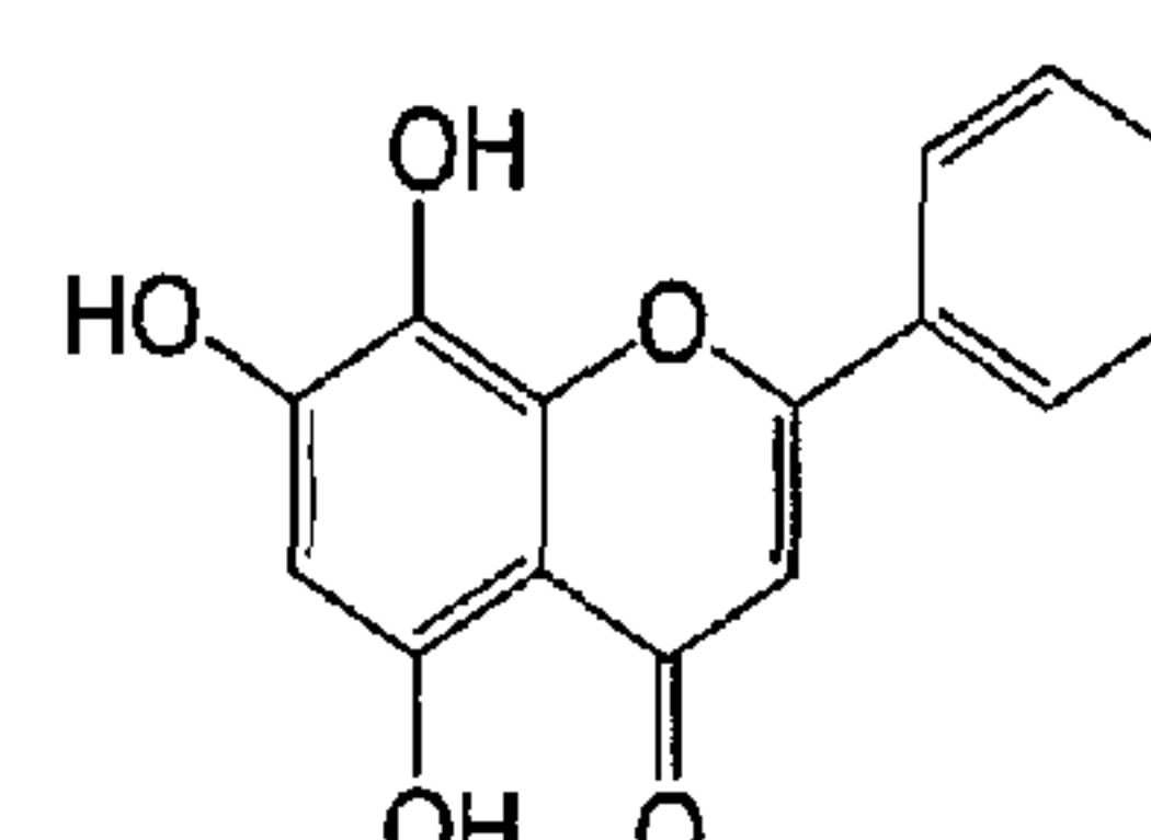
5, 7, 8-trihydroxyflavone
