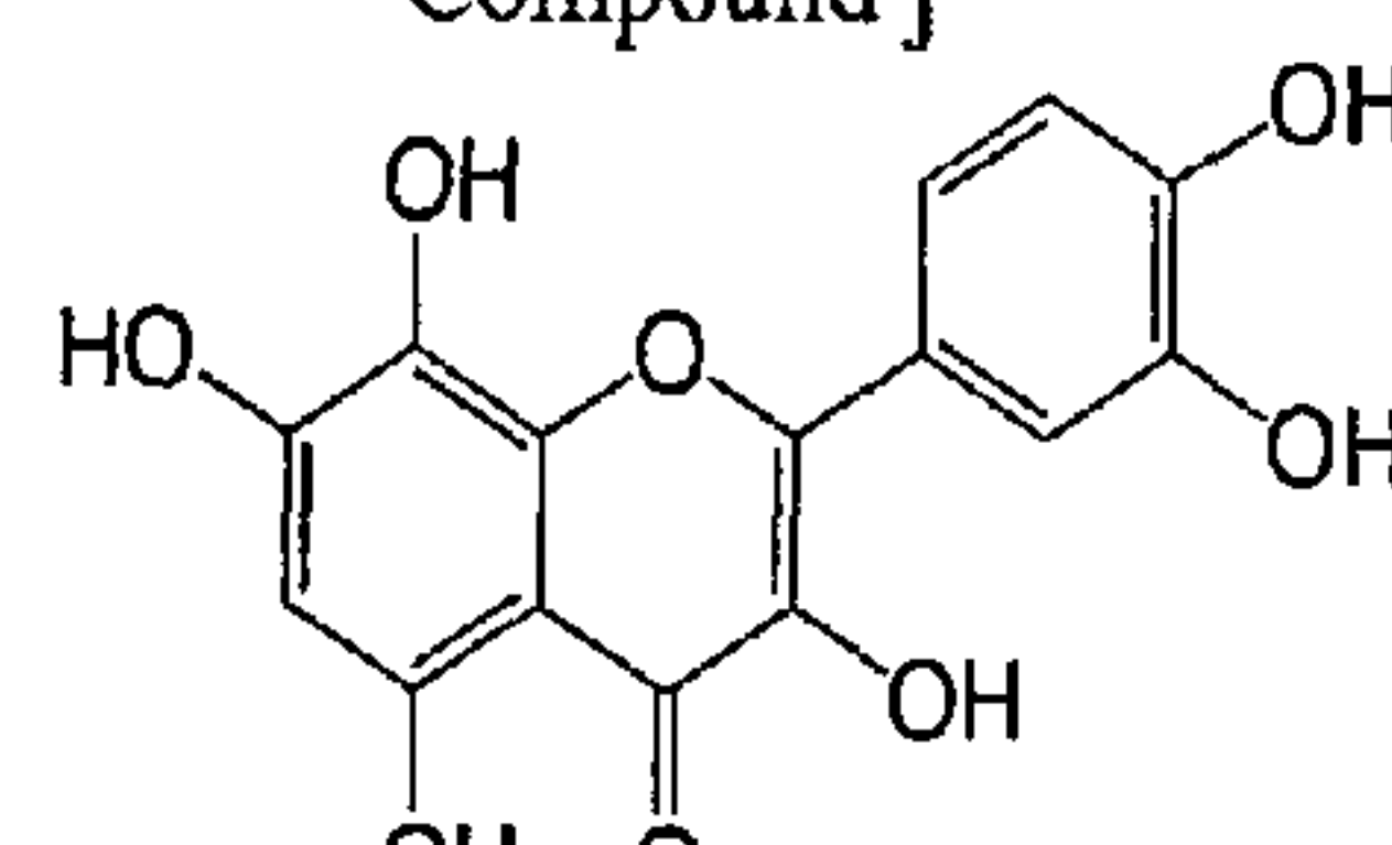
3, 5, 7, 8, 3', 4'-hexahydroxyflavone
