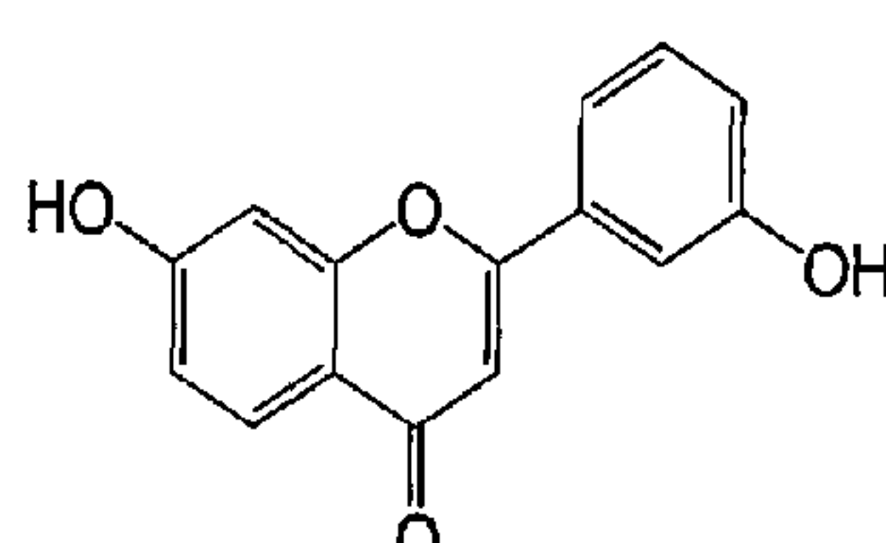
7, 3'-dihydroxyflavone
