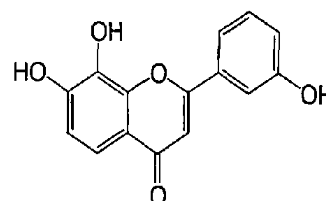
7, 8, 3'-trihydroxyflavone
