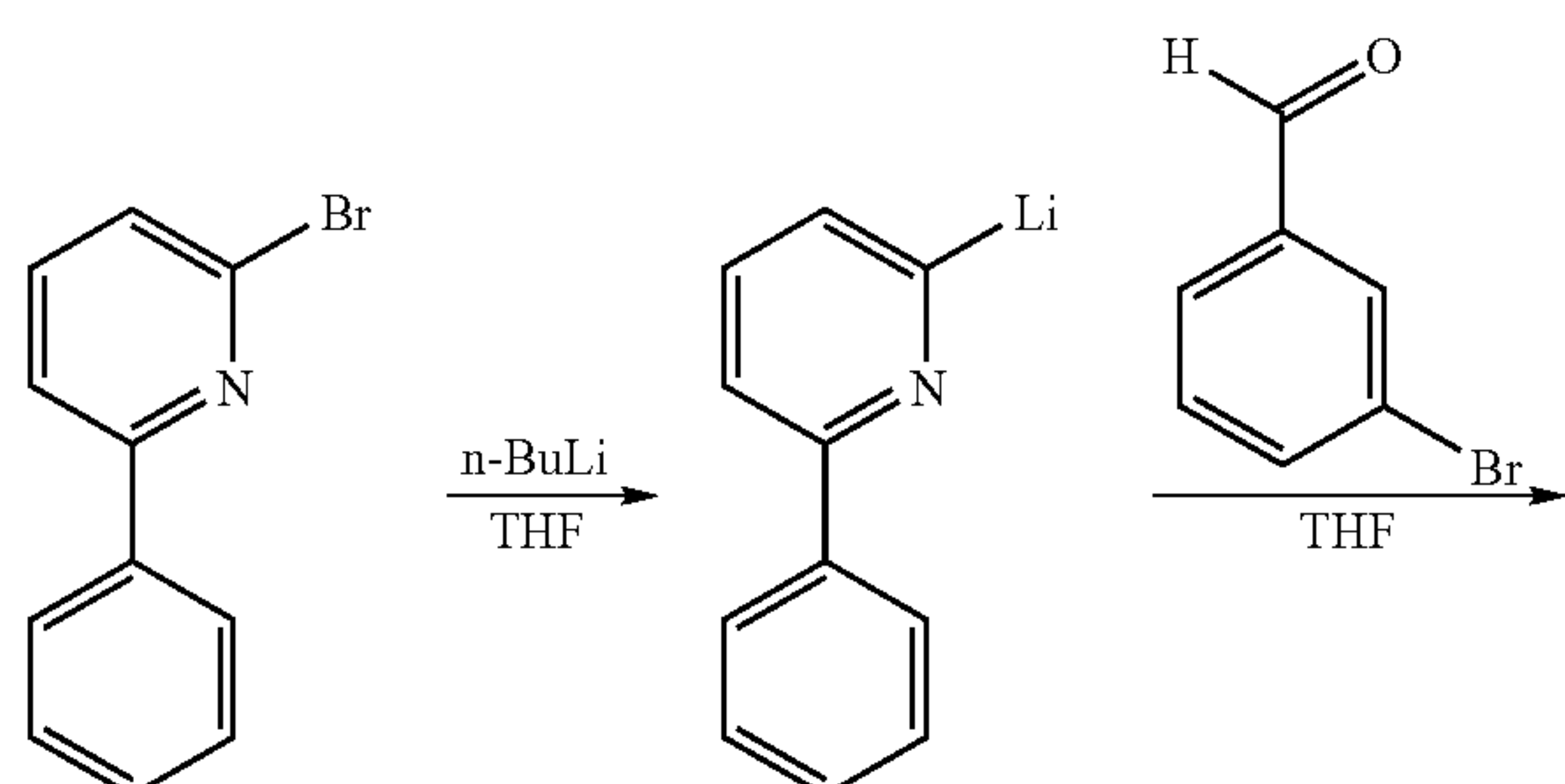
Scheme 7:
