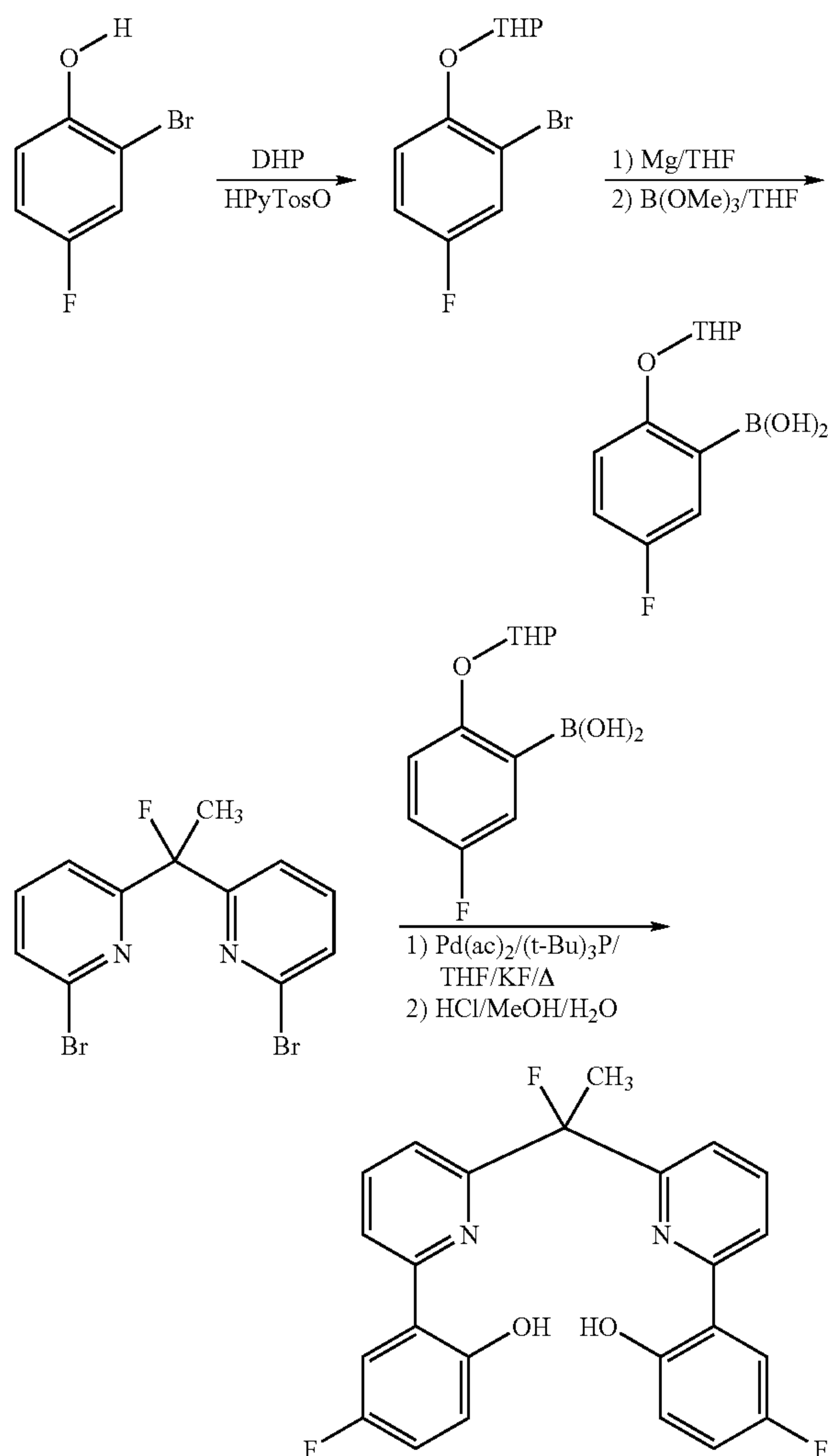
Scheme 6:
