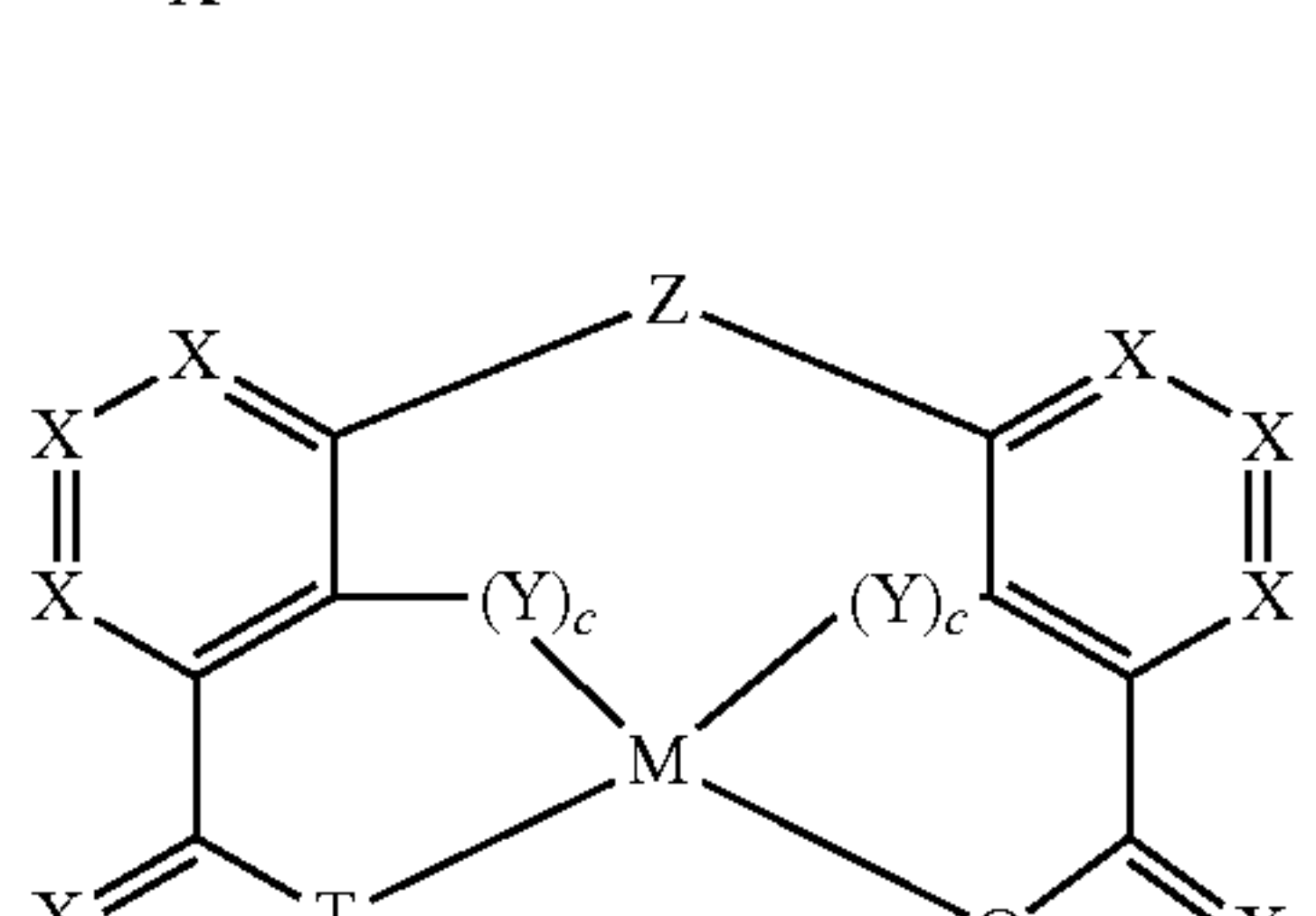
Compounds (18)
