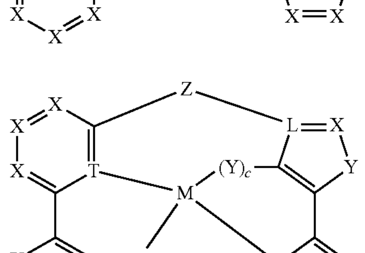
Compounds (20)
