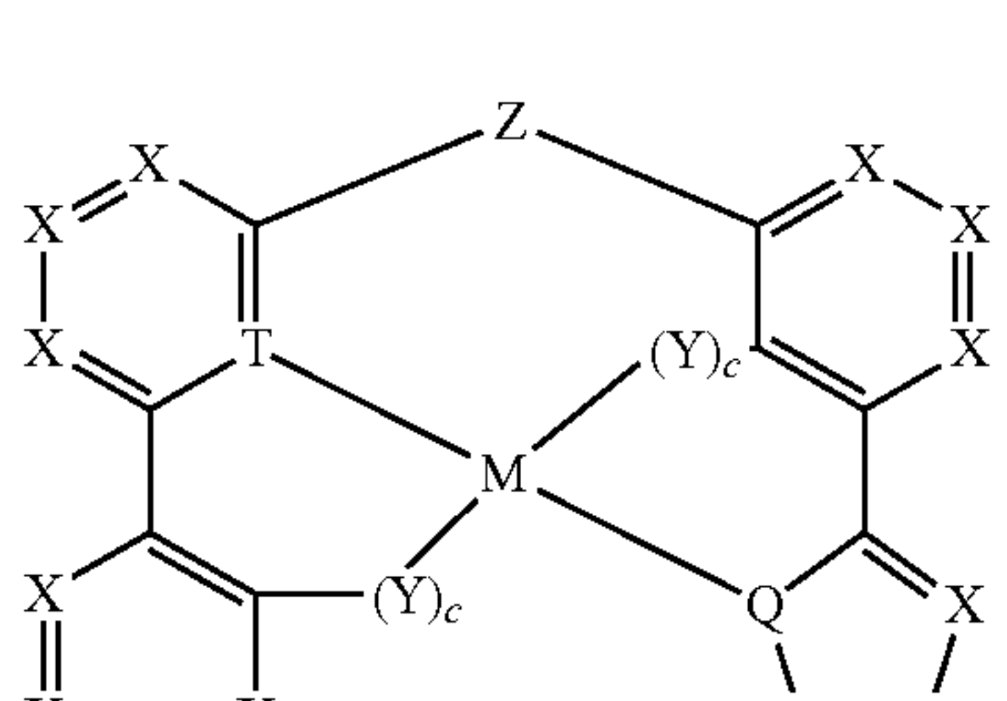
Compounds (17)
