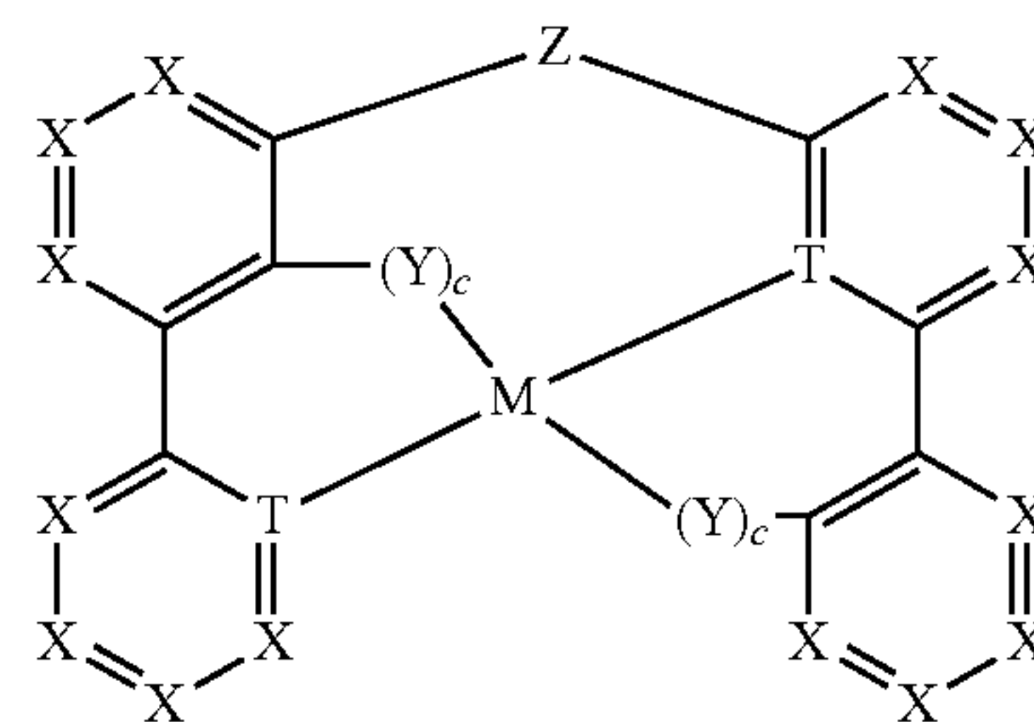
Scheme 2:
