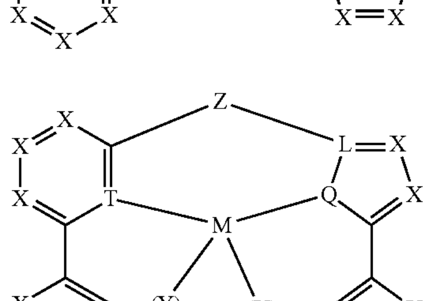
Compounds (19)
