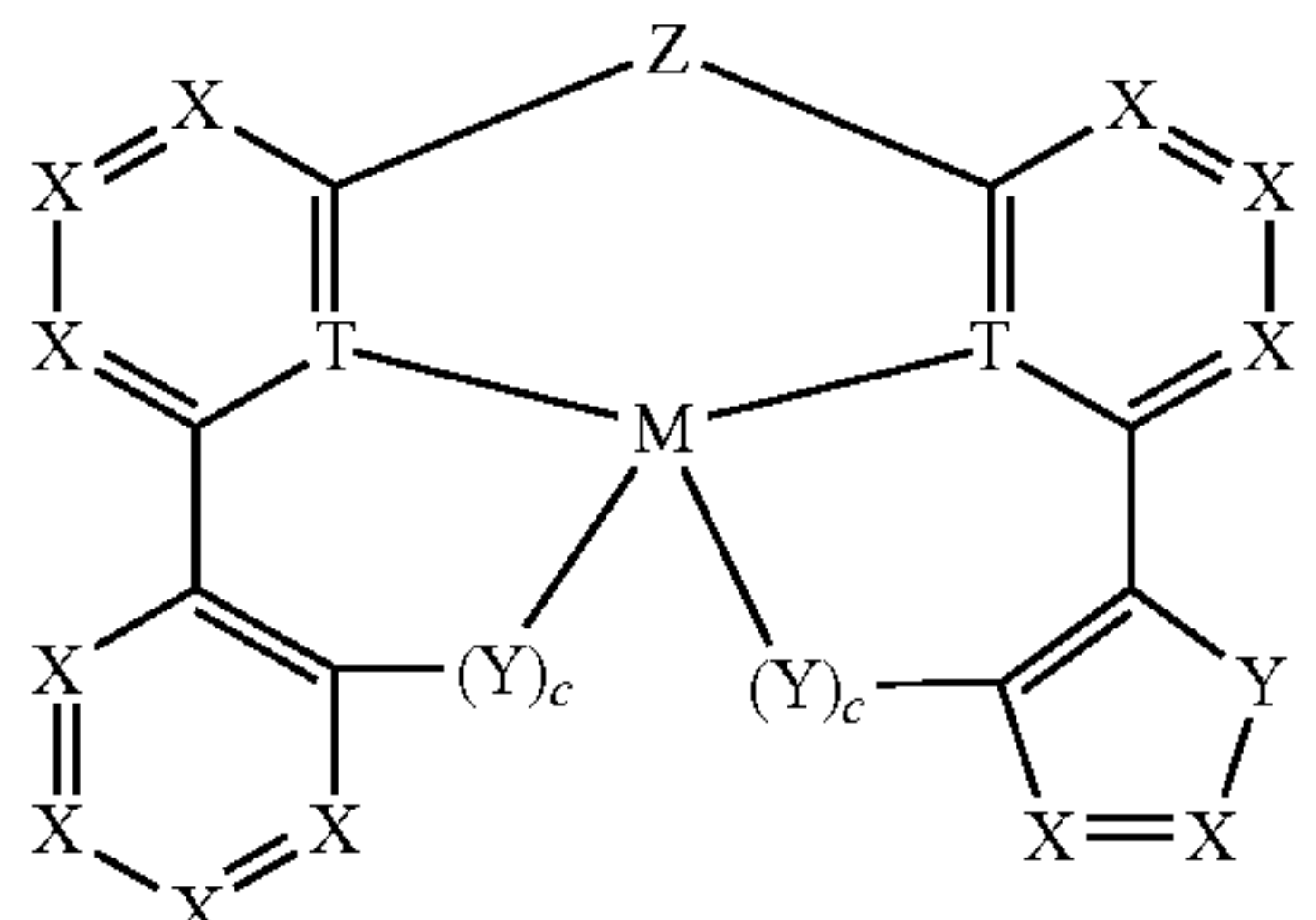
Scheme 3:
