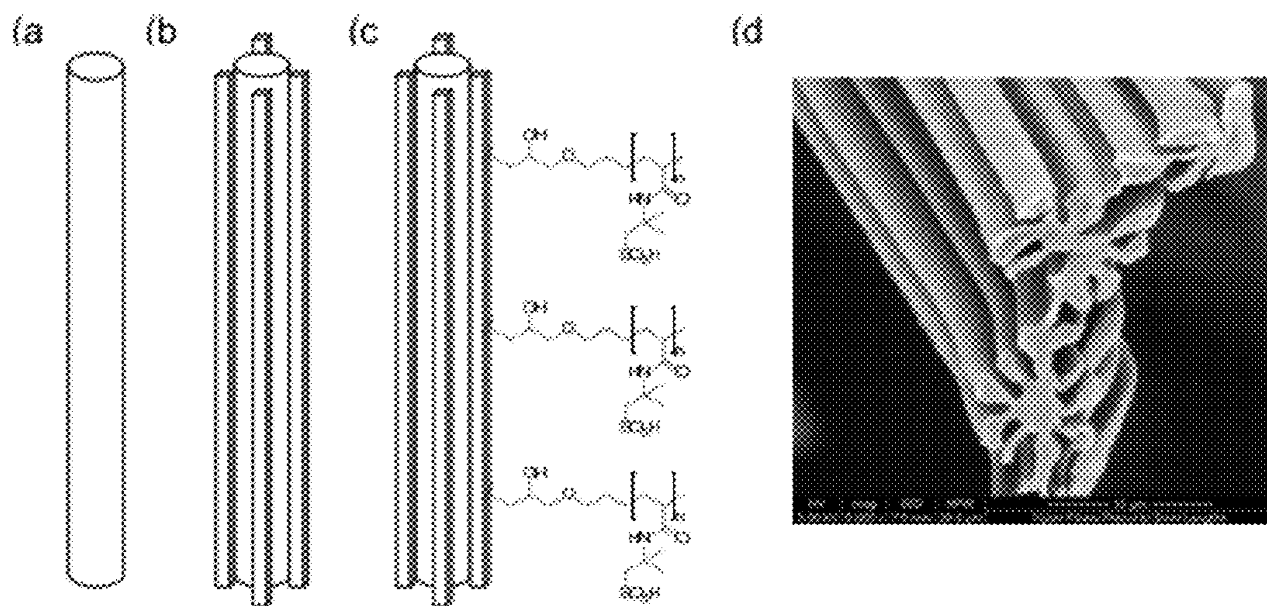
1(a)-c): A schematic illustration of fibers of the inventive concept. 1(d): SEM image of Allasso Industries Corporation winged fibers.
