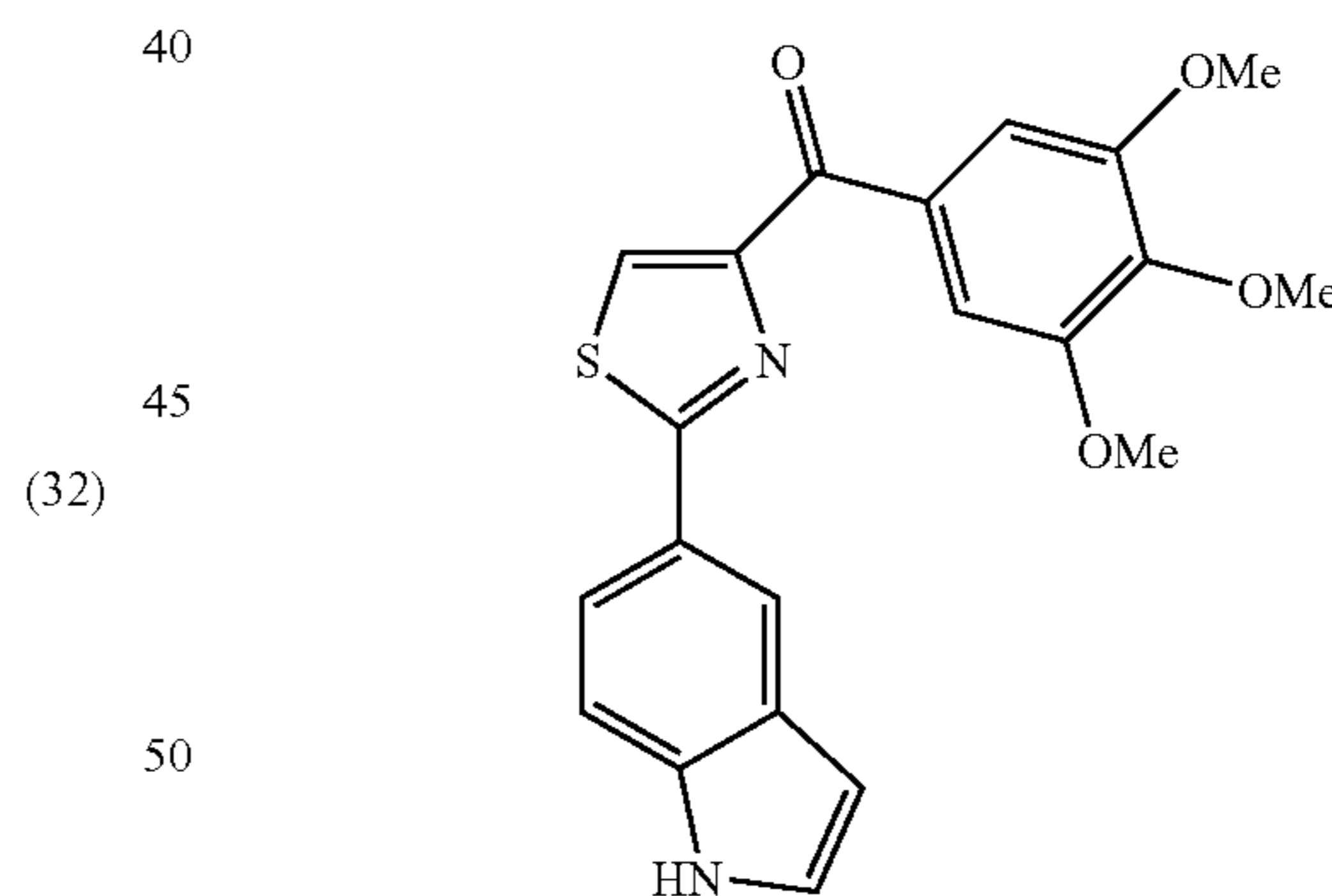
(R)-2-(1-(Phenylsulfonyl)-1H-indol-5-yl)-4,5-dihydrothiazole-4-carboxylic acid (64a)
