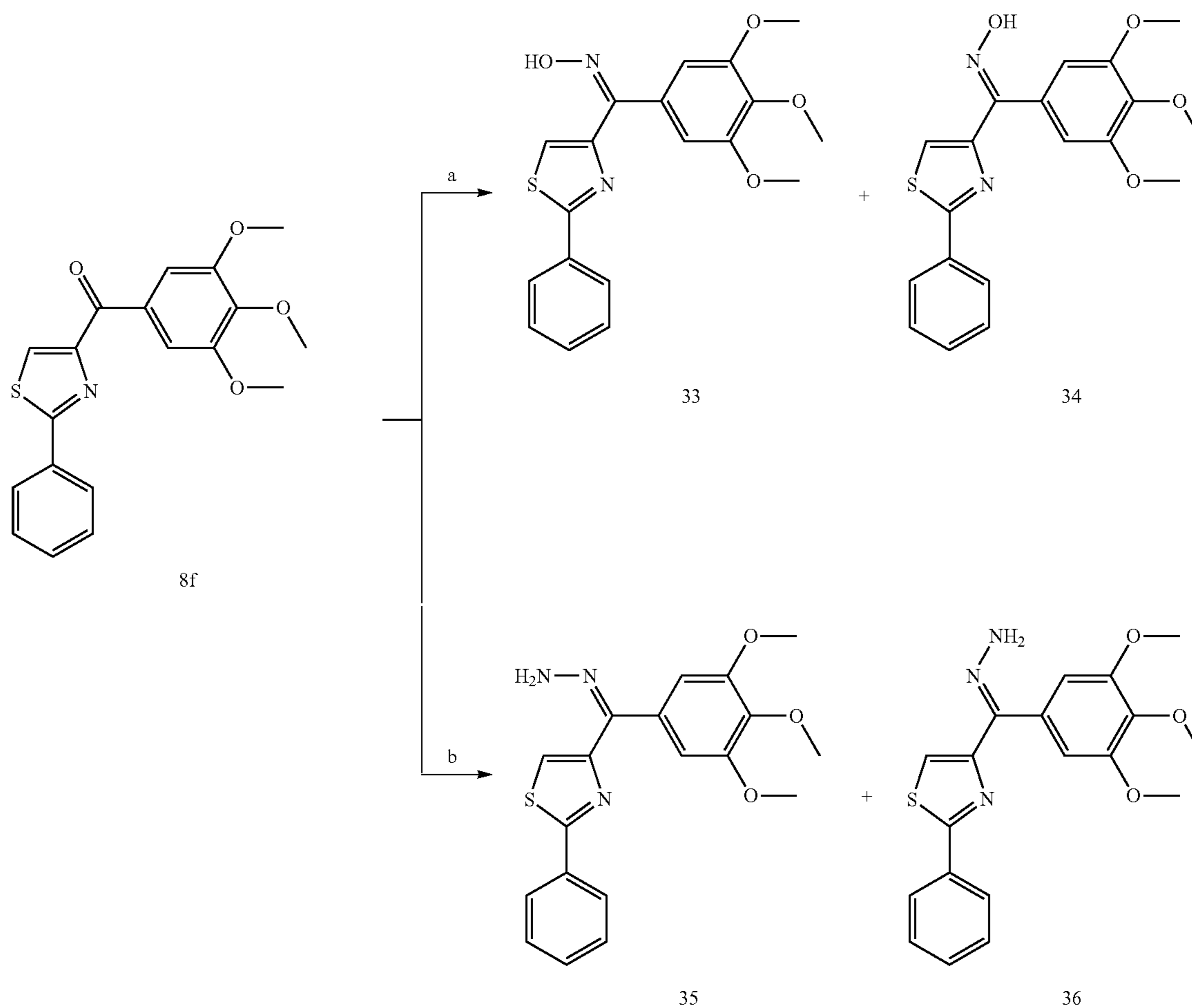
Scheme 4
