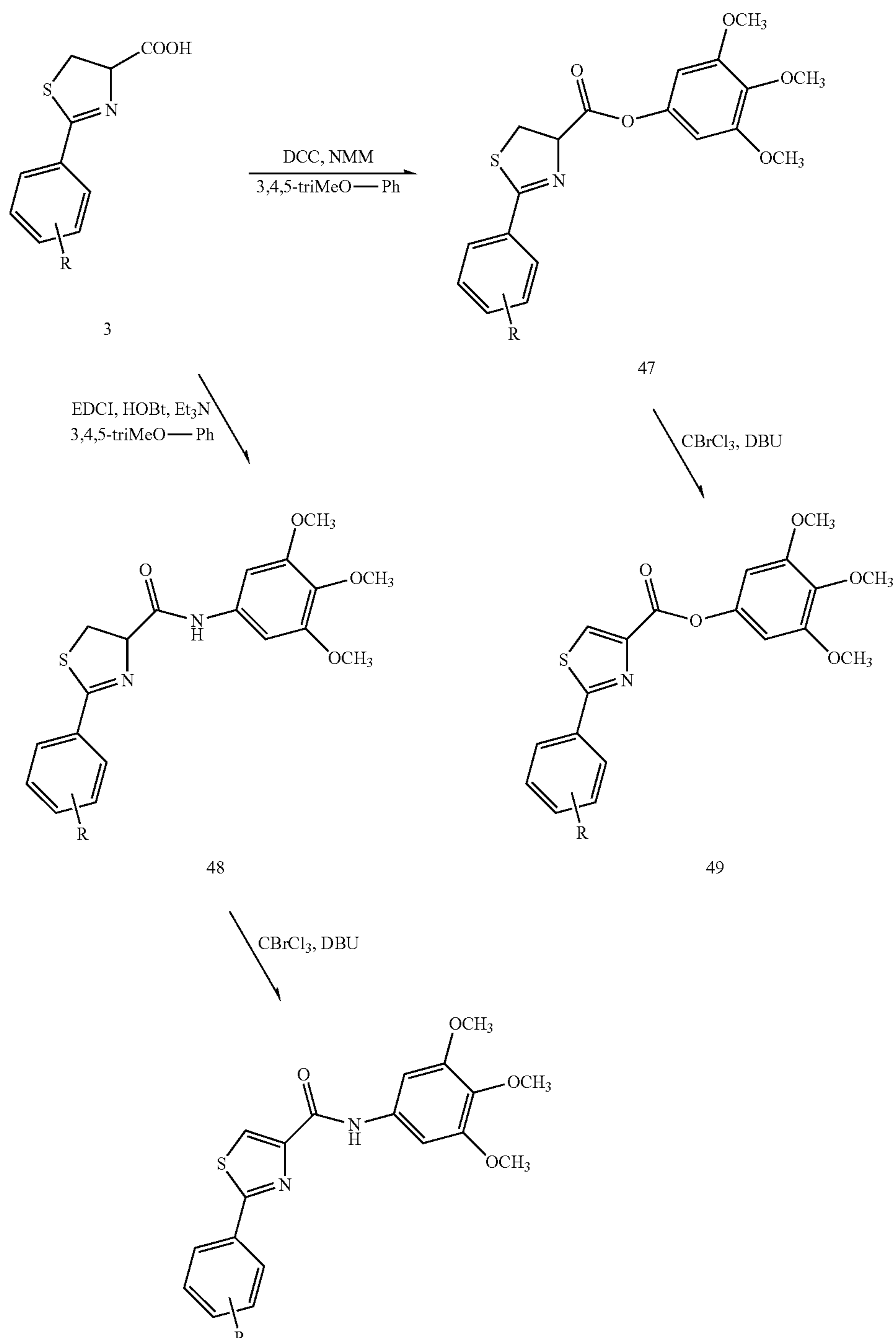
Scheme 7
