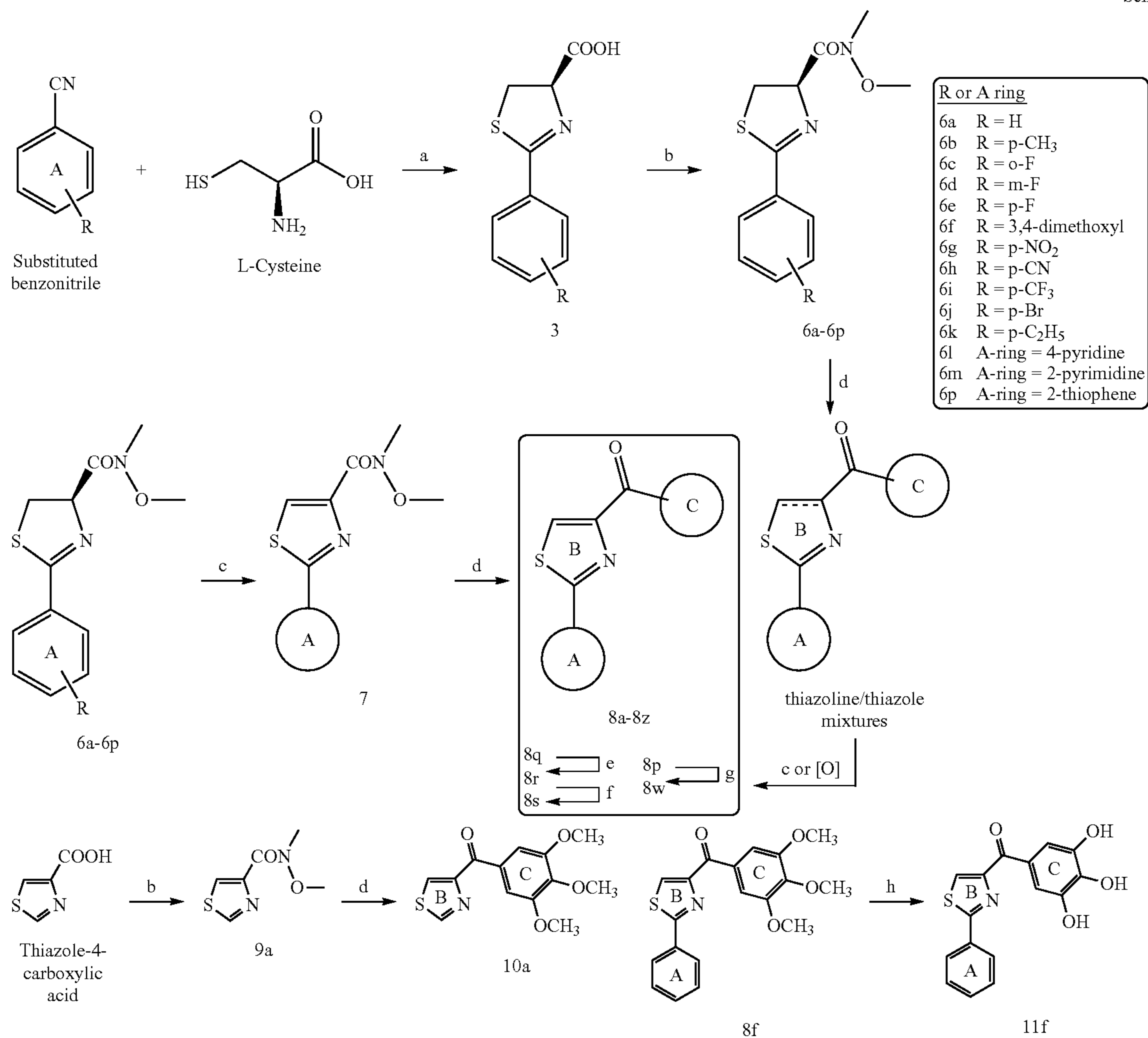
Scheme 3
