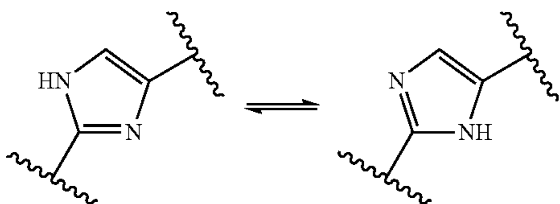
Tautomerization of the imidazole ring
