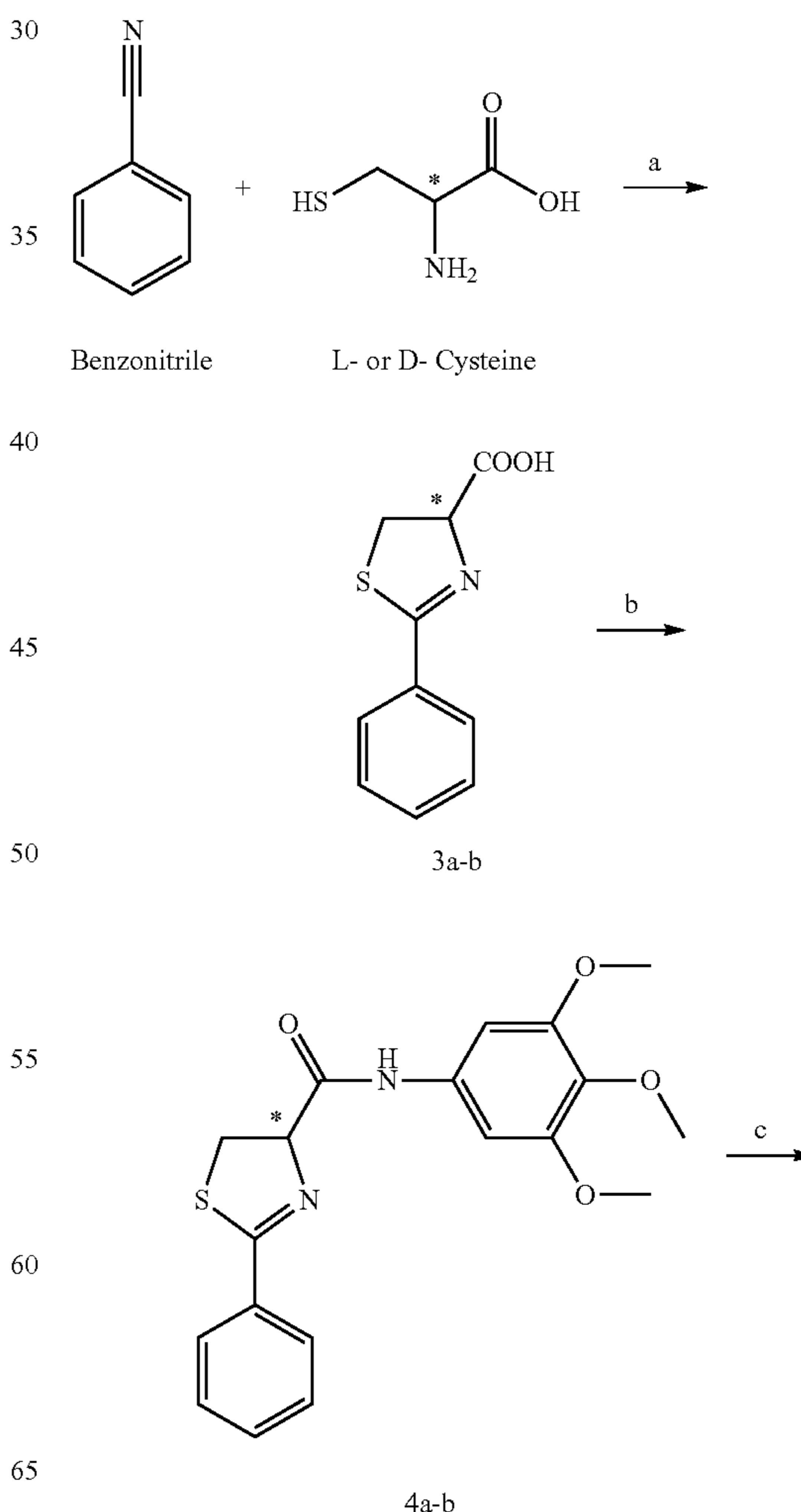
Scheme 2
