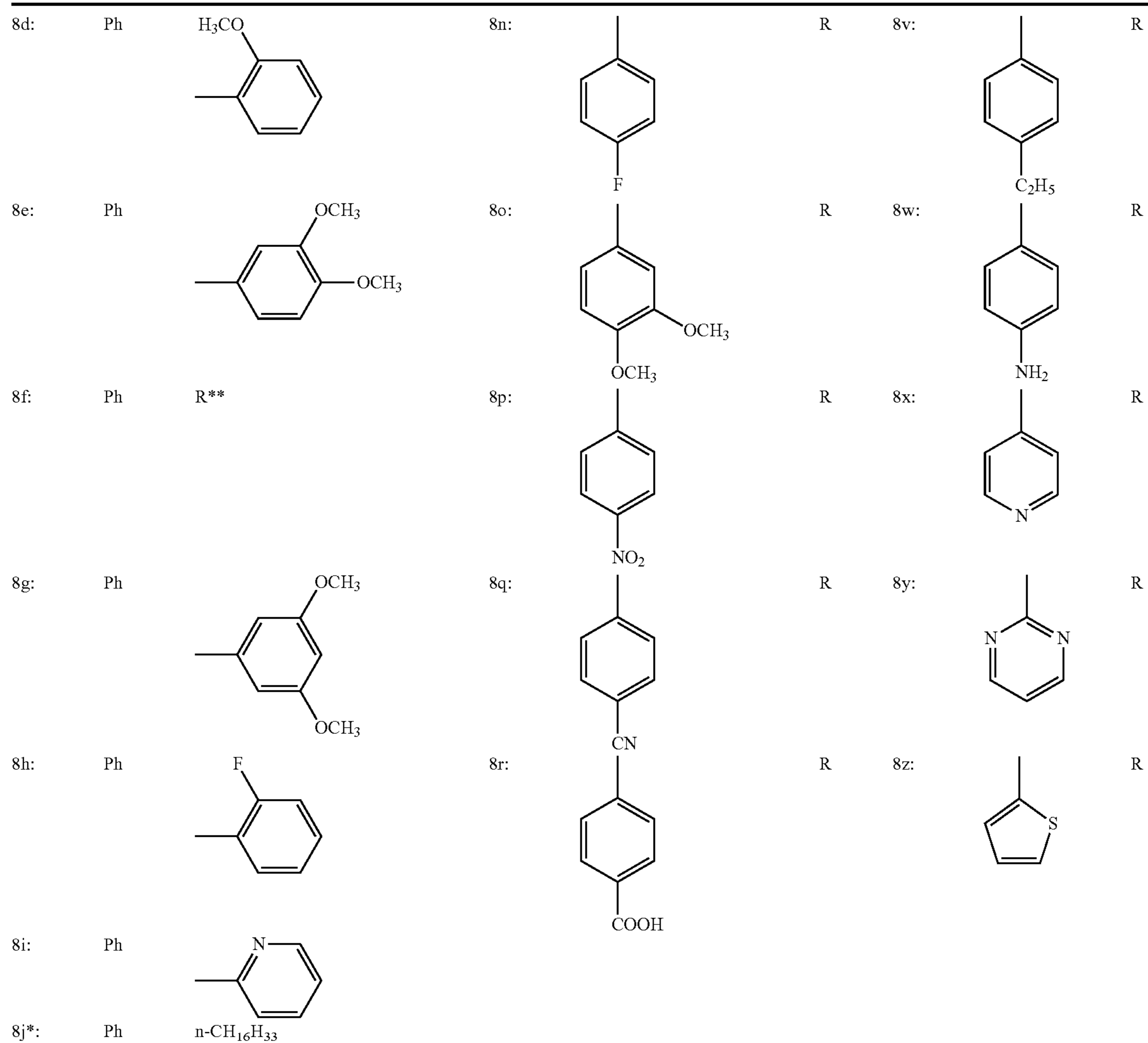
Scheme 3
