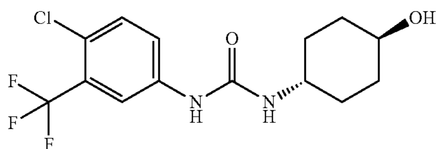
trans-1-(4-Chloro-3-trifluoromethyl-phenyl)-3-(4-hydroxy-cyclohexyl)-urea (07086)
