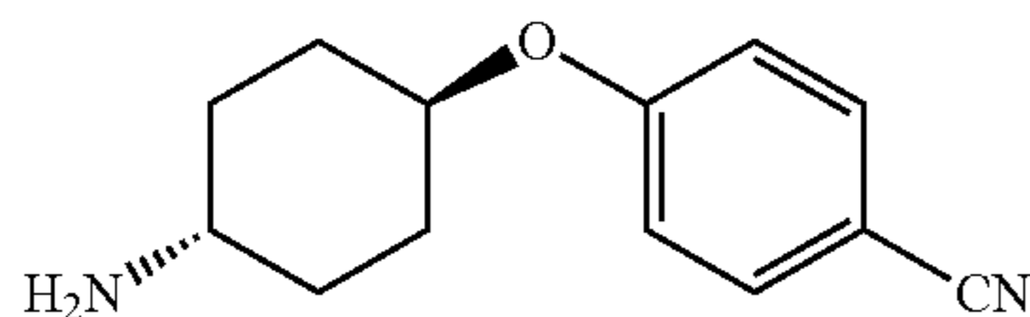
trans-4-(4-Amino-cyclohexyloxy)-benzonitrile
