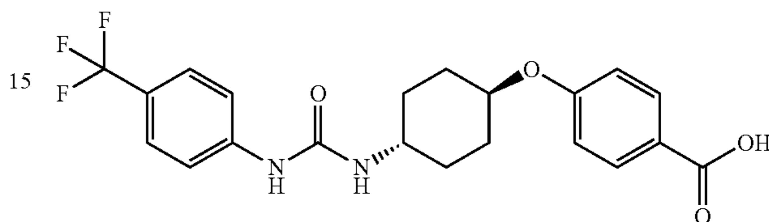
trans-4-{4-[3-(4-Trifluoromethyl-phenyl)-ureido]-cyclohexyloxy}-benzoic acid (2372)
