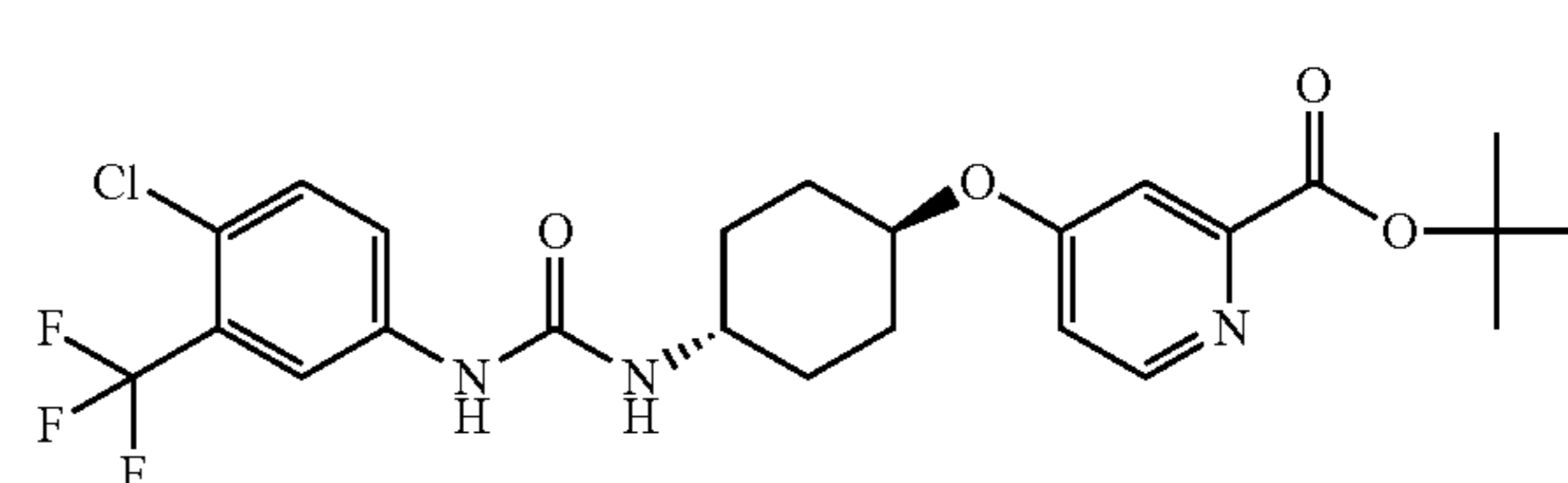
trans-4-{4-[3-(4-Chloro-3-trifluoromethyl-phenyl)-ureido]-cyclohexyloxy}-pyridine-2-carboxylic acid tert-butyl ester (2280)
