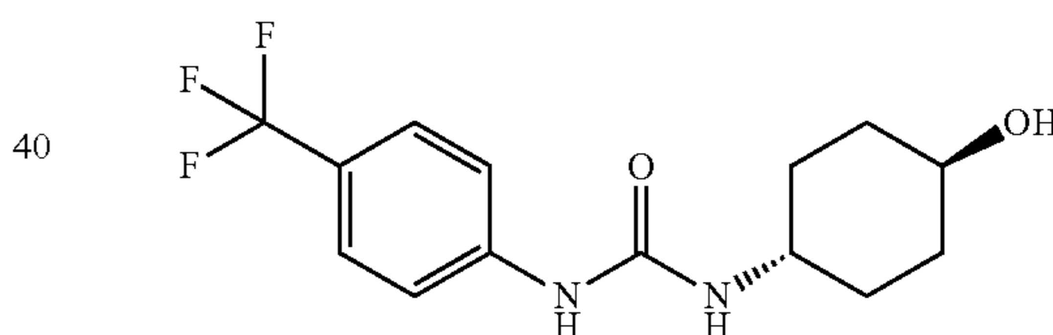
trans-1-(4-Hydroxy-cyclohexyl)-3-(4-trifluoromethyl-phenyl)-urea (08070)
