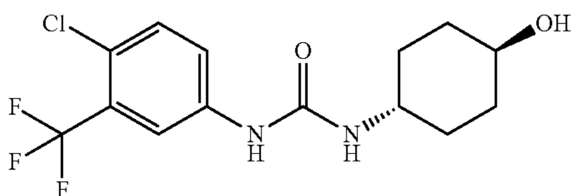
trans-1-(4-Chloro-3-trifluoromethyl-phenyl)-3-(4-hydroxy-cyclohexyl)-urea (07086)
