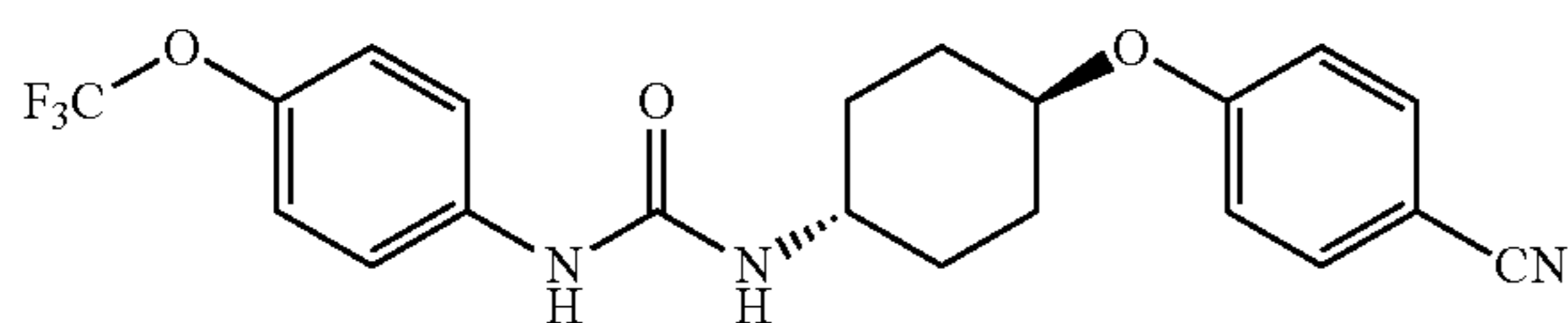
trans-1-[4-(4-Cyano-phenoxy)-cyclohexyl]-3-(4-trifluoromethoxy-phenyl)-urea (2581)
