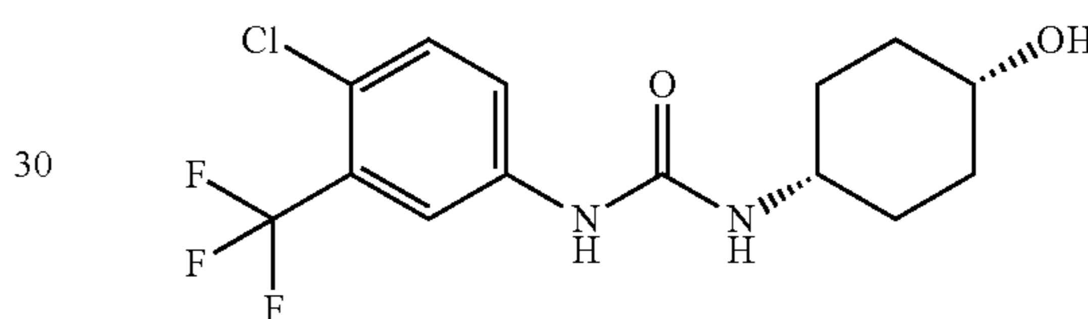
cis-1-(4-Chloro-3-trifluoromethyl-phenyl)-3-(4-hydroxy-cyclohexyl)-urea
