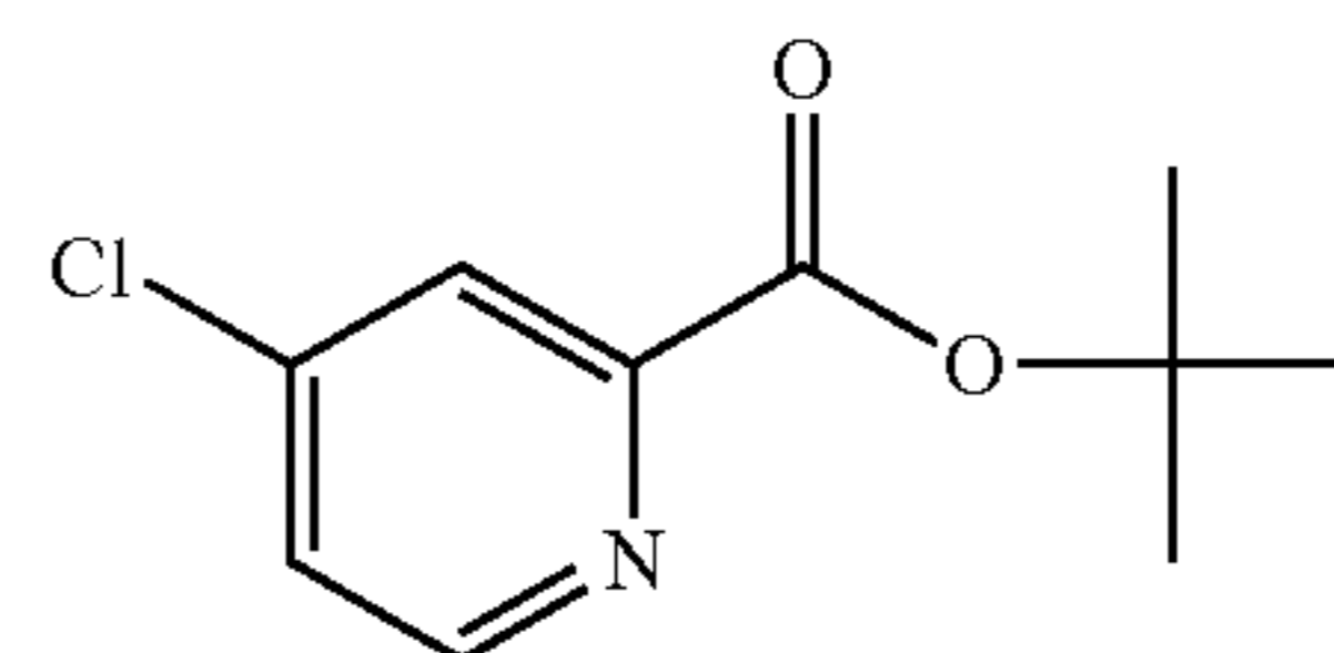
tert-Butyl 4-chloropicolinate
