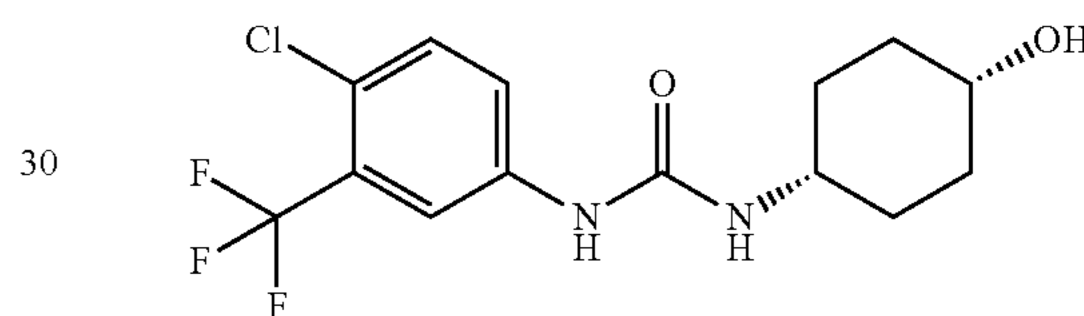
cis-1-(4-Chloro-3-trifluoromethyl-phenyl)-3-(4-hydroxy-cyclohexyl)-urea
