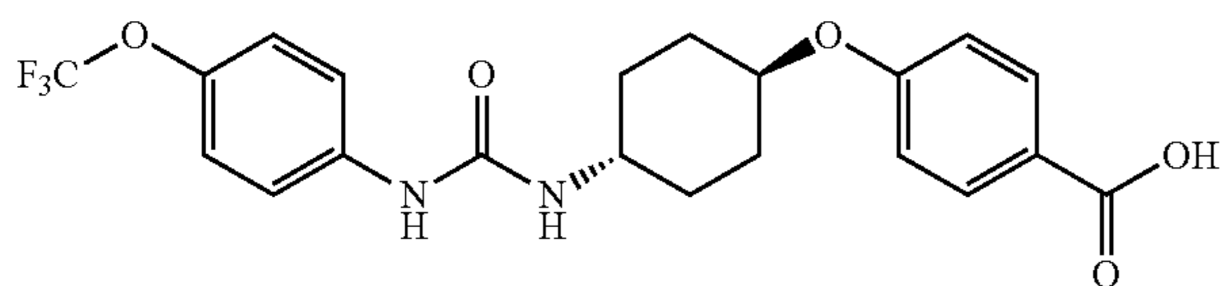
trans-4-{4-[3-(4-Trifluoromethoxy-phenyl)-ureido]-cyclohexyloxy}-benzoic acid (1728)
