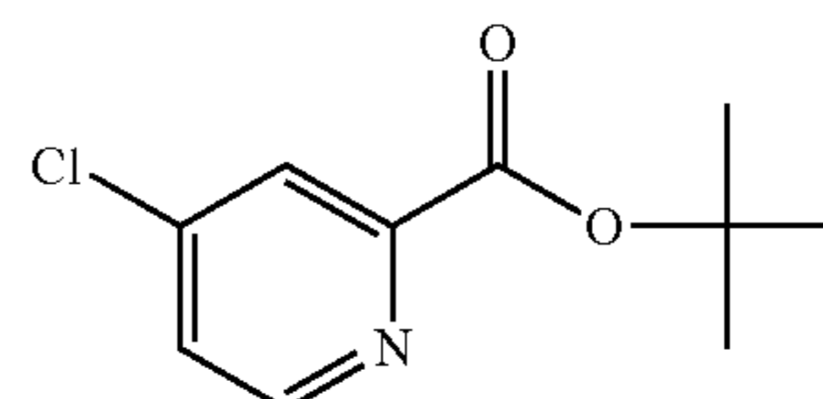
tert-Butyl 4-chloropicolinate
