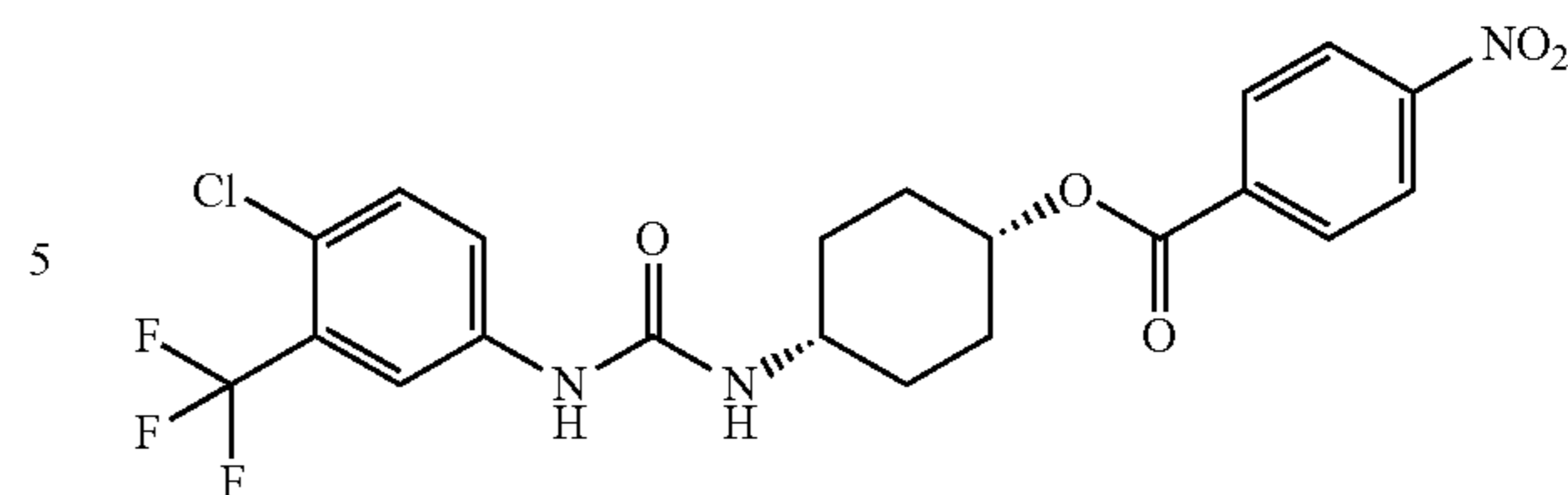
cis-4-Nitro-benzoic acid 4-[3-(4-chloro-3-trifluoromethyl-phenyl)-ureido]-cyclohexa-2,3-dienyl ester
