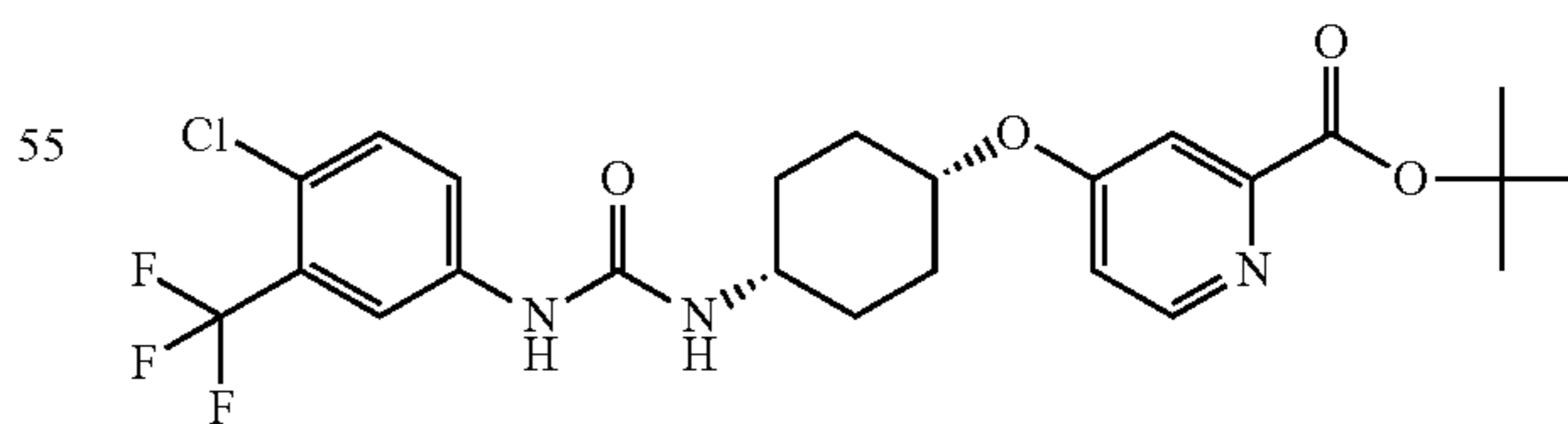
cis-4-{4-[3-(4-Chloro-3-trifluoromethyl-phenyl)-ureido]-cyclohexyloxy}-pyridine-2-carboxylic acid tert-butyl ester (2318)
