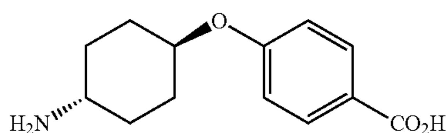
trans-4-(4-Amino-cyclohexyloxy)-benzoic acid
