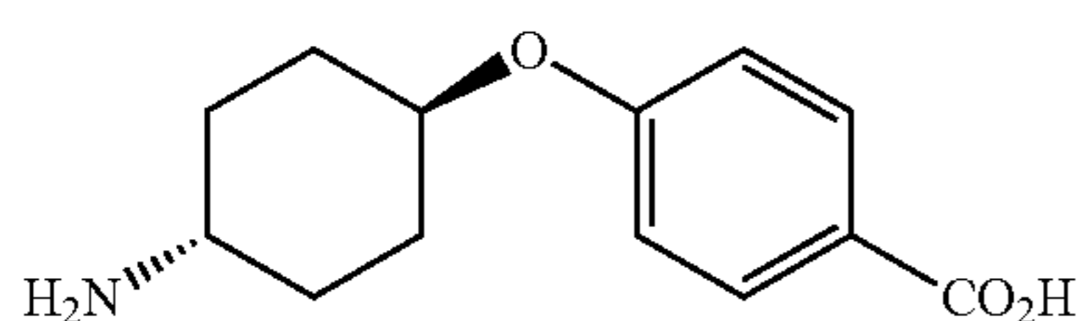
trans-4-(4-Amino-cyclohexyloxy)-benzoic acid
