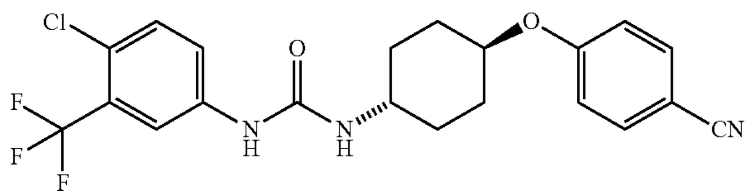
trans-1-(4-Chloro-3-trifluoromethyl-phenyl)-3-[4-(4-cyano-phenoxy)-cyclohexyl]-urea (2182)
