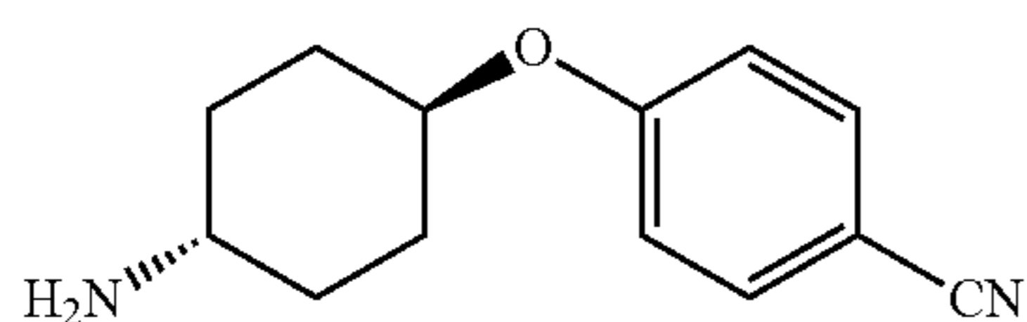
trans-4-(4-Amino-cyclohexyloxy)-benzonitrile
