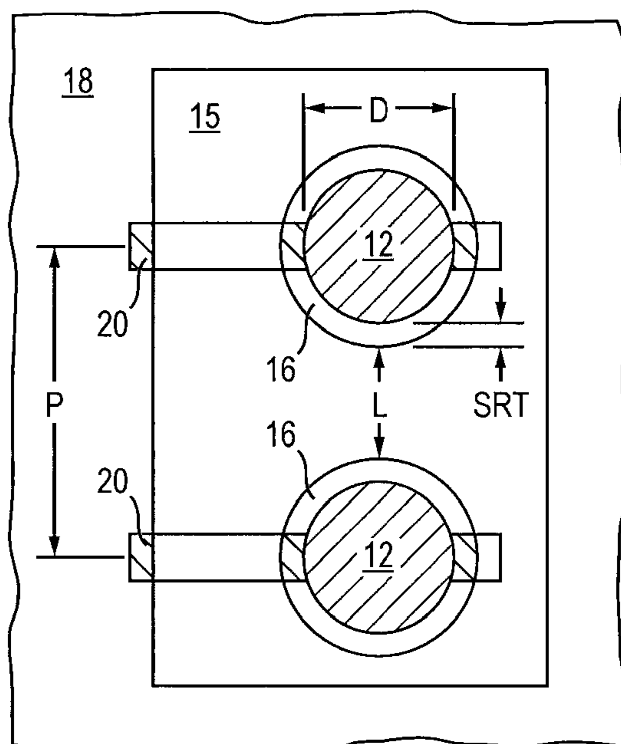
FIG. 2 (PRIOR ART)
