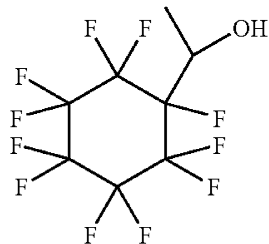
1-(1,2,2,3,3,4,4,5,5,6,6-undecafluorocyclohexyl)ethanol:
