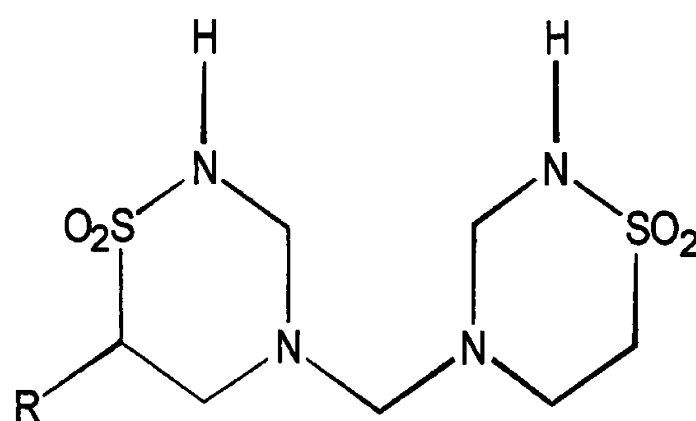
Taurolidine
