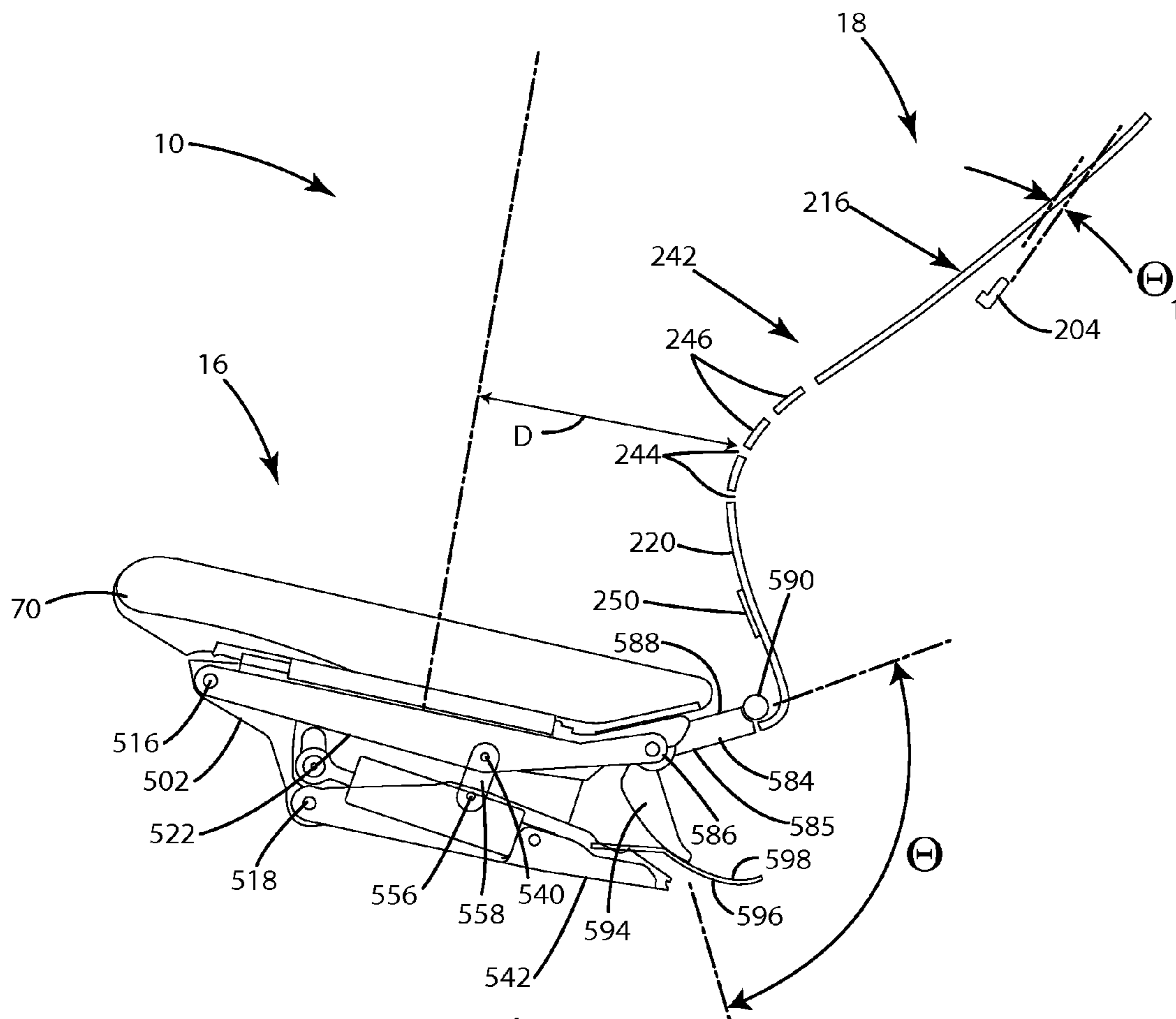
Fig.52A
