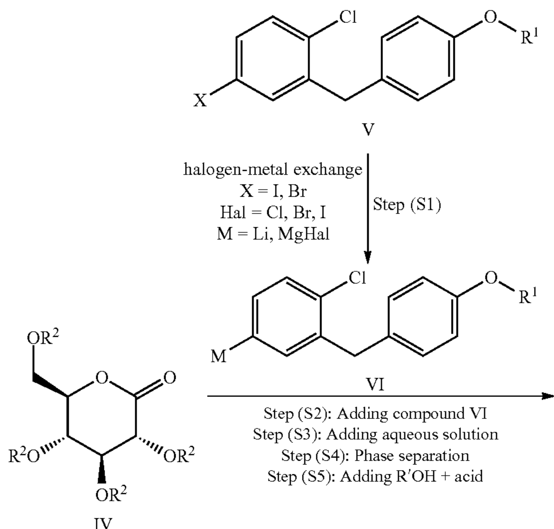
Scheme 1: Addition of an Organometallic Compound to Gluconolactone
