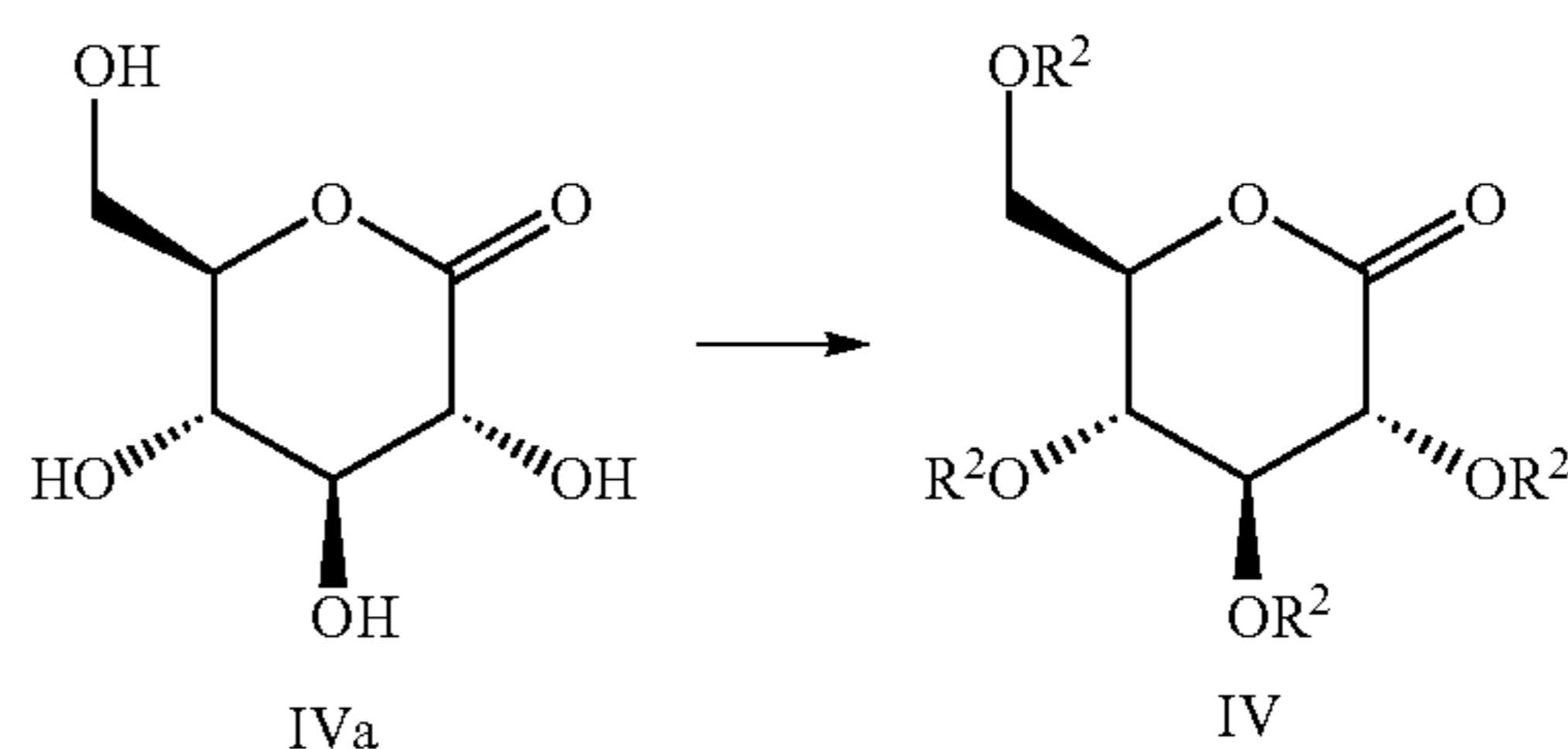
Scheme 3: Synthesis of the gluconolactone IV
