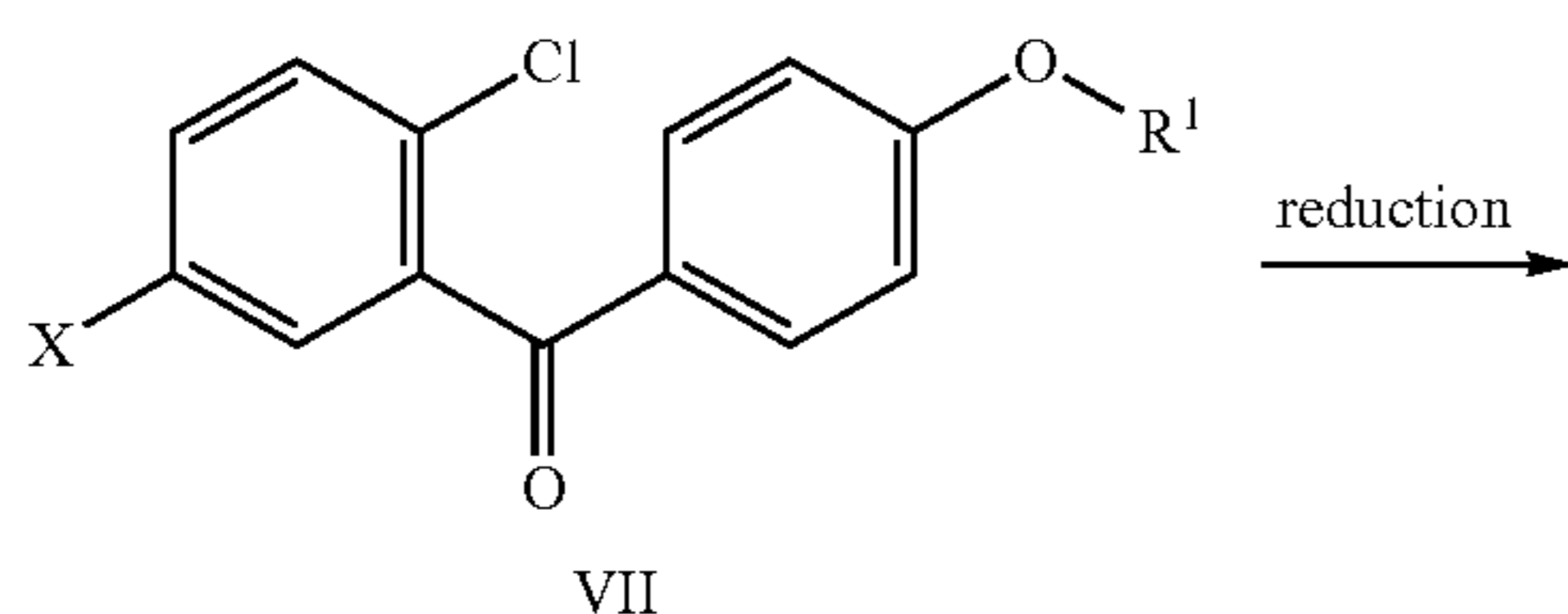
Scheme 4: Synthesis of the compound of the formula V
