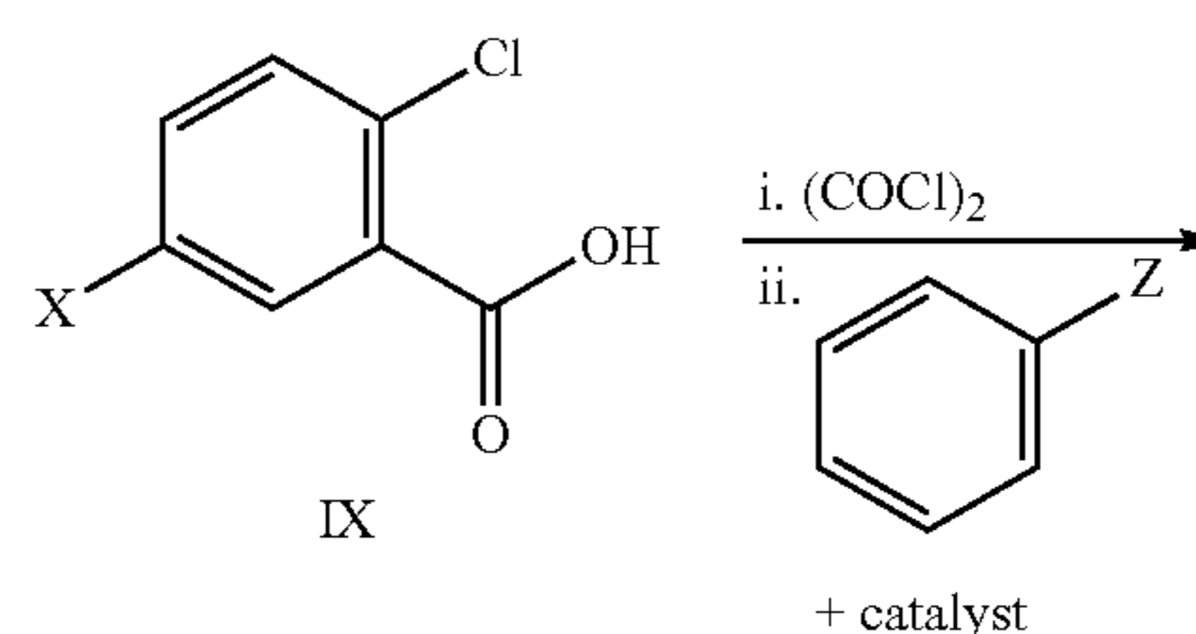
Scheme 5: Synthesis of the ketone of the formula VIII
