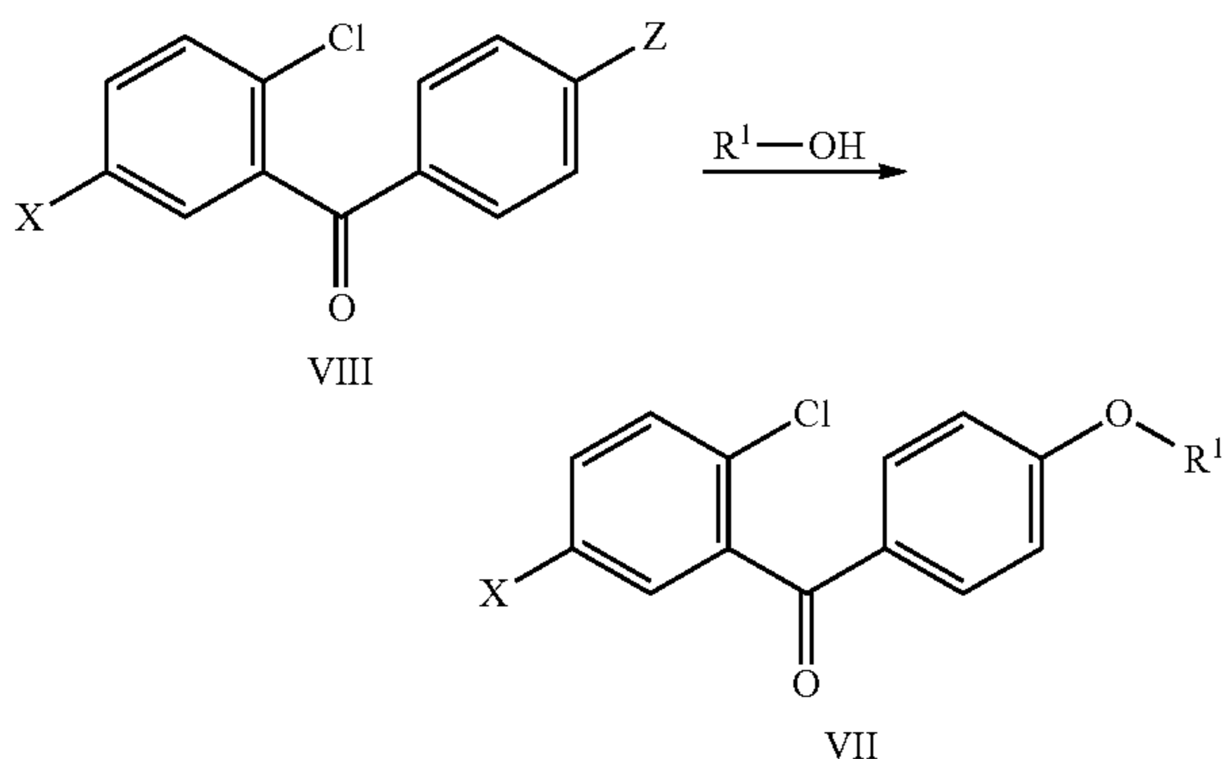
Scheme 5: Synthesis of the ketone of the formula VII
