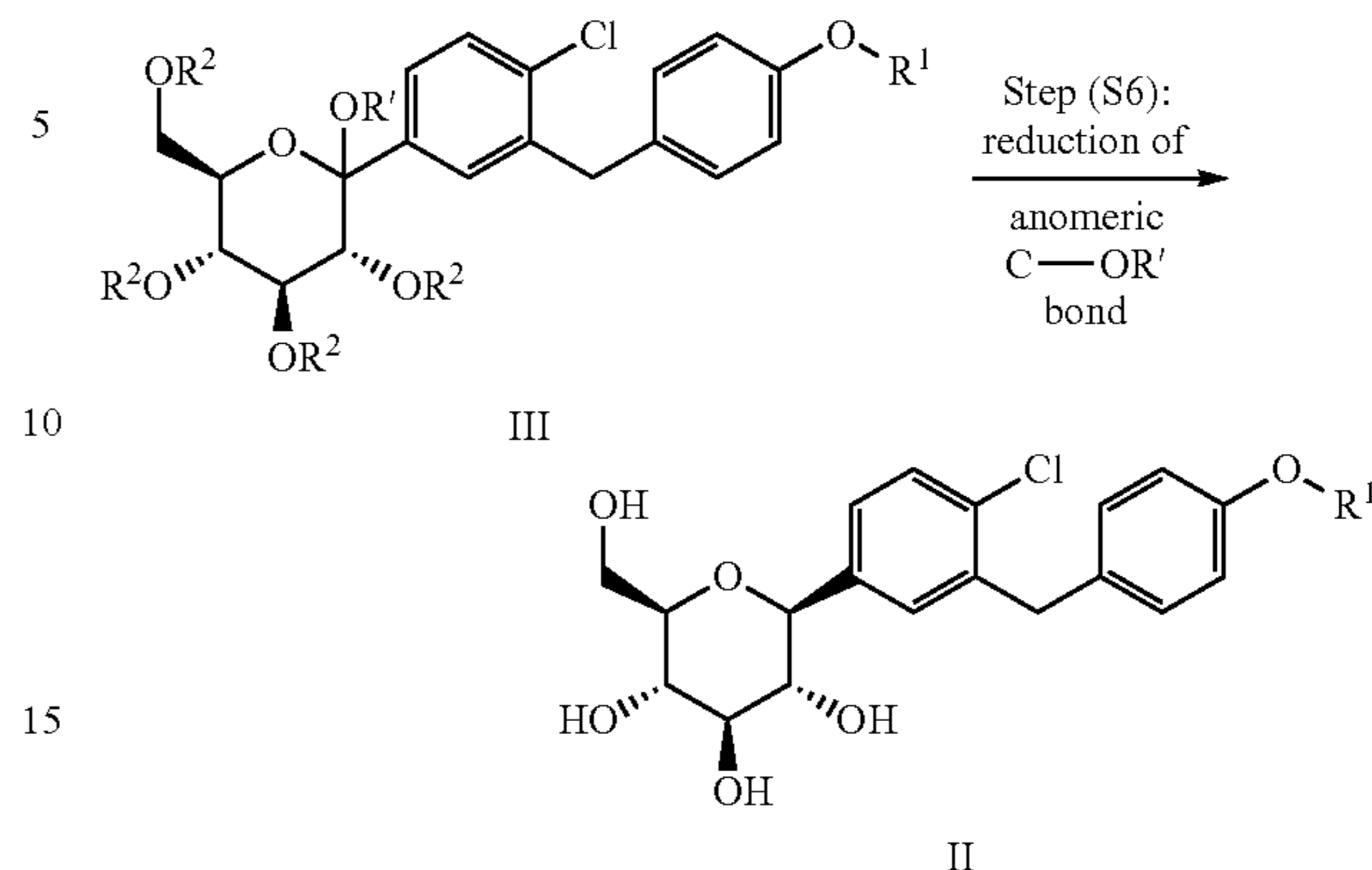
Scheme 2: Reduction of the compound III
