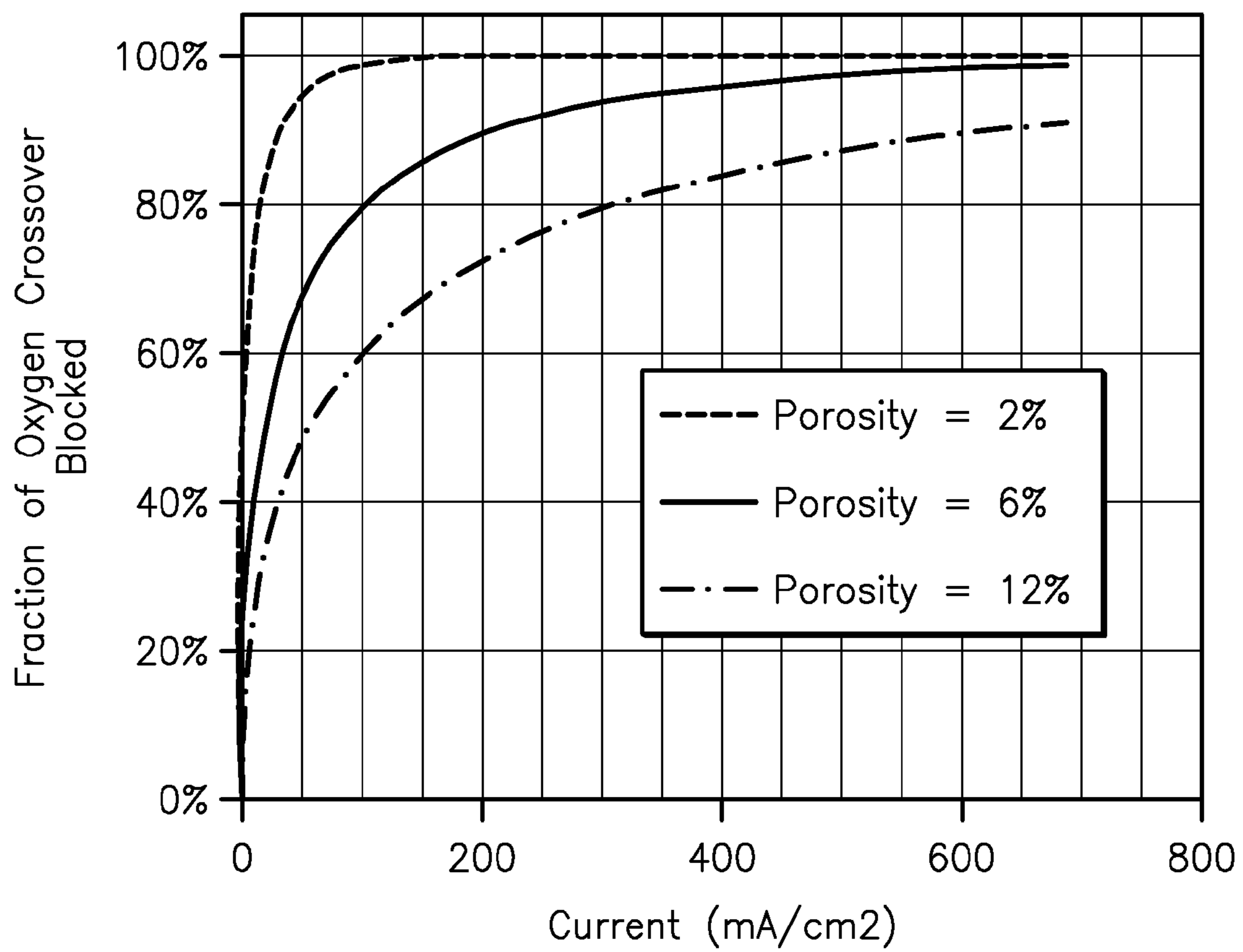
Protection Factor due to Cathode Underlayer Various Underlayer Characteristic Diffusion Currents
