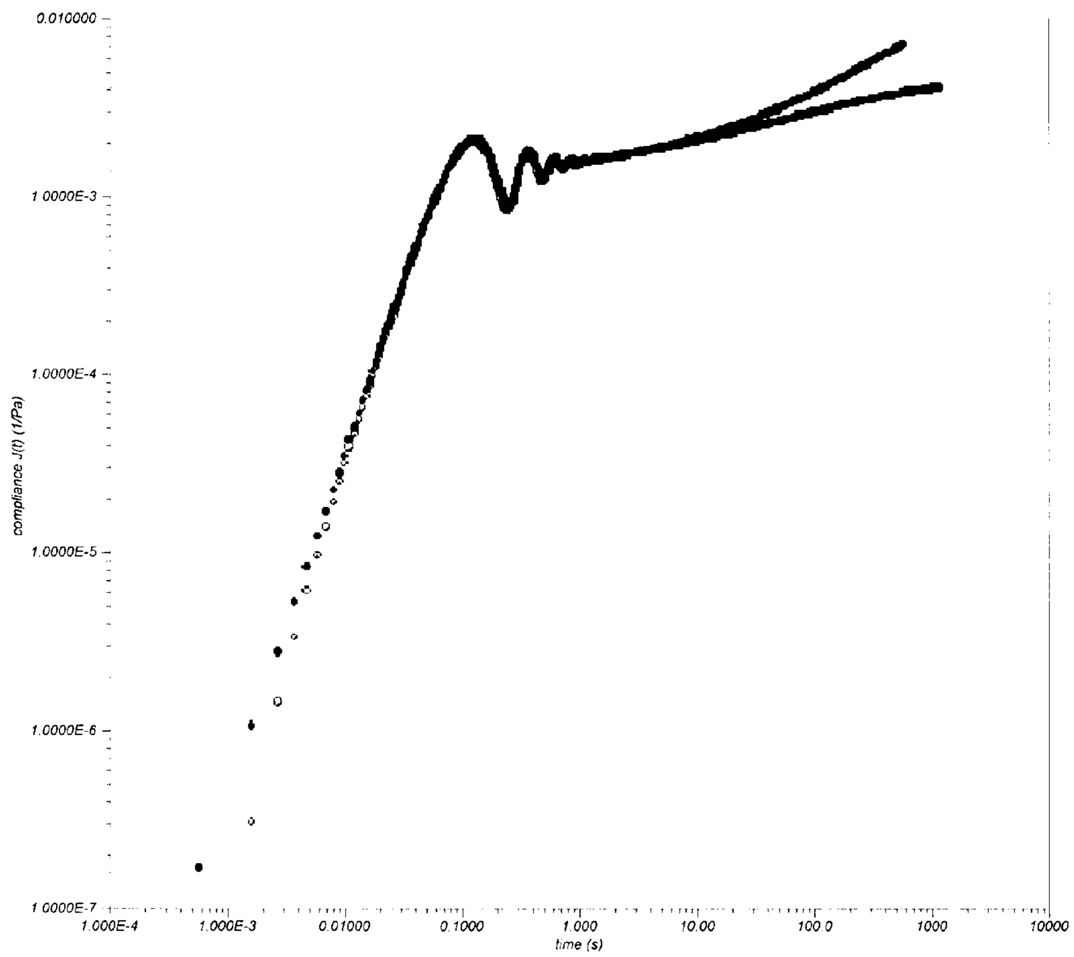
FIGURE 2: Creep and Recovery Compliances at Constant Stress = 10Pa for Example 4
