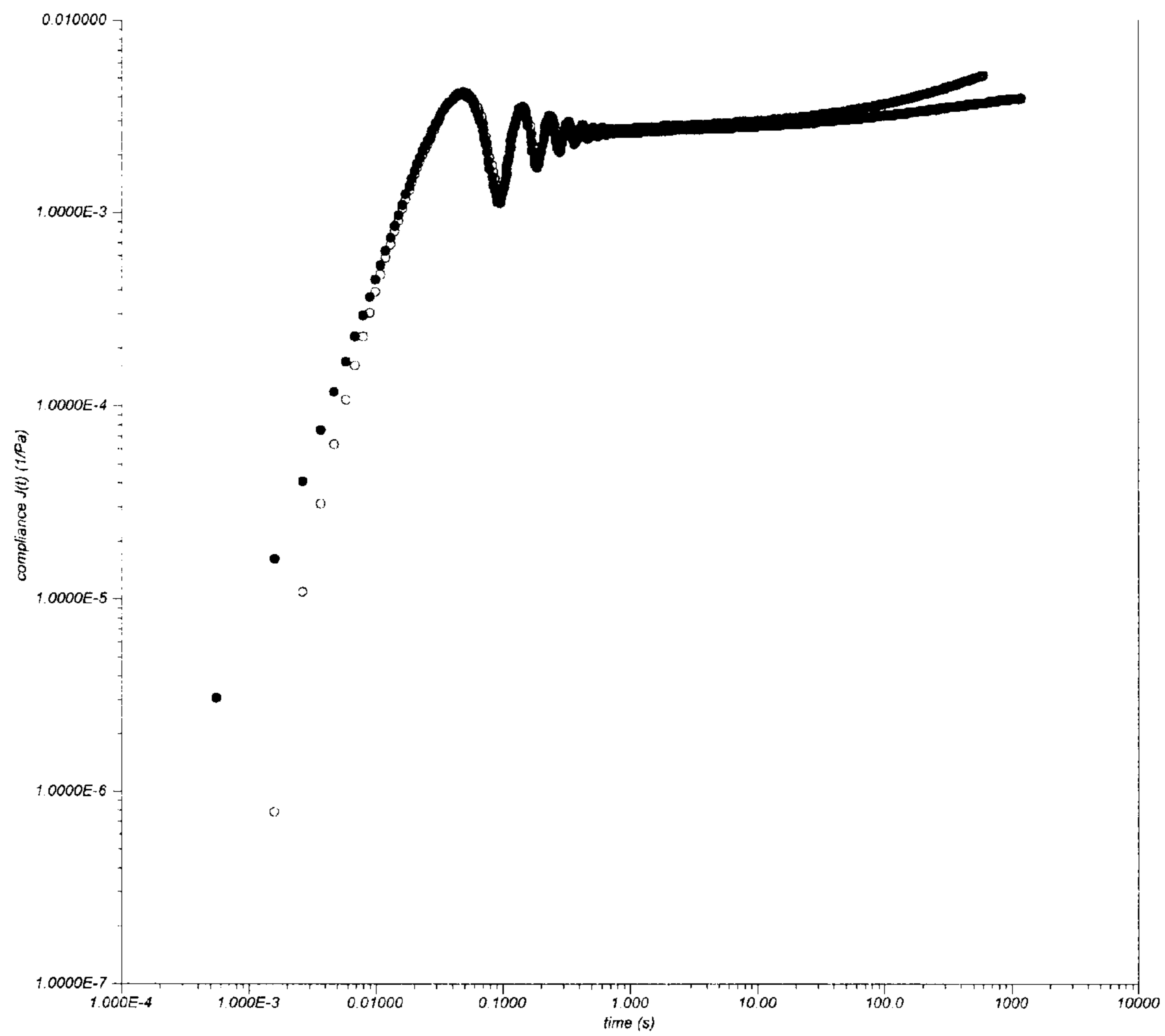
FIGURE 1: Creep and Recovery Compliances at Constant Stress = 10Pa for Example 1
