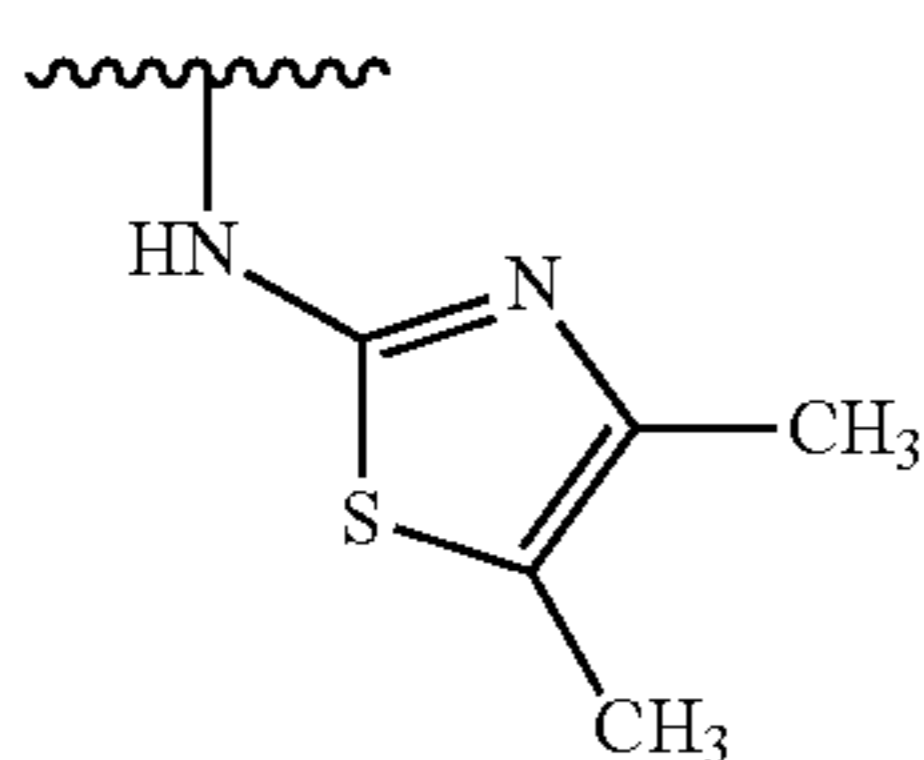
2-(4,5-DIMETHYL-1,3-THIAZOYL) GROUP
