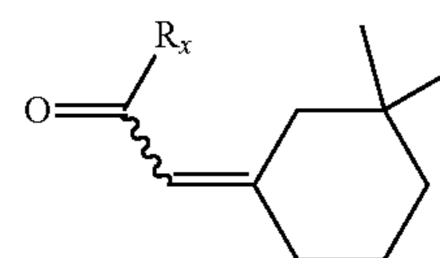
(grandlure, E/Z-(3,3-dimethyl)-cyclohexylideneacetaldehyde)
