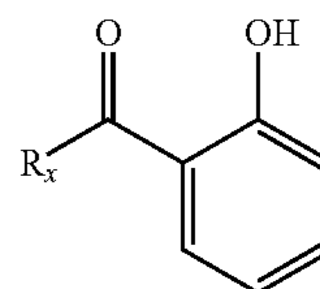
(salicylaldehyde)
