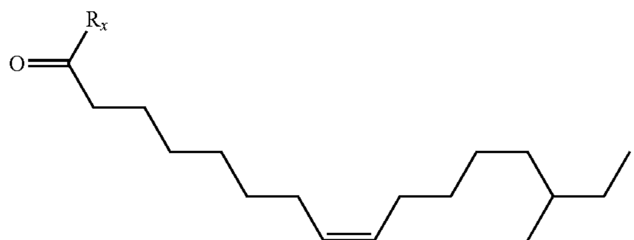
(14Me-Z8-16:Ald, Z-trogodermal)
