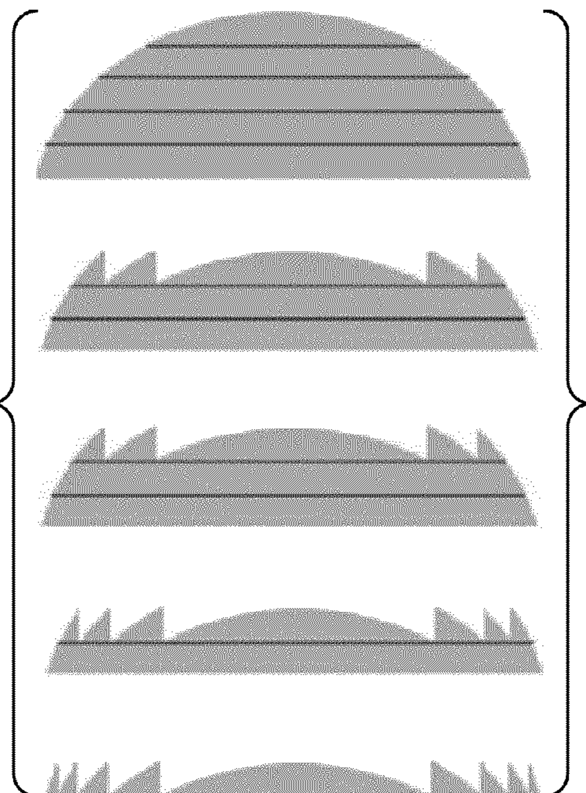
Phase Wrapping Lens Stack Example 1203
